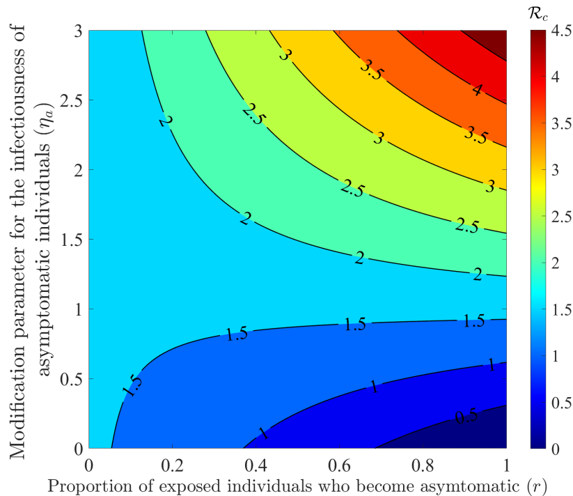
Figure C.2: Contour plot generated using the behavior-epidemiology model (2.4) depicting the impact of the proportion of exposed individuals who become asymptomatic at the end of the exposed period ( r ) and the modification parameter for the infectiousness of asymptomatic individuals ( \eta_a ) on the control reproduction number ( \mathcal{R}_C ).
