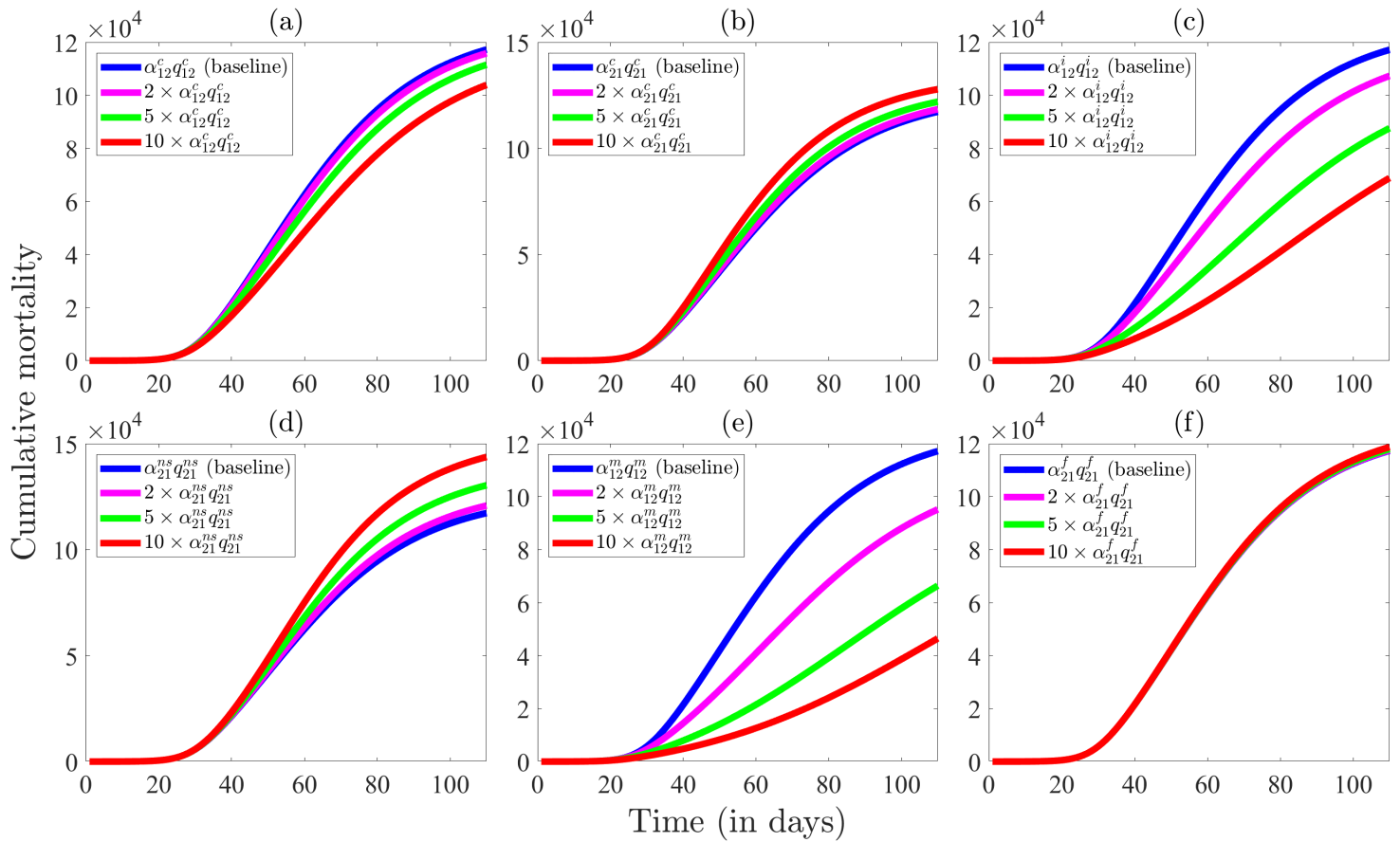
Figure 5: Simulations of the behavior-epidemiology model (2.4) assessing the impact of behavior change metrics on the cumulative mortality as a function of time. The impact on cumulative mortality is shown by increasing the product of the maximum rate of behavior change ( \alpha_{ij} ) and its associated parameter of influence ( q_{ij} ) by 2-fold, 5-fold and 10-fold and comparing the obtained cumulative mortality with that of the baseline scenario. The impact on cumulative mortality is assessed by amplifying the above-mentioned parameters related to behavior change due to (a) contact with individuals in group 2 ( \alpha_{12}^c q_{12}^c ), (b) contact with individuals in group 1 ( \alpha_{21}^c q_{21}^c ), (c) level of symptomatic transmission ( \alpha_{12}^i q_{12}^i ), (d) proportion of non-symptomatic individuals in the community ( \alpha_{21}^{ns} q_{21}^{ns} ), (e) disease-induced mortality ( \alpha_{12}^m q_{12}^m ) and (f) fatigue to intervention ( \alpha_{21}^f q_{21}^f ) by 2-fold, 5-fold and 10-fold from their baseline values. The baseline figure (i.e., cumulative mortality generated using parameter values from Tables 3 and 4) is depicted with a blue curve while magenta, green, and red curves project cumulative mortality when the respective behavior change parameters are amplified by 2-fold, 5-fold and 10-fold, respectively, with remaining parameter held at their baseline values.
