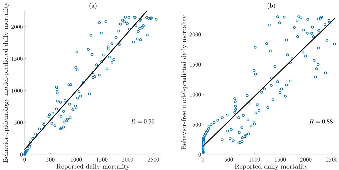
Figure B.1: Correlation between reported daily mortality and predicted daily mortality with (a) behavior-epidemiology model (2.4) and (b) behavior-free model (2.12). The data points are given by blue circles while the black line represents the best linear fit to the data. The correlation coefficient ( R ) for behavior-epidemiology and behavior-free models are 0.96 and 0.88, respectively.
