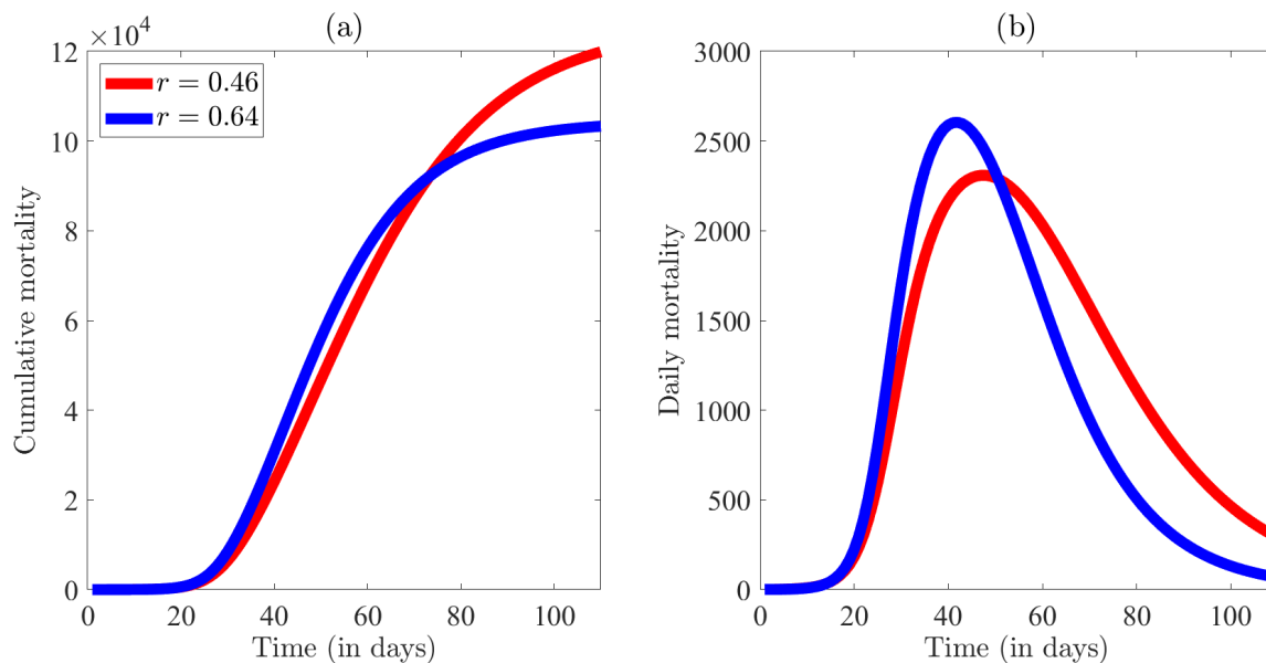
Figure C.1: Simulation of the behavior-epidemiology model (2.4) depicting the impact of two specific values of the proportion of newly infected individuals who become asymptotically-infectious at the end of the exposed period ( r ) on mortality. The (a) cumulative mortality and (b) daily mortality figures are generated for values of r = 0.46 and r = 0.64 with remaining parameters as in Tables 3 and 4.
