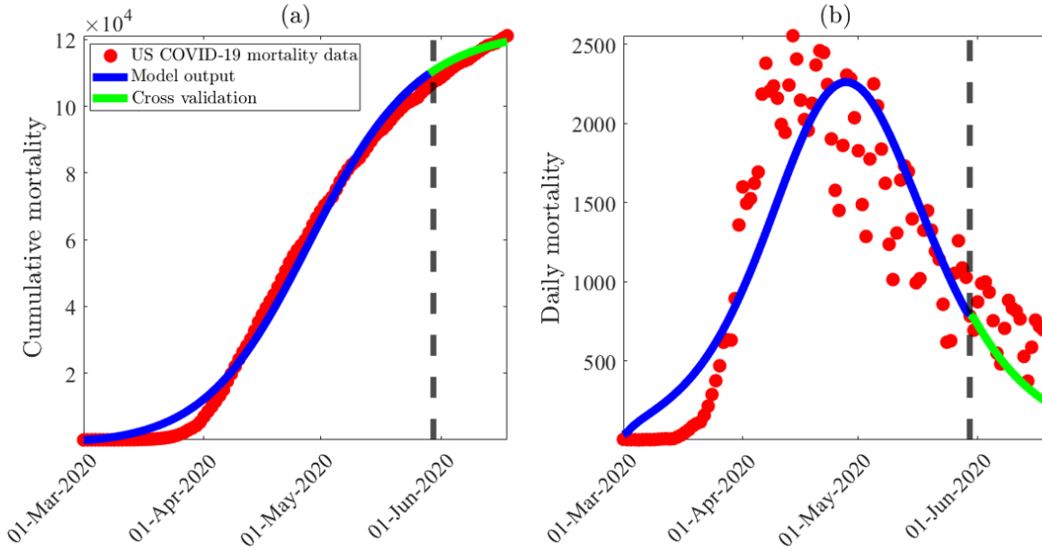
Figure 3: Data fitting, parameter estimation and cross-validation of the behavior-free model (A.1), using SARS-CoV-2 cumulative mortality data for the United States during the first wave of the pandemic (corresponding to the period from March 1st, 2020 to June 18th, 2020). (a) Least-squares fitting of the behavior-free model (A.1), showing the cumulative COVID-19 mortality generated from the model, compared to the observed cumulative mortality data for the United States during the first wave (obtained from the Johns Hopkins University COVID-19 repository [53]). (b) Simulation results of the behavior-free model (A.1), depicting the daily COVID-19 mortality for the United States, as a function of time, predicted by the behavior-free model using the fixed parameters tabulated in Table 3 and estimated parameters obtained through fitting (i.e., \beta = 0.132 per day, \eta_a = 5.349 and \delta = 1.611 \times 10^{-4} per day), in comparison to the observed daily mortality data for the United States during the first wave (obtained from the Johns Hopkins University COVID-19 repository [53]). The behavior-free model was fitted to the data from March 1st, 2020 until May 29th, 2020 (depicted by a dashed black line in the figure), and cross-validated by comparing the model output with the observed mortality data for the remaining 20 days (depicted with a green curve). Three of the initial conditions of the behavior-free model (namely E_1(0) , I_1(0) and A_1(0) ) were estimated from fitting the model with the aforementioned cumulative mortality data. The estimated values were E_1(0) = 1,388,568 , I_1(0) = 10,3571 and A_1(0) = 350,357 , respectively. The remaining initial conditions were set to (using US census data near the disease-free equilibrium): S_2(0) = 1 , E_2(0) = 0 , I_2(0) = 0 , A_2(0) = 0 , R_1(0) = 0 , R_2(0) = 0 , D(0) = 1 , N(0) = 3.314 \times 10^8 , and S_1(0) = N(0) - E_1(0) - I_1(0) - A_1(0) - R_1(0) , R_1(0) = 0 .
