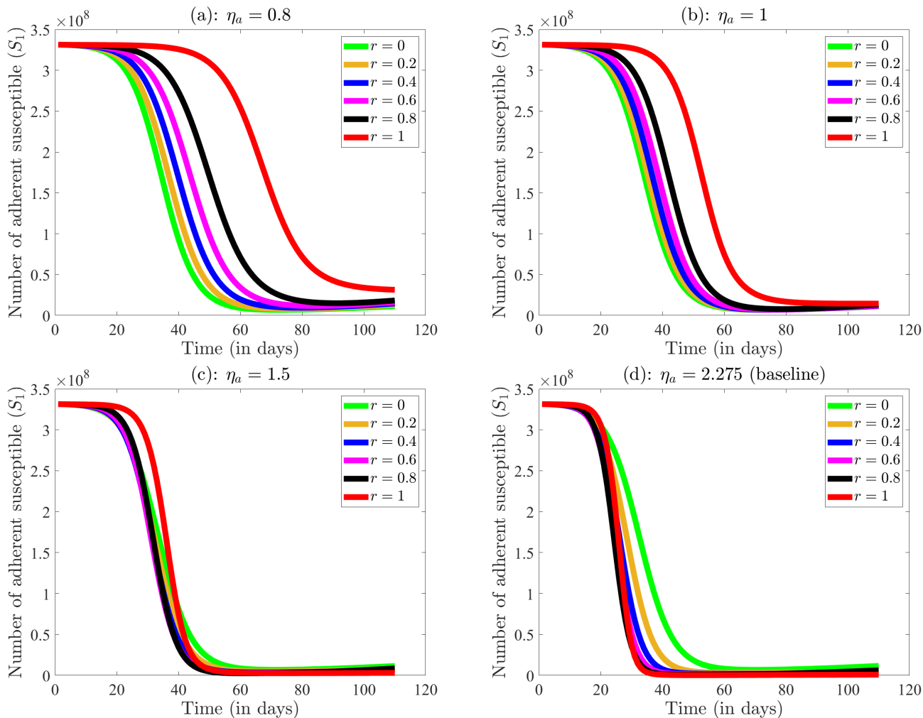
Figure 9: Simulations of the behavior-epidemiology model (2.4) assessing the impact of change in the proportion of exposed individuals who become asymptomatic at the end of the exposed period ( r ) on human behavior. The impact of r on human behavior is assessed by plotting the number of susceptible individuals in group 1 ( S_1 ) for several values of r (specifically, r = 0 , r = 0.2 , r = 0.4 , r = 0.6 , r = 0.8 and r = 1 ) for (a) \eta_a = 0.8 , (b) \eta_a = 1 , (c) \eta_a = 1.5 and (d) \eta_a = 2.275 . The figures are generated using the behavior-epidemiology model (2.4) with aforementioned values of r and \eta_a while keeping the remaining parameter values as in Tables 3 and 4.
