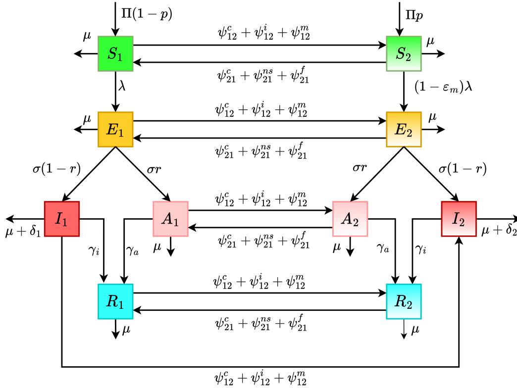
Figure 1: Flow diagram of the behavior-epidemiology model (2.4), where \lambda and p are defined in Equations (2.3) and (2.5), respectively. The state variables and parameters of the model are described in Tables 1 and 2, respectively.
