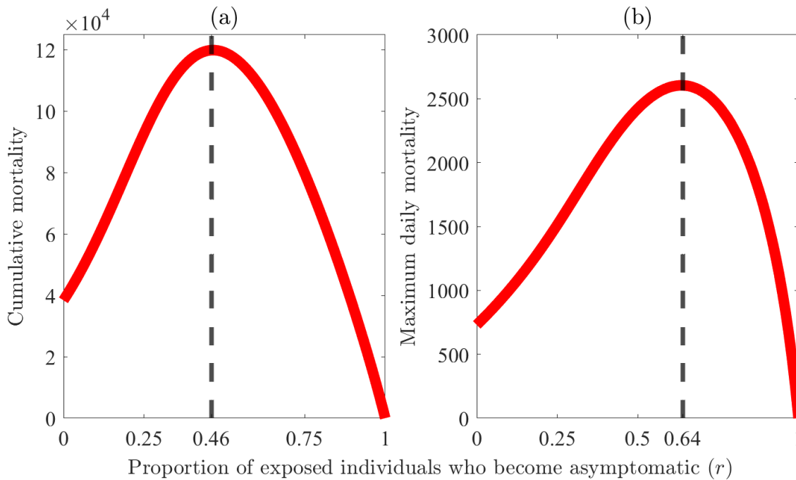
Figure 7: Simulations of the behavior-epidemiology model (2.4) assessing the impact of change in the proportion of exposed individuals who become asymptomatic at the end of the exposed period ( r ) on mortality. The change in (a) cumulative mortality and (b) maximum daily death is displayed for varying values of r . The vertical dashed line in (a) depicts the value of r that maximizes cumulative mortality while in (b) it depicts a value of r that maximizes daily mortality. The figures are generated by varying the value of r between 0 and 1 in the behavior-epidemiology model (2.4) while taking the remaining parameter values from Tables 3 and 4.
