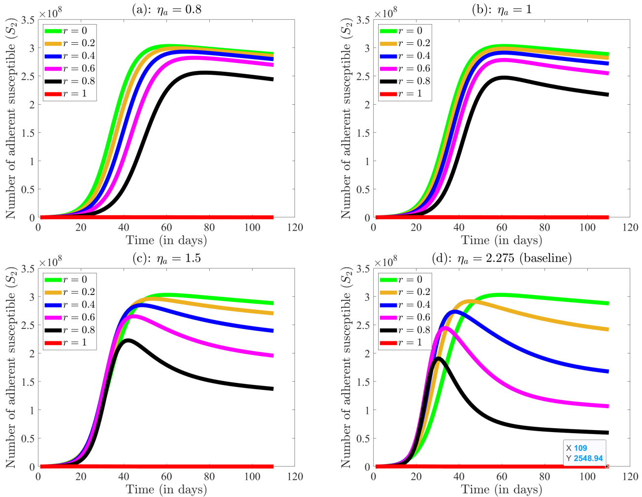
Figure 8: Simulations of the behavior-epidemiology model (2.4) assessing the impact of change in the proportion of exposed individuals who become asymptomatic at the end of the exposed period ( r ) on human behavior. The impact of r on human behavior is assessed by plotting the number of susceptible individuals in group 2 ( S_2 ) for several values of r (specifically, r = 0 , r = 0.2 , r = 0.4 , r = 0.6 , r = 0.8 and r = 1 ) for (a) \eta_a = 0.8 , (b) \eta_a = 1 , (c) \eta_a = 1.5 and \eta_a = 2.275 . Figure (d) (corresponding to \eta_a = 2.275 ) shows that the equilibrium of S_2 curve when r = 1 is minute (approximately 2,549 people) but non-zero. The figures are generated using the behavior-epidemiology model (2.4) with aforementioned values of r and \eta_a while keeping the remaining parameter values as in Tables 3 and 4.
