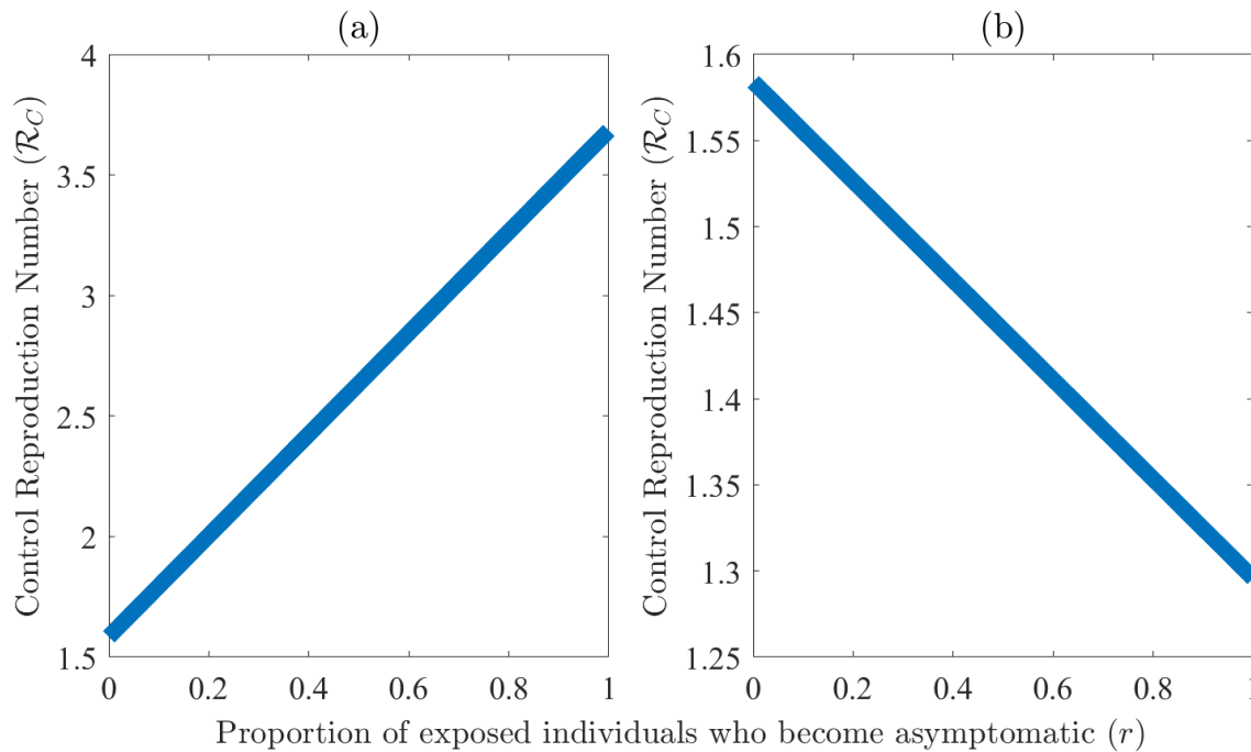
Figure 6: Simulations of the behavior-epidemiology model (2.4) assessing the impact of change of the proportion of exposed individuals who become asymptomatic at the end of the exposed period ( r ) on the control reproduction number ( \mathcal{R}_C ). An increase in r can increase or (b) decrease \mathcal{R}_C . Figure (a) is generated by calculating \mathcal{R}_C , given by Equation (2.25), for varying values of r between 0 and 1, with remaining parameter values as in Tables 3 and 4. Figure (b) is similarly generated by varying r between 0 and 1, \eta_a = 0.8 and remaining parameter values as in Tables 3 and 4.
