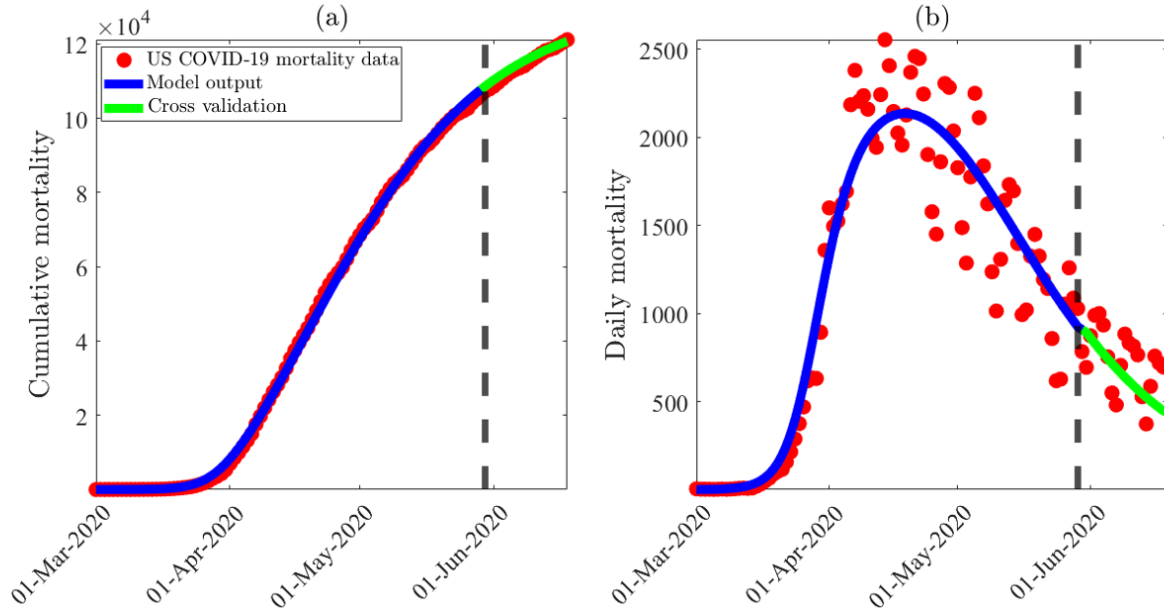
Figure 2: Data fitting, parameter estimation and cross-validation of the behavior-epidemiology model (2.4), using SARS-CoV-2 cumulative mortality data for the United States during the first wave of the pandemic (corresponding to the period from March 1st, 2020 to June 18th, 2020). (a) Least-squares fitting of the behavior-epidemiology model (2.4), showing the cumulative COVID-19 mortality generated from the model, compared to the observed cumulative mortality data for the United States during the first wave (obtained from the Johns Hopkins University COVID-19 repository [53]). (b) Simulation results of the behavior-epidemiology model (2.4), depicting the daily COVID-19 mortality for the United States, as a function of time, predicted by the behavior-epidemiology model using the fixed and estimated parameters tabulated in Tables 3 and 4, respectively, in comparison to the observed daily mortality data for the United States during the first wave (obtained from the Johns Hopkins University COVID-19 repository [53]). The behavior-epidemiology model was fitted to the data from March 1st, 2020 until May 29th, 2020 (depicted by a dashed black line in the figure), and cross-validated by comparing the model output with the observed mortality data for the remaining 20 days (depicted with a green curve). Three of the initial conditions of the behavior-epidemiology model (namely E_1(0) , I_1(0) and A_1(0) ) were estimated from fitting the model with the aforementioned cumulative mortality data. The estimated values were E_1(0) = 5,754 , I_1(0) = 2,338 and A_1(0) = 2,501 , respectively. The remaining initial conditions were set to (using US census data near the disease-free equilibrium): N(0) = 3.314 \times 10^8 , S_2(0) = 1 , E_2(0) = 0 , I_2(0) = 0 , A_2(0) = 0 , R_1(0) = 0 , R_2(0) = 0 , D(0) = 1 , and S_1(0) = N(0) - E_1(0) - I_1(0) - A_1(0) - S_2(0) .
