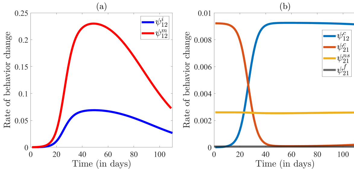
Figure 4: Simulations of the behavior-epidemiology model (2.4) assessing the impact of disease-related metric on behavior change during the first wave of COVID-19 in the United States. The rate of behavior change (a) due to infection ( \psi_{12}^i ) and mortality ( \psi_{12}^m ) and (b) due to contact with individuals in group 2 ( \psi_{12}^c ), contact with individuals in group 1 ( \psi_{21}^c ), presence of non-symptomatic individuals in the community ( \psi_{21}^{ns} ) and fatigue ( \psi_{21}^f ) plotted as a function of time. The figure is generated using baseline parameter values from Tables 3 and 4.
