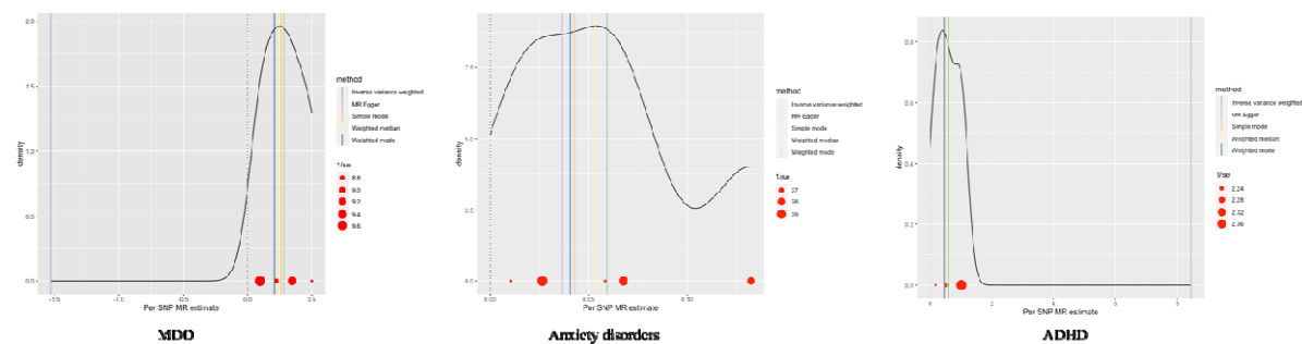
Figure 3: Mendelian Randomization Analysis: Causal Effects of MDD, ADHD, and Anxiety Disorders on IBS.
