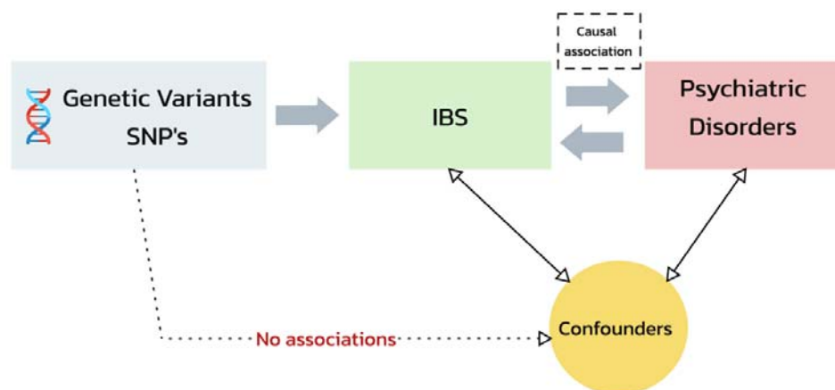
Figure 1: Flowchart of Mendelian Randomization Analysis: IBS and Psychiatric Disorder Associations.
