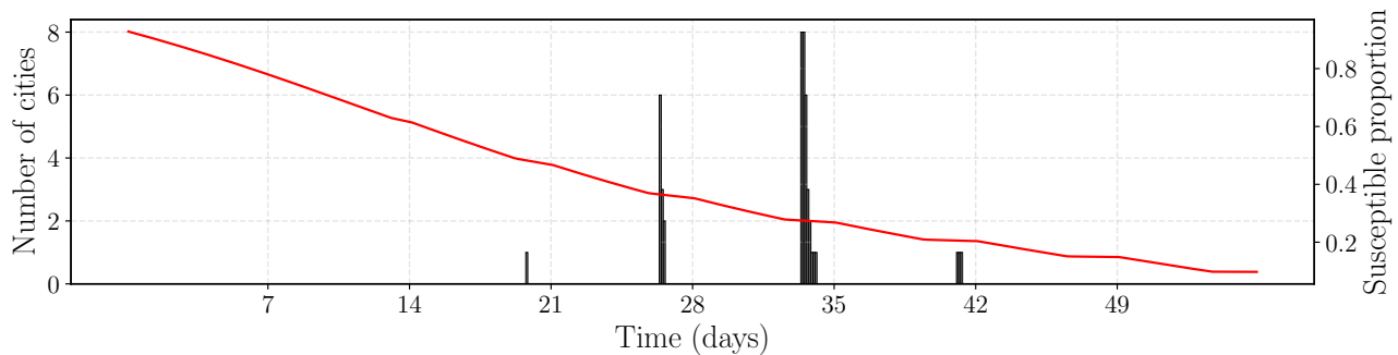
Figure 19: Analysis of Effective Vaccination Rates in the Rio de Janeiro Metropolitan Area.
