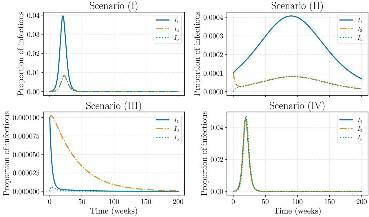
Figure 9: Infectious curves for different scenarios of \beta .
