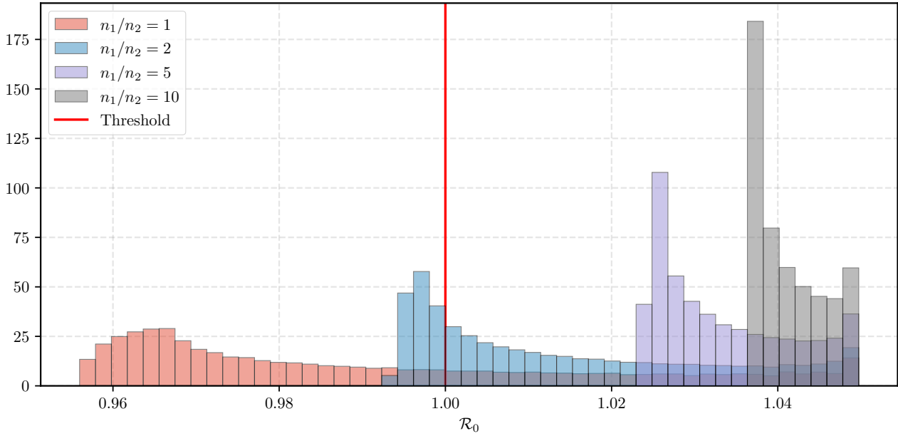
Figure C.21: Histogram of the possible values of \mathcal{R}_0 as function of \alpha and p_{21} for two cities: histogram of the values of \mathcal{R}_0 generated by randomly selecting \alpha \in (0, 1) and p_{21} \in (0, 0.9) . We consider four scenarios for the ratio n_1/n_2 , (1, 2, 5, 10). The other parameters are \beta_1 = 0.15 , \gamma = 1/7 and \mu = 3.6 \cdot 10^{-5} , the same as in Figure 6.
