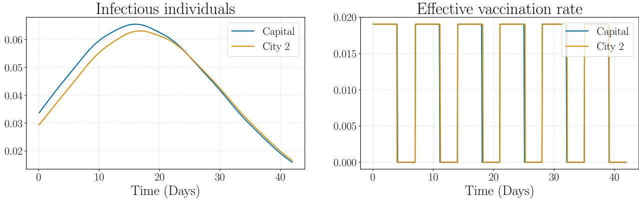
Figure 13: Optimal trajectories and control for two-city interaction for uniform infection rates. Optimal trajectory of the proportion of susceptible and infectious individuals in two cities and the optimal control using the same settings as Figure 11 except \beta = (0.25, 0.25) .
