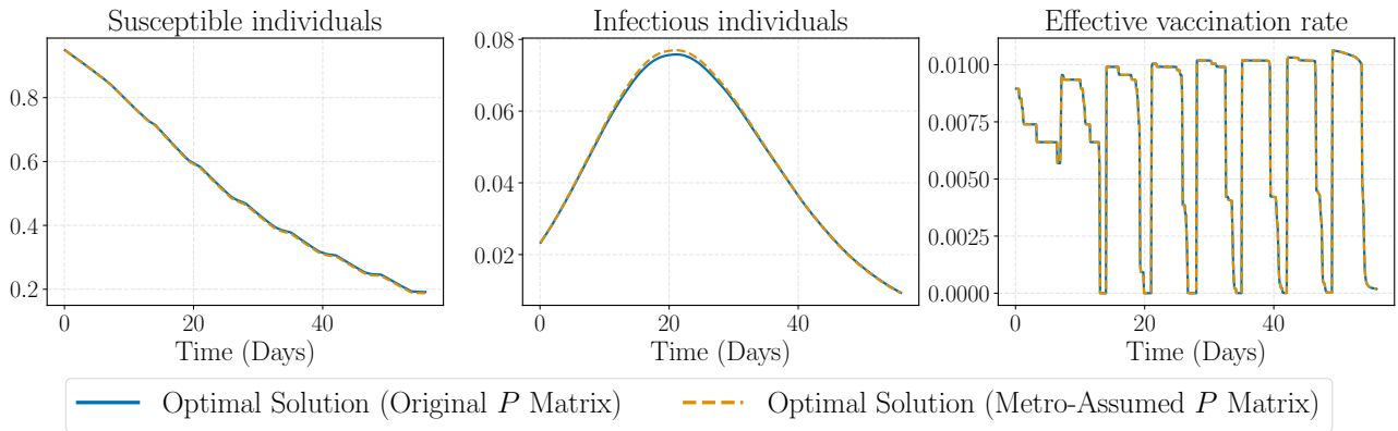
Figure 18: Comparative Analysis of Optimal Vaccination Strategies in the Rio de Janeiro Metropolitan Area.
