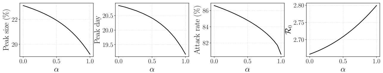
Figure C.23: Impact of \alpha on the epidemic: We analyze four different epidemiological quantities considering the aggregated population, the peak size (the highest value in the infectious curve), the peak day (the day when the peak size occurs), the attack rate (the number of individuals who contract the disease after T = 200 days), and \mathcal{R}_0 , as functions of \alpha . The parameters used are based on the setting in Table C.2, except for matrix P , where we assume that 20% of each city's population goes to the capital while the remaining population stays in their home city.
