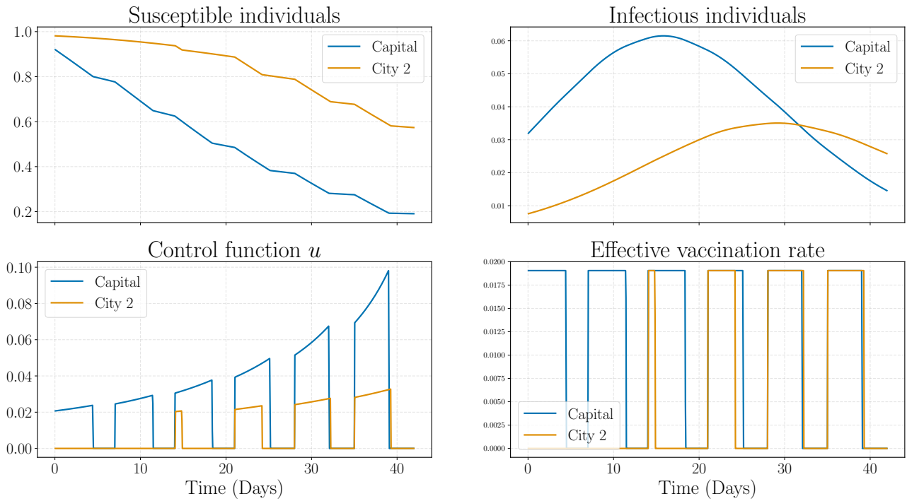
Figure 11: Optimal trajectories and control for two-city interaction.
