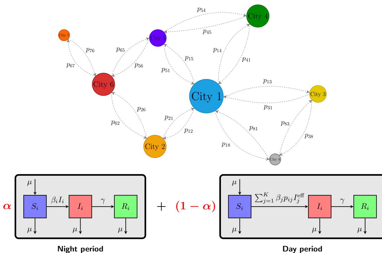
Figure 1: Graphical representation of city interactions and the SIR model.
