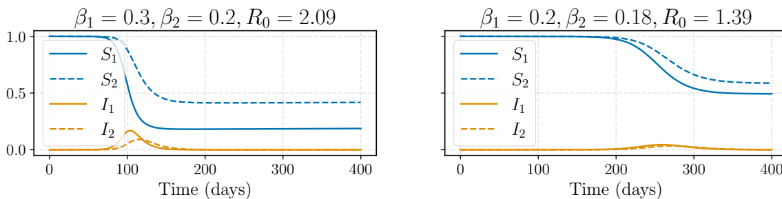
Figure 5: Dynamics of the Epidemic in Two Cities.
