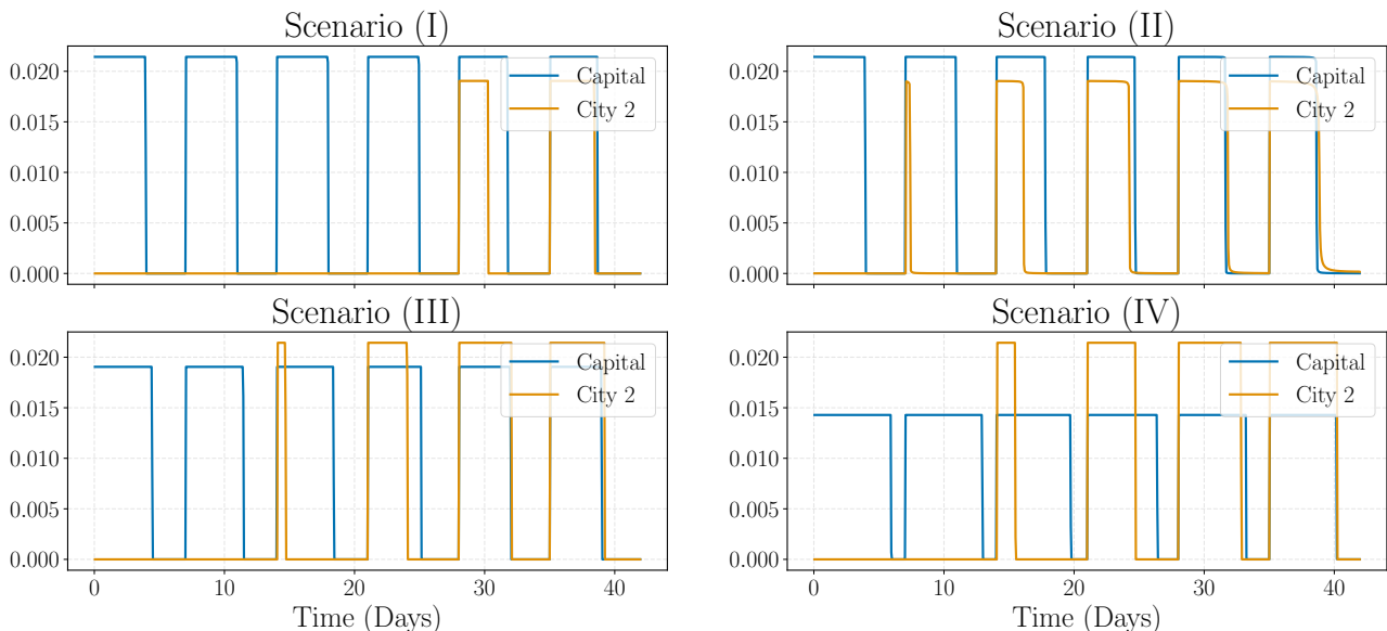
Figure 14: Optimal effective vaccination rate for two-city interaction.
