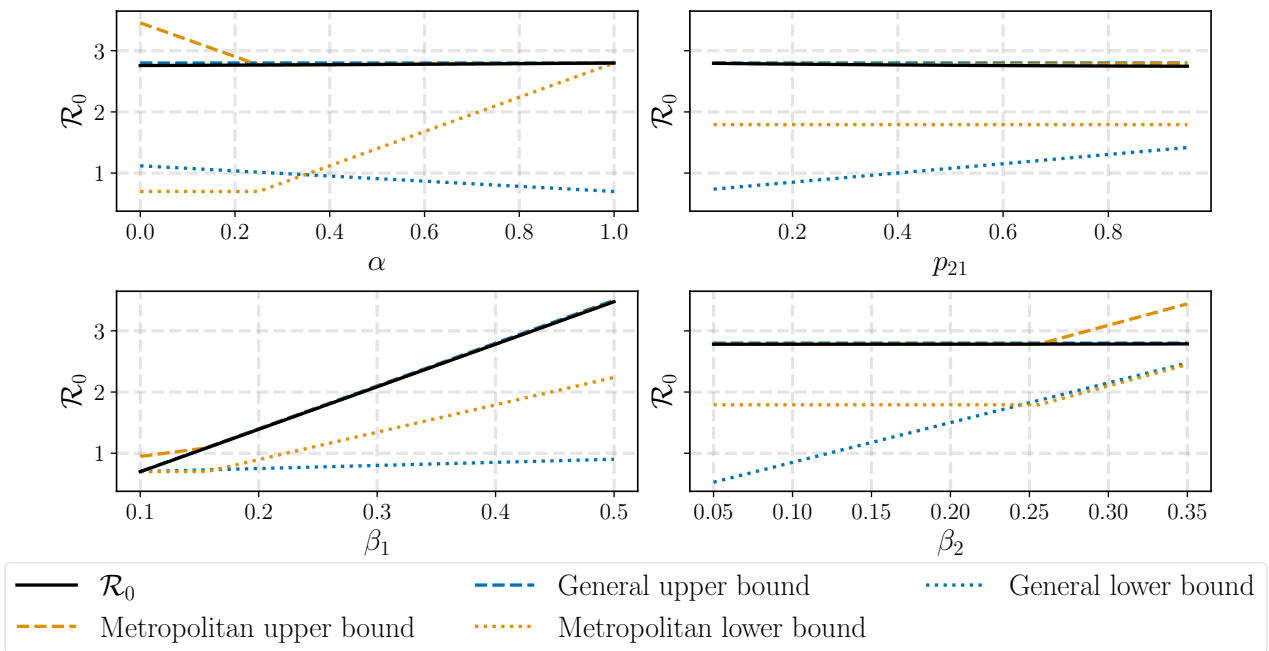
Figure 7: Impact of the parameters on the bounds of \mathcal{R}_0 .
