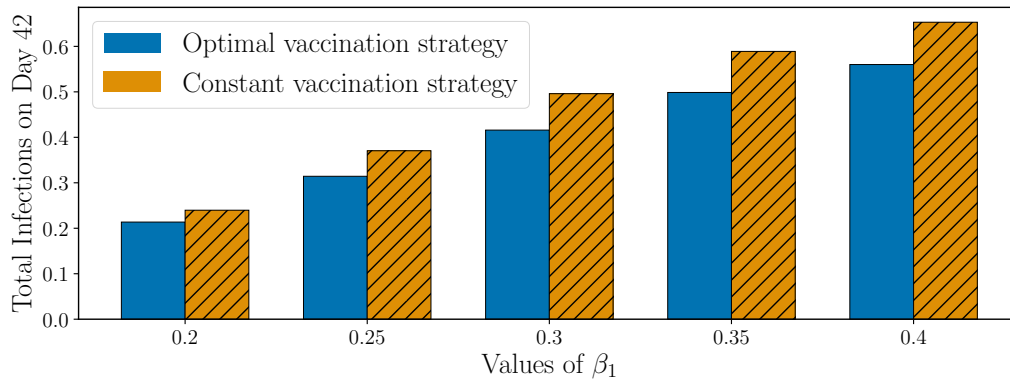
Figure 16: Comparison between optimal and constant vaccination strategies for different values of \beta_1 .
