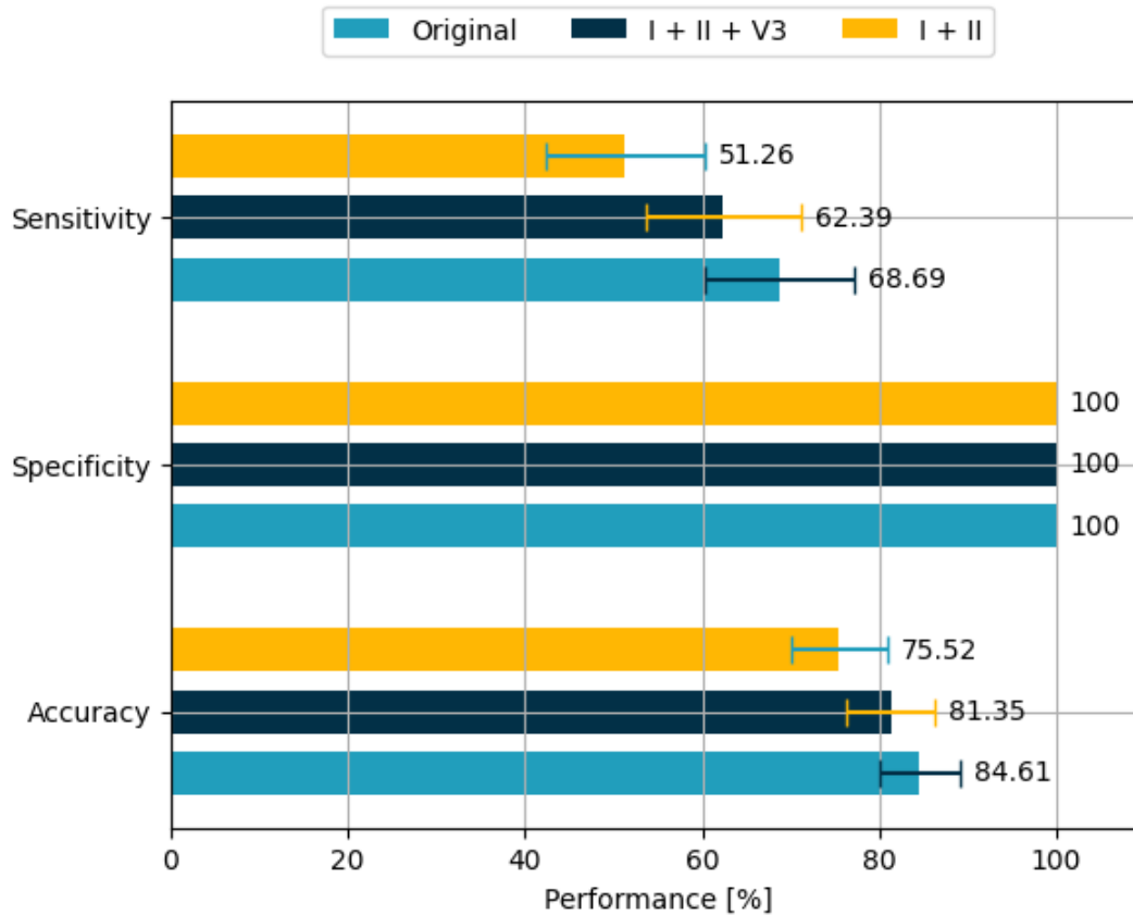
Figure 3. Detection accuracy of the original and reconstructed ECGs in clinical validation. Sensitivity, specificity and accuracy obtained during the clinical validation of the proposed reconstruction model. The sensitivity, also known as true positive ratio, corresponds to the probability that an ECG is diagnosed as STEMI, conditioned on the fact the original signal presents STEMI evidence. The specificity, also known as true negative ratio, corresponds to the probability that an ECG is diagnosed as not-STEMI, conditioned on the fact that the original signal does not present STEMI evidence. Finally, the accuracy is given by the ratio between the number of correct diagnoses and the total number of ECGs analyzed.
