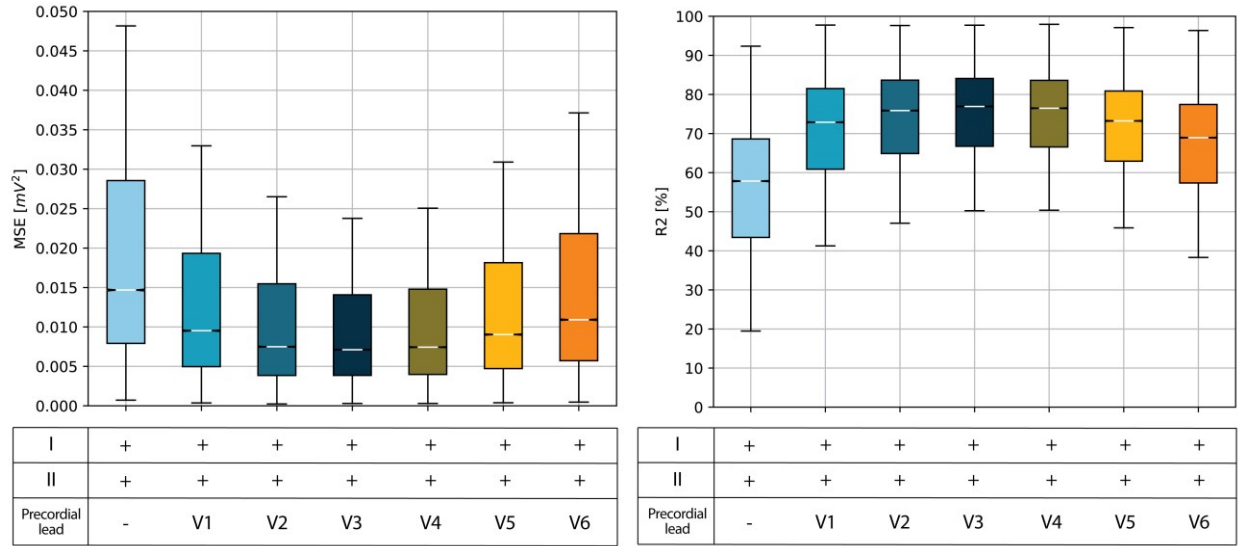
Figure 1. Distributions of mean square error and coefficient of determination in 12-lead ECG reconstruction.
