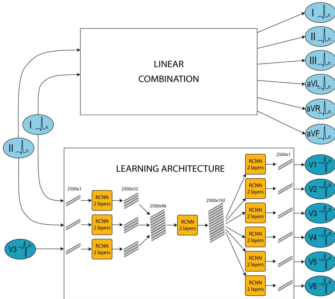
Figure 4. 12-lead ECG reconstruction algorithm architecture.
