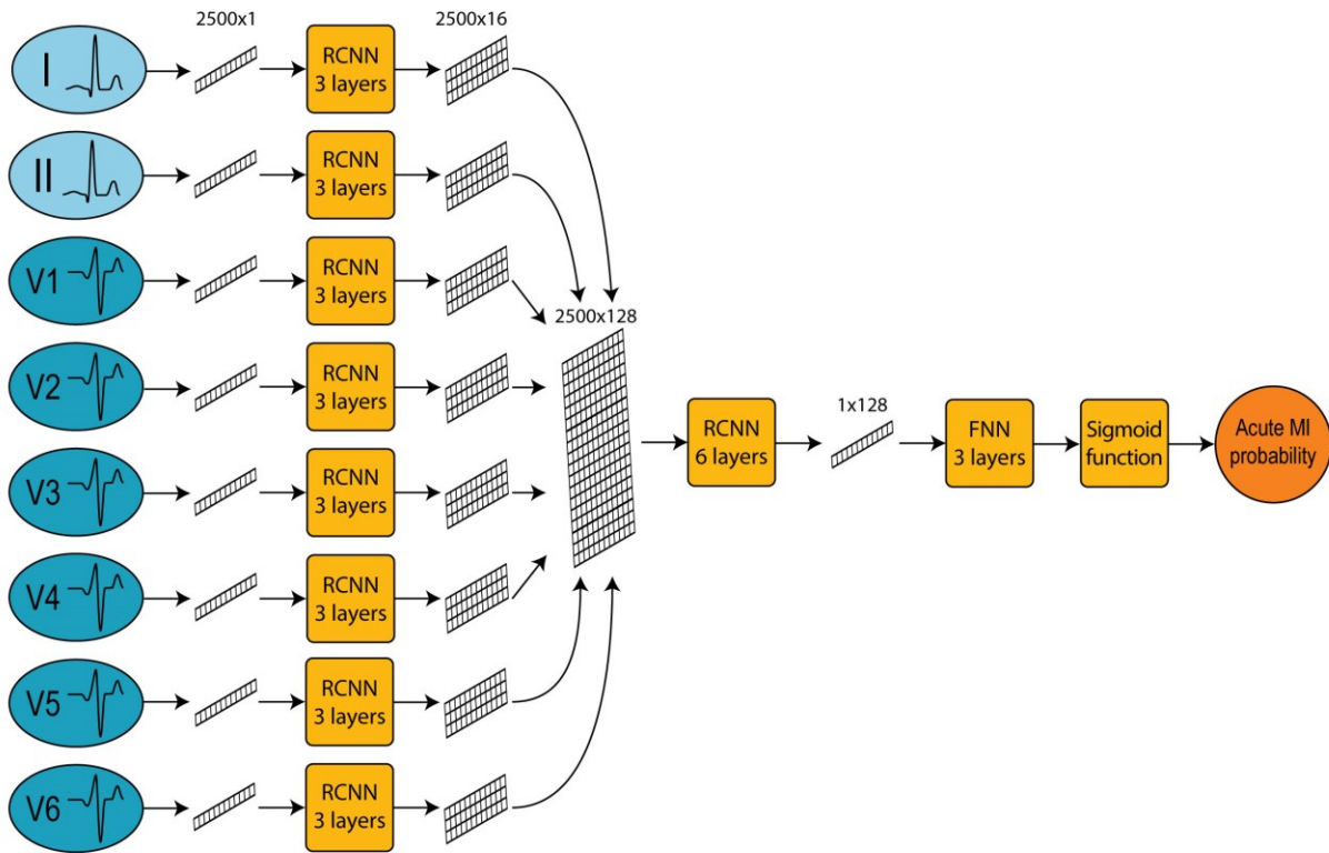
Figure 5. Acute MI detection algorithm architecture.
