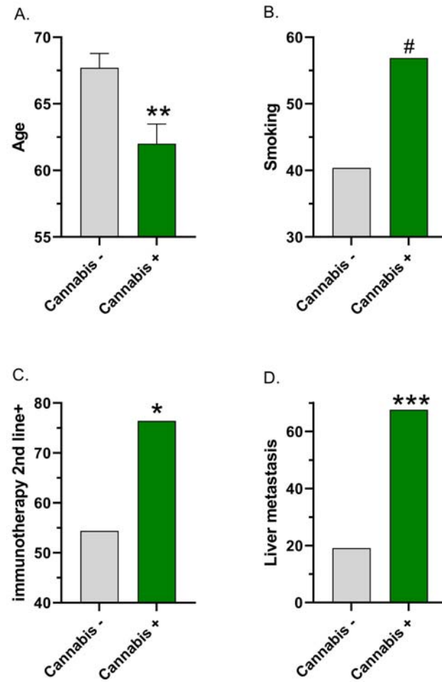
Figure 1. Baseline group differences between cannabis non-users (-) and users (+) based on re-analysis of the reported data in [8] (A, B) and [9] (C, D) #chi-square p \leq .061 , *chi-square p < .05 , **t-test p < .005 , ***chi-square p < .0001 .
