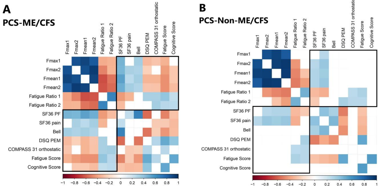
Figure 2. Correlation matrix showing correlation coefficients of parameters of symptom severity and handgrip strength (HGS) for both patient groups. Rectangles indicate the parameters of HGS. Non-significant coefficients were left blank. (A) Patients diagnosed with both PCS and ME/CFS; (B) patients diagnosed with PCS but not ME/CFS.
