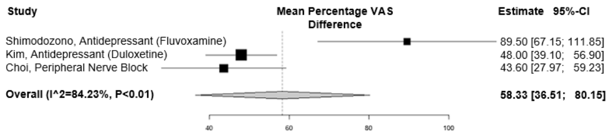
Figure 7: Proportional Meta-analysis results and forest plot from Pharmacological studies
