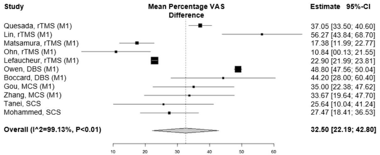
Figure 5: Proportional Meta-analysis results and forest plot from Neuromodulation studies.
