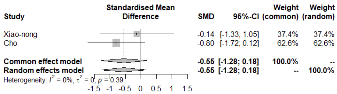
Figure 8: Random-Effects Meta-analysis results and forest plot from Acupuncture studies
