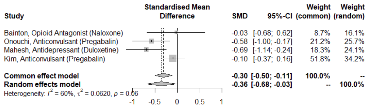
Figure 6: Random-Effects Meta-analysis results and forest plot from Pharmacological studies
