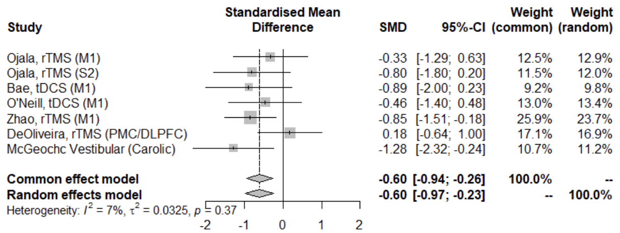
Figure 4: Meta-analysis results and forest plot from Neuromodulation studies.
