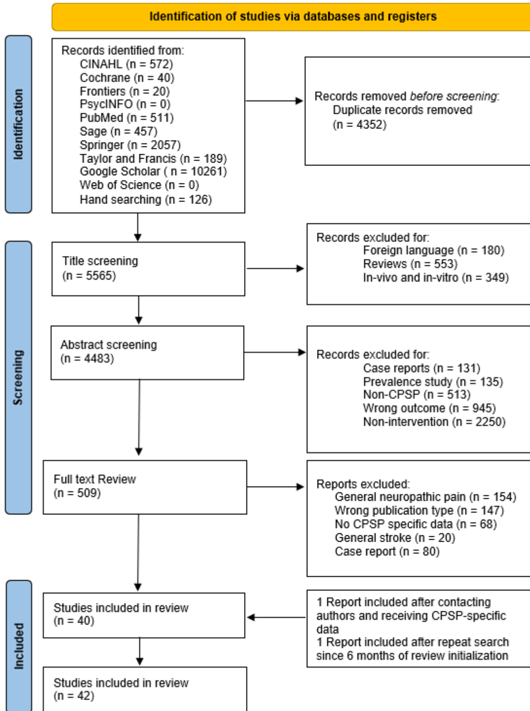
Figure 1: PRISMA flowchart of literature review
