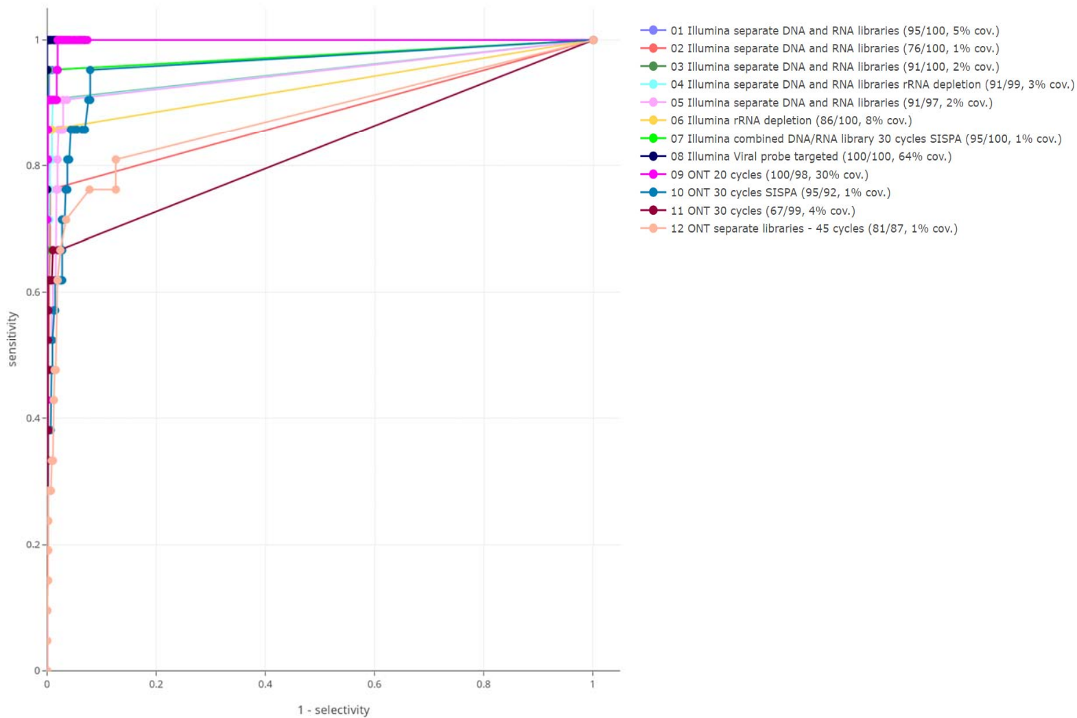
Figure 3. Receiver operating characteristic (ROC) curves based on varying threshold of percentage genome covered for defining a positive result for the twelve metagenomic protocols. Viruses up to PCR CT-values of 35 were included in the analyses. Legend: protocol name, sensitivity/specificity (%), and optimal threshold for horizontal genome coverage (% cov.) at the optimal ROC point.
