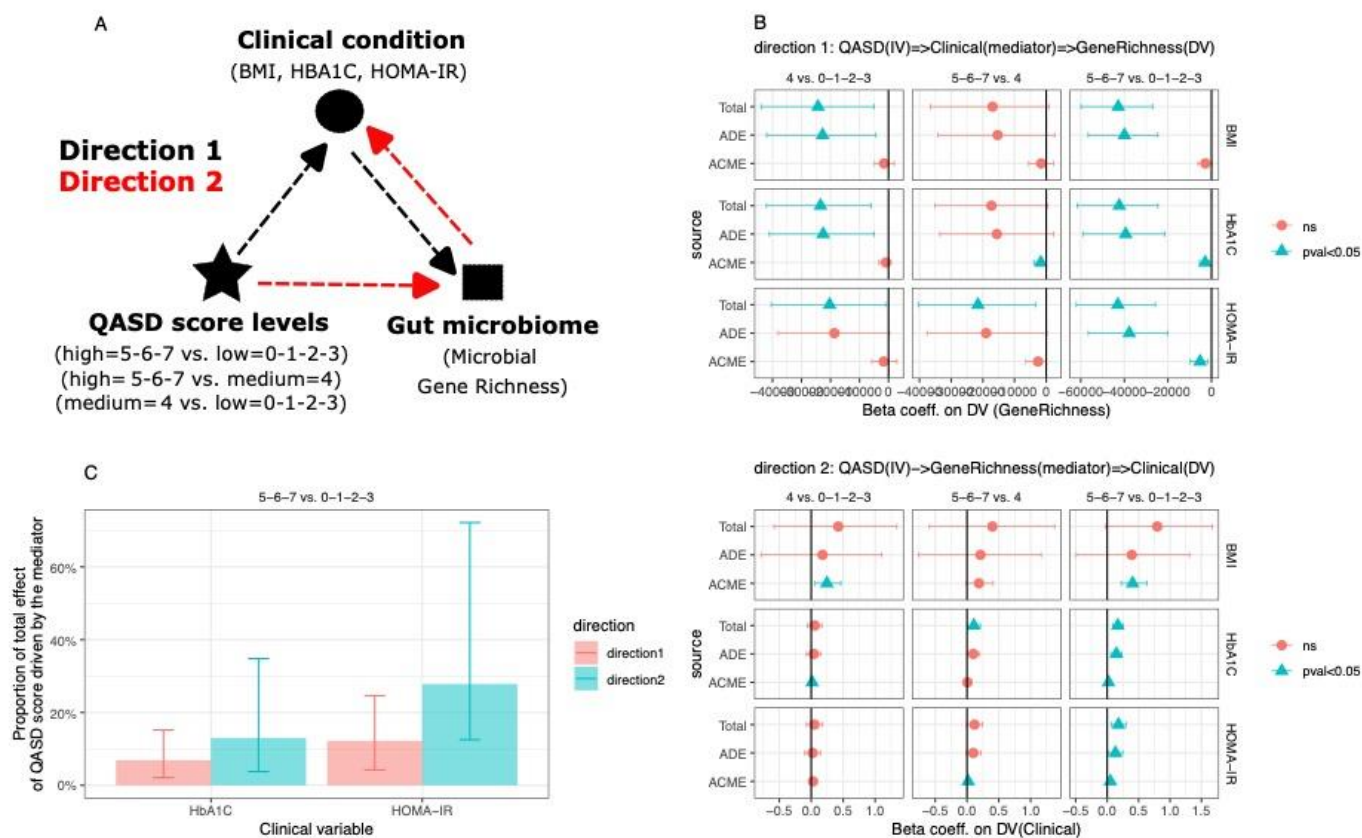
Figure 2: Causal mediation analyses on the impact of QASD score on the gut microbiome and clinical conditions in Metacardis population. (A) Schematic representation of the two-mediation hypothesis tested to evaluate the impact of QASD score (independent variable) on the gut microbiome and clinical profile of individuals. In direction 1 the QASD score would impact gut microbiome (GMGR; dependent variable) mediated by alterations in clinical profile (mediator). In direction2 the QASD score would impact the clinical profile (dependent variable) mediated by alterations in the gut microbiome (GMGR; mediator). BMI, glycated haemoglobin and HOMA-IR have been tested as clinical variables. Pairwise QASD score levels compared were low (0-1-2-3) vs. medium (4), low vs. high(5-6-7), and medium vs. high. Mediation analyses were adjusted by center of recruitment, age, gender and intake of metformin, statin and PPI. (B) Confidence intervals of the beta coefficients corresponding to the total effect (Total), Average Direct Effect (ADE) and Average Causal Mediation Effect (ACME) of the QASD score on the dependent variable in each direction (GMGR in direction 1; clinical variables on direction 2). Color and shape reflect the significance of the effects in mediation analyses. Only for extreme levels of the QASD score (high vs. low) vs. glycated haemoglobin and HOMA-IR we observed an overall significant
