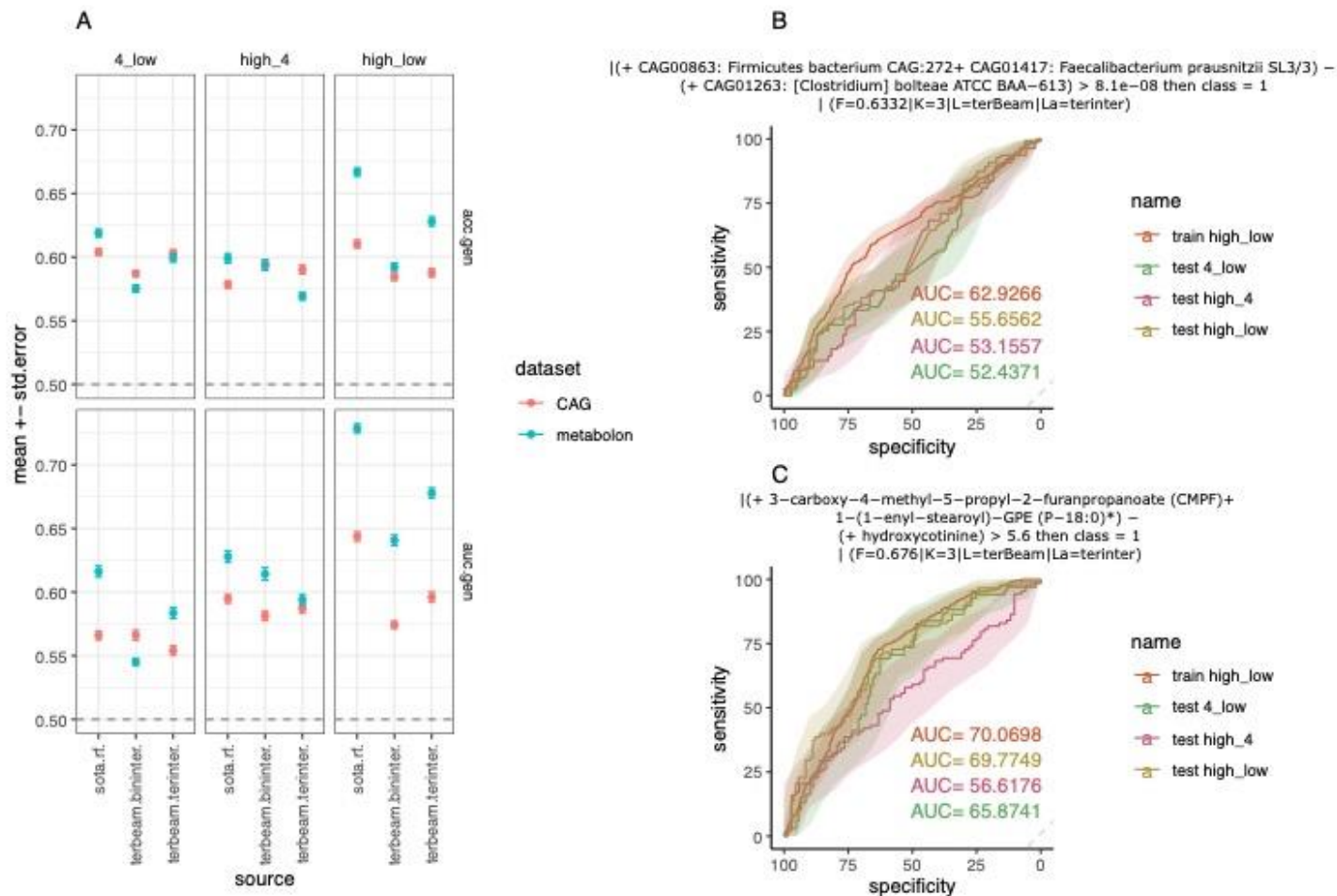
Suppl. Figure 5: Predictive power of metagenomic and metabolomic features across pairwise levels of the QASD score. (A) mean \pm standard error of accuracy (acc) and AUC of predictions between pairwise levels of the QASD score (3 levels decomposition) of best models based on random forest (sota.rf) and binary and ternary Predomics models built with terbeam learner. Models were trained on 80% of the data on 10 times 10-fold cross-validation schema on 135 MGS and 272 serum metabolites (metabolon quantification) product of deconfounding analyses (OK_sd status, FDR<0.1, absolute Cliff's Delta effect size>0.1). (B) ROC curves of the best ternary model trained to classify individuals between high vs. low levels of the QASD score on the training data and holdout datasets (20% of the data not seen during training) based on MGS features. (C) Same as (B) based on metabolomic features
