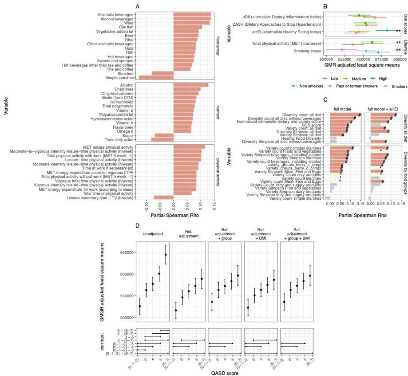
Figure 1 alternative Dietary and physical activity factors, diet variety and diversity scores and a composite lifestyle score associated with Gut Microbiota Gene Richness (GMGR) in MetaCardis population. (A) Barplot of 43 food groups, nutrients and physical activity variables significantly associated with GMGR (FDR<0.05; partial Spearman's rank coefficient correlation with GMGR, adjusted on age, center of recruitment, energy intake in kcal, antibiotics treatments (number of treatments in past five years), metformin (yes/no), statin (yes/no) and PPI (yes/no) medications. (B) Dietary scores (aHEI, DASH, aDII) and lifestyle factors (Total physical activity and Smoking status) associated with GMGR. For diet scores and total physical activity, the variables were divided in tertiles (low/medium/high), and estimated marginal means of GMR across levels of the variables derived from linear regression models adjusted on age, center of recruitment, energy intake in kcal, antibiotics treatments (number of treatments in past five years), metformin (yes or no), statin (yes or no) and PPI (yes/no) medications are represented (**=FDR<0.05; ANOVA tests on linear regression models). (C) Associations of 25 Dietary diversity and variety scores with GMGR (*: p-value<0.05; #: FDR<0.05; partial
