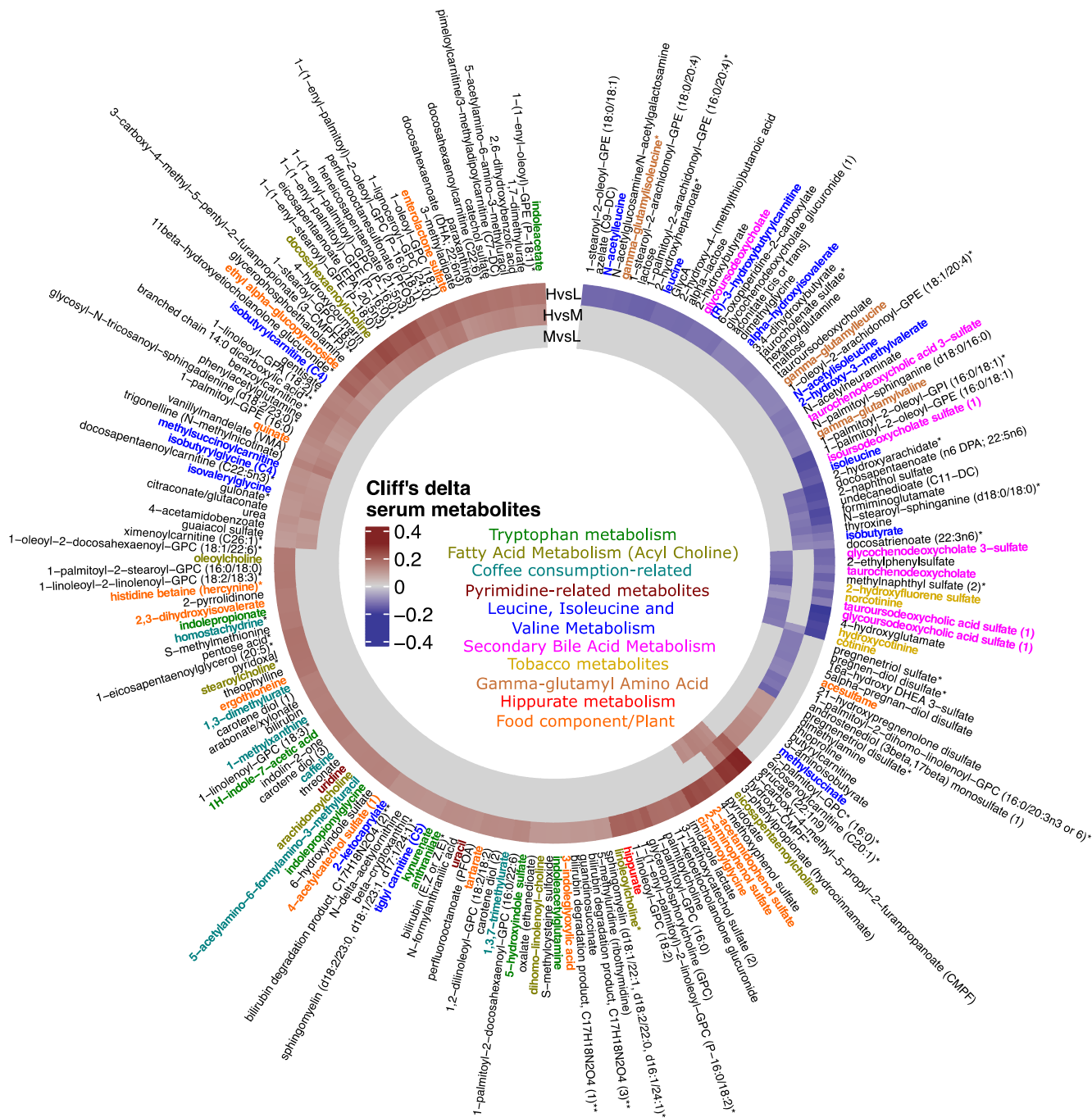
Figure 5: Metabolites significantly altered between levels of the lifestyle score: Circle plot showing at each layer the effect sizes (cliff's delta) of 204 annotated serum metabolites with significant differences between levels of the lifestyle scores (HvsL=High vs. Low; HvsM=High vs. Medium; MvsL=Medium vs. Low; Low=QASD 0,1,2,3; Medium = 4; High 5,6,7) and strictly deconfounded by intake of metformin, statin, PPI and MetaCardis clinical groups according to metadeconfoundR results (FDR<0.1, OK_sd status and absolute Cliff's delta effect sizes greater than 0.1). Positive values correspond to higher abundance of the metabolite in the reference level of the pairwise comparison (p.ex. in HvsL, Cliff's delta>0=High abundance in level high of the lifestyle score vs. level Low; Cliff delta<0=Low abundance in level high of the lifestyle score vs. level Low). The full list of 319 metabolites with significant differences between levels of the lifestyle scores are provided in Supplemental Table S7.
