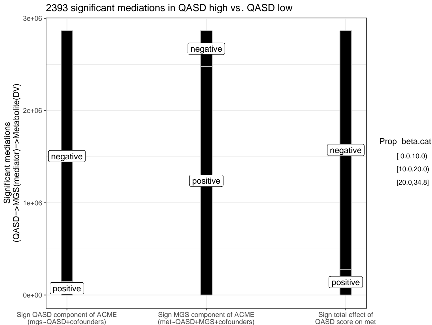
Suppl. Figure 8: Summary of the different types of causal mediation relationships between QASD score (causal factor) → MGS (mediator) → Serum metabolite (outcome variable). Alluvial diagram showing the 2393 inferred causal mediation relationships in direction 1 (QASD score (high vs. low) impacts on serum metabolite levels mediated by MGS abundances) decomposed by the sign of the beta coefficients in the QASD component of the ACME, the MGS component of the ACME and the total effect of the QASD score on the serum metabolite levels. Positive mediations are considered those where the sign of the MGS component of the ACME is positive (serum metabolite and MGS positively associated), whereas negative mediations are those where this sign is negative (serum metabolite and MGS negatively associated).
