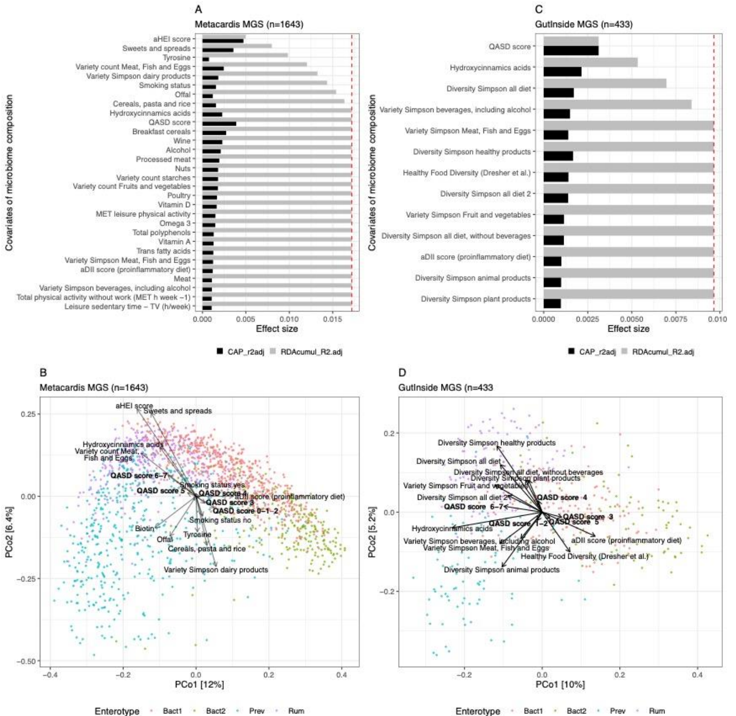
Figure 3: Evaluation of the links between lifestyle on microbiome composition in the Metacardis and GutInside cohorts: (A) 30 of the 47 nutritional variables with highest significant impact over microbiome composition in individuals of the MetaCardis cohort (n=1643; distance-based redundancy analysis, dbRDA; Bray-Curtis dissimilarity from MGS abundance data), either independently (univariate effect sizes in black; FDR<0.01 in dbRDA) or in a multivariate model (cumulative effect sizes in gray, n=9 variables). The
