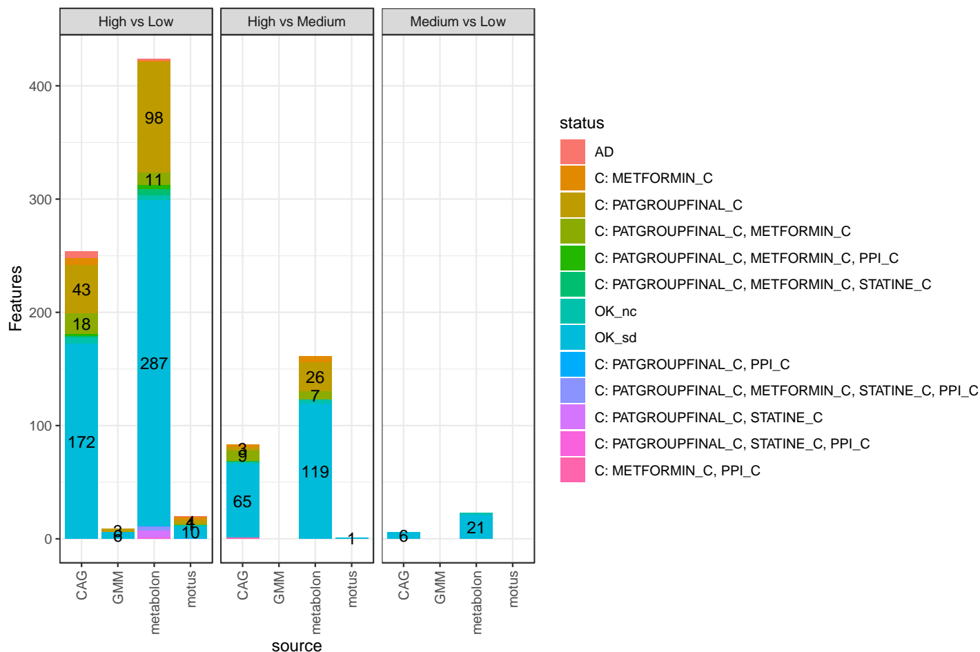
Suppl. Figure 4: Summary of alterations in the microbiome and metabolome features (x-axis) between pairwise levels of the QASD score: Number of features in different spaces showing significant variations in between pairwise levels of the lifestyle score in metadecomfoundR analyses colored by the status of the association (AD: Ambiguously deconfounded, C: Confounded by the corresponding variables; OK_nc=No other covariates; OK_sd=Strictly deconfounded=The hardest label to reach, meaning that another covariate is associated to the feature but the signal can be reduced to the pairwise level of the lifestyle scores.)
