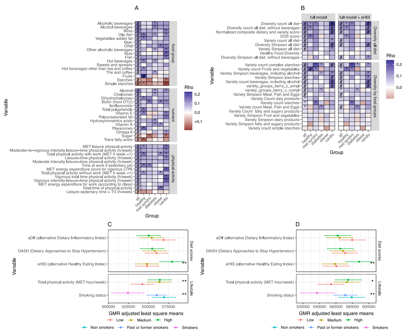
Suppl. Figure 1: Sensitivity analysis on dietary and physical activity factors, diet variety and diversity scores associated with GMGR in MetaCardis population (A) Heatmap representing the coefficients of partial Spearman correlations between GMGR and
