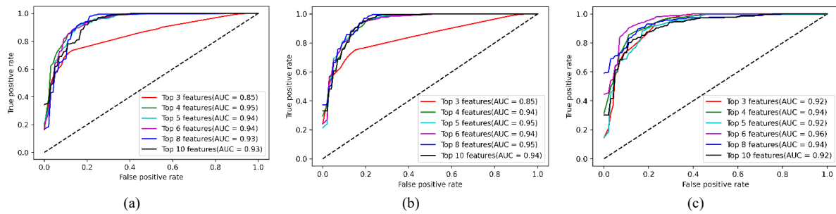
Figure 4: ROC curve and AUC of top three performing models (a) RF (b) XGBoost (c) LSTM
