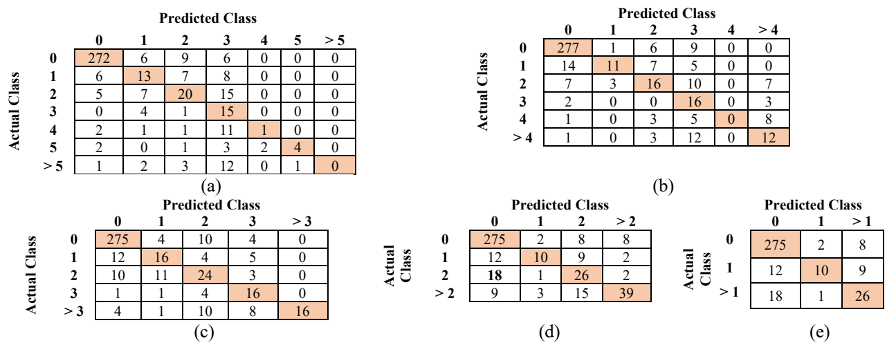
Figure 9: Confusion Matrix of ventilated days prediction (a) 7 class 10 features (b) 6 class 8 features (c) 5 class 10 features (d) 4 class 10 features (e) 3 class 10 features
