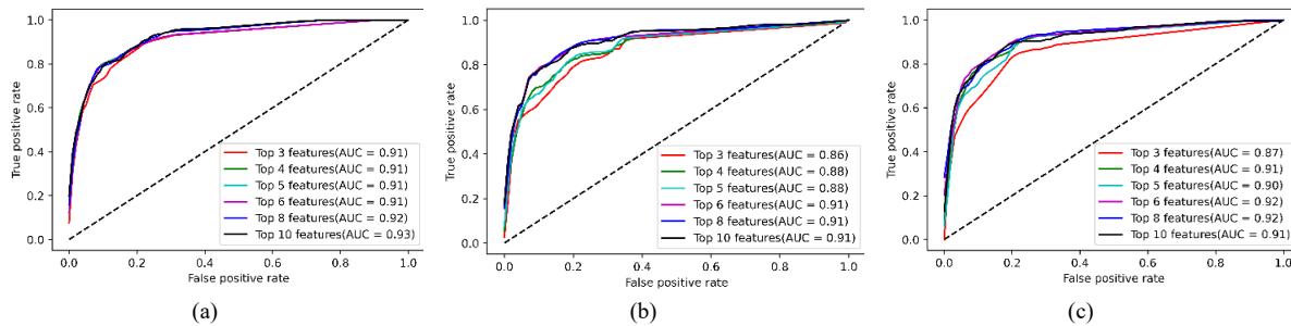
Figure 6: ROC curve and AUC of top three performing models for predicting “ICU Requirement” using original data. (a) XGBoost, (b) LDA and (c) LSTM
