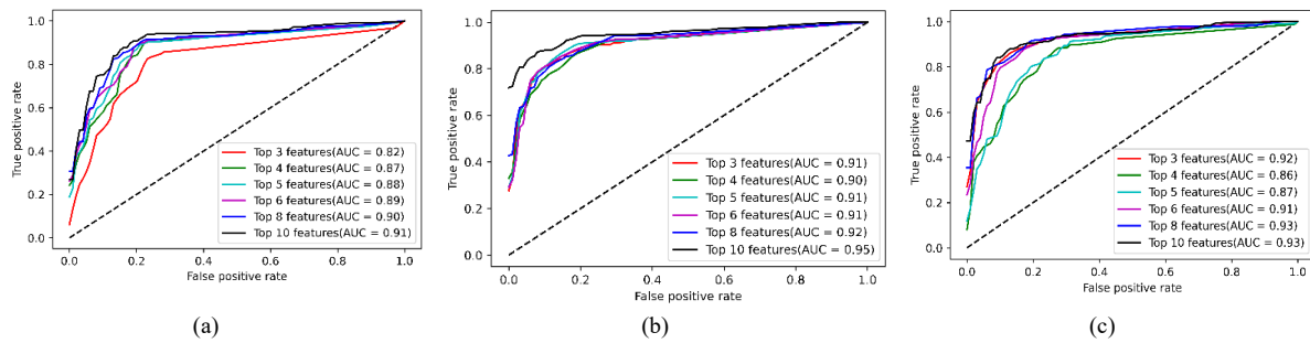
Figure 7: ROC curve and AUC of top three performing models for predicting “ICU Requirement” using under-sampled data. (a) SVM, (b) DNN and (c) LSTM.
