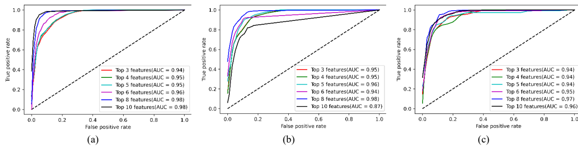
Figure 5: ROC curve and AUC of top three performing models (a) RF (b) DNN (c) LSTM
