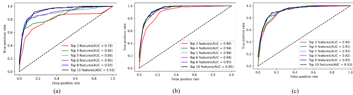
Figure 3: ROC curve and AUC of top three performing models (a) SVM (b) XGBoost (c) LDA
