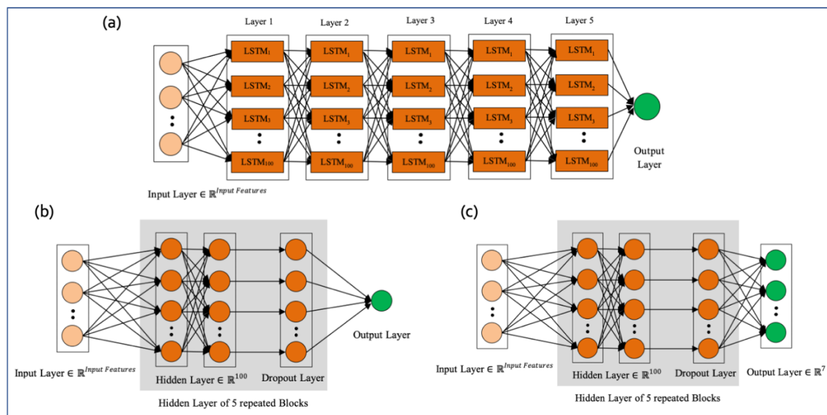
Figure 1: Model architecture (a) Long Short-Term Memory (LSTM) and (b) Deep Neural Network (DNN) architecture for predicting “last status” and “ICU requirement”. (c) DNN architecture for predicting “Ventilation days”.
