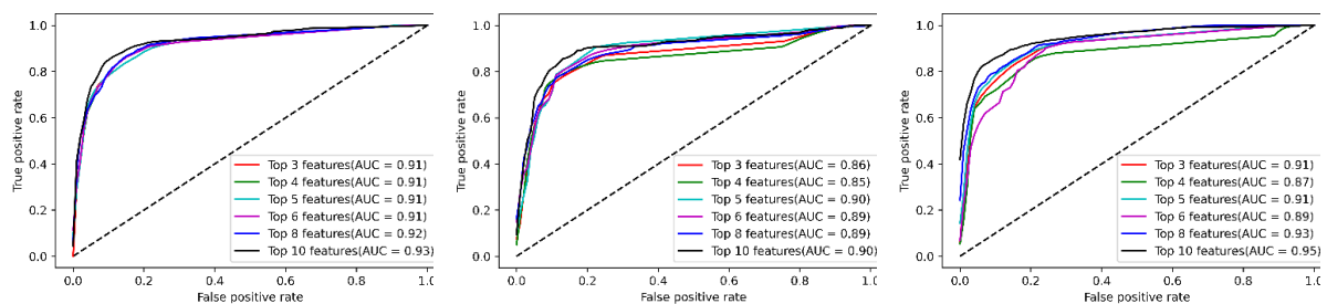
Figure 8: ROC curve and AUC of top three performing models for predicting “ICU Requirement” using oversampled data. (a) RF, (b) SVM and (c) LSTM.
