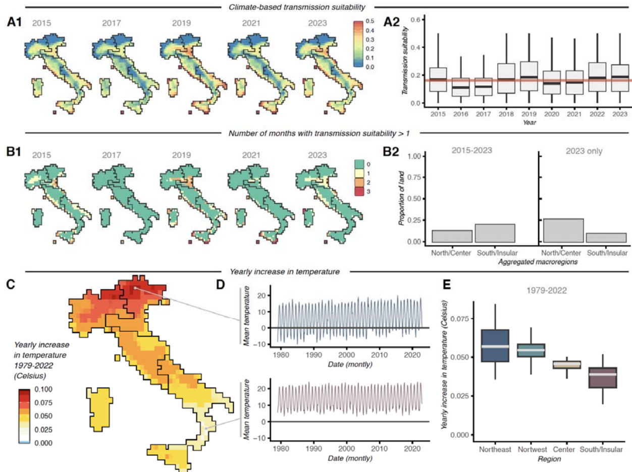
251 252 Figure 4. Climate-based Suitability of Dengue in Italy. A1) Yearly mean climate-based transmission suitability (index P) per 253 geographical pixel of the climate satellite data; presented are a subset of years. A2) Distributions of suitability values per year. 254 The light red horizontal line marks the historical mean (2015-2023). B1) Yearly number of months in which climate-based 255 transmission suitability (index P) per geographical pixel of the climate satellite data was above 1; presented are a subset of years. 256 B2) Proportion of land (of geographical pixels available in climate data) that present suitability above 1 for at least 1 month of the 257 year. Presented are the historical period (2015-2023) and 2023 only. North/Center is the aggregation of the Northwest, Northeast 258 and Center macroregions. C) Map of Italy with estimates of rate of increase (linear slope) in mean yearly temperature (color 259 legend). Black boundaries are macroregions. D) Time series of mean monthly temperature (1979-2022) for two geolocations as 260 marked on panel D. Line coloring follows the corresponding macroregion. E) Distributions of rates of increase (linear slopes) for 261 each of the macroregions (as presented in panel D).
