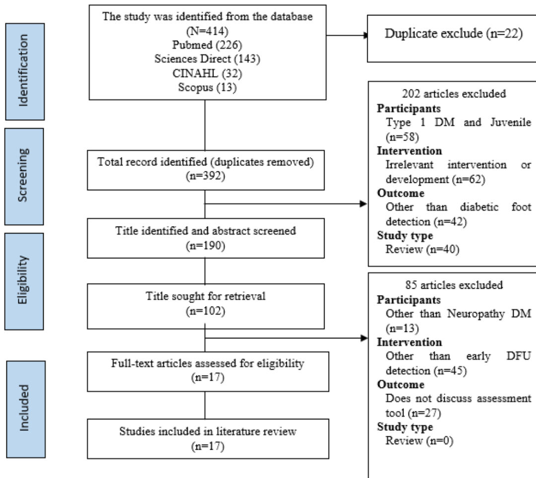
Figure 1. Preferred Reporting Items for Systematic Review and Meta Analysis (PRISMA)
