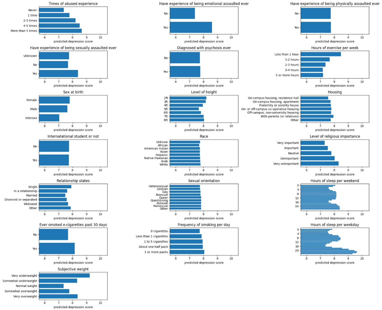
Supplemental Figure 2. Partial dependence plot for rest variables in sequence of binary XGBoost models.
