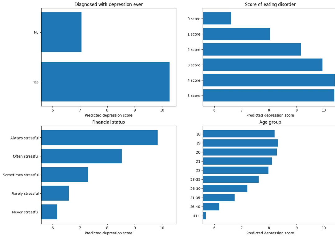
Figure 5. Partial dependence of depression history, eating disorder, financial status, and age group.
