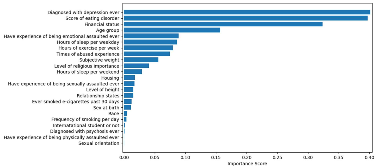
Figure 4. Permutation importance score in MAE of each predictor in sequence of binary XGBoost models.
