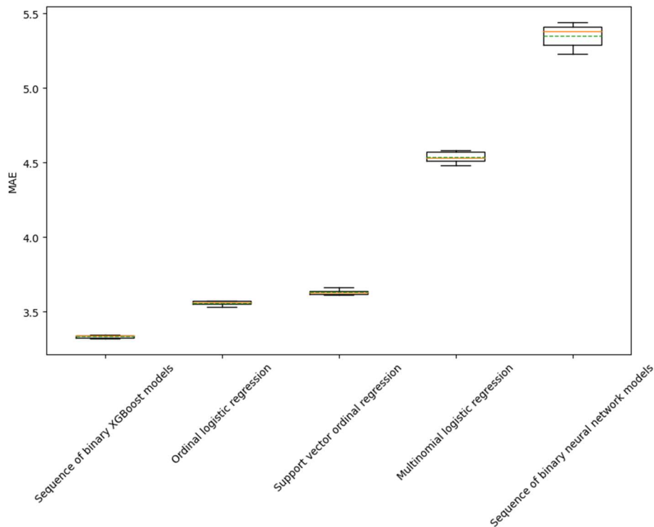
Figure 3. MAE of potential multi-class models to predict overall depression.
