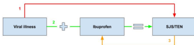
Figure 1: Directed acyclic graph showing possible associations between the observed pharmacovigilance signal suggesting increased reports of SJS-TEN with ibuprofen use.
