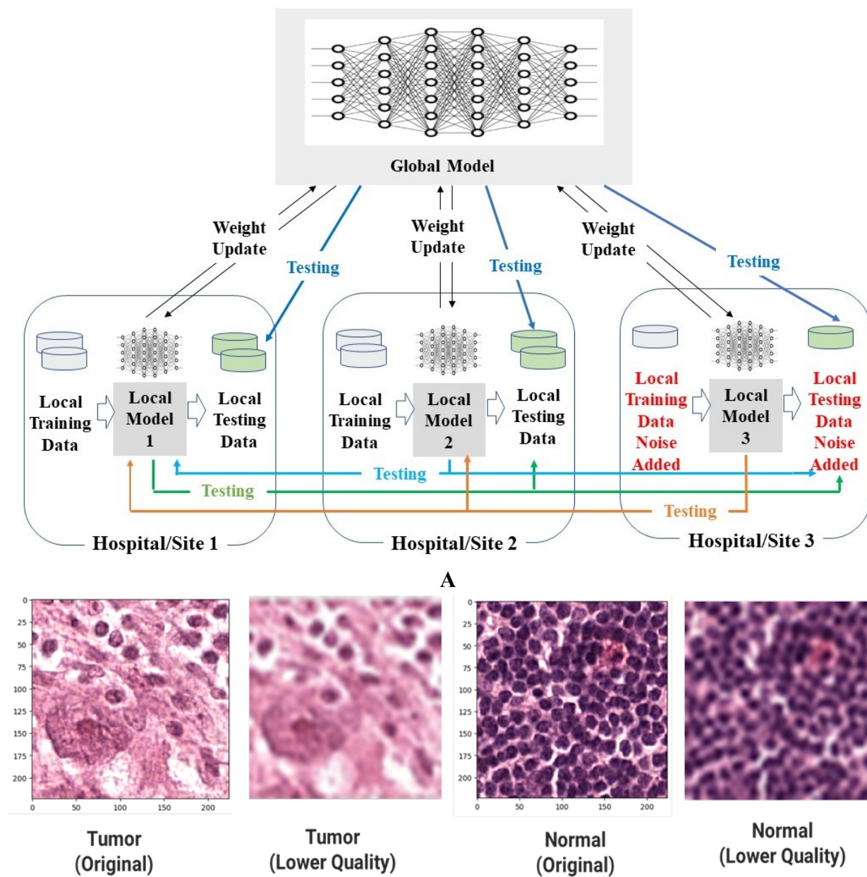
Figure 4. Experiment design to evaluate performance of federated model in improving diagnostic performance on lower quality images at a local site.
