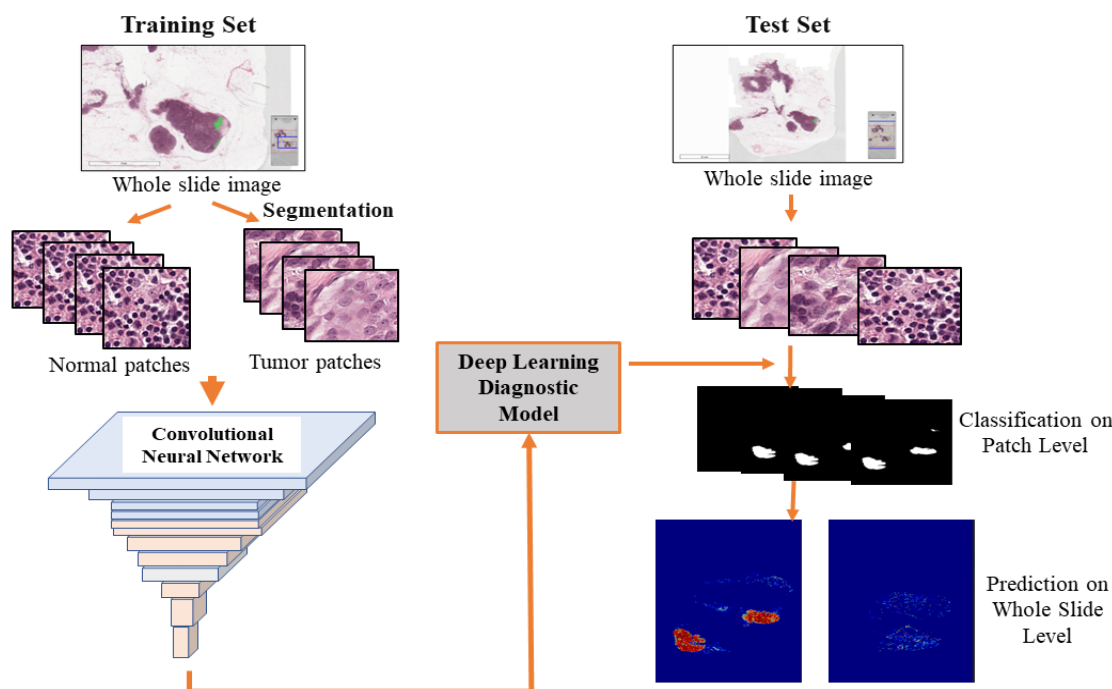
Figure 2. The Workflow of Deep Learning-Based Metastatic Breast Cancer Prediction
