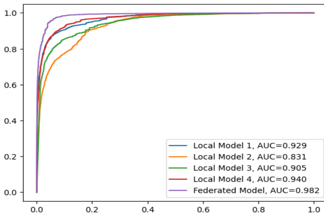
Figure 5. Receiver Operating Characteristics (ROC) curves of the federated model as compared with the local models from 4 collaborating sites.
