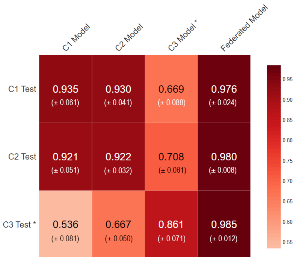
Figure 6. Diagnostic performance of the local models and federated model (average ROC AUC \pm Standard Deviation): testing on respective test sets at individual institutions. * For institution 3, the histopathological images for training and testing were augmented to simulate images of lower quality.
