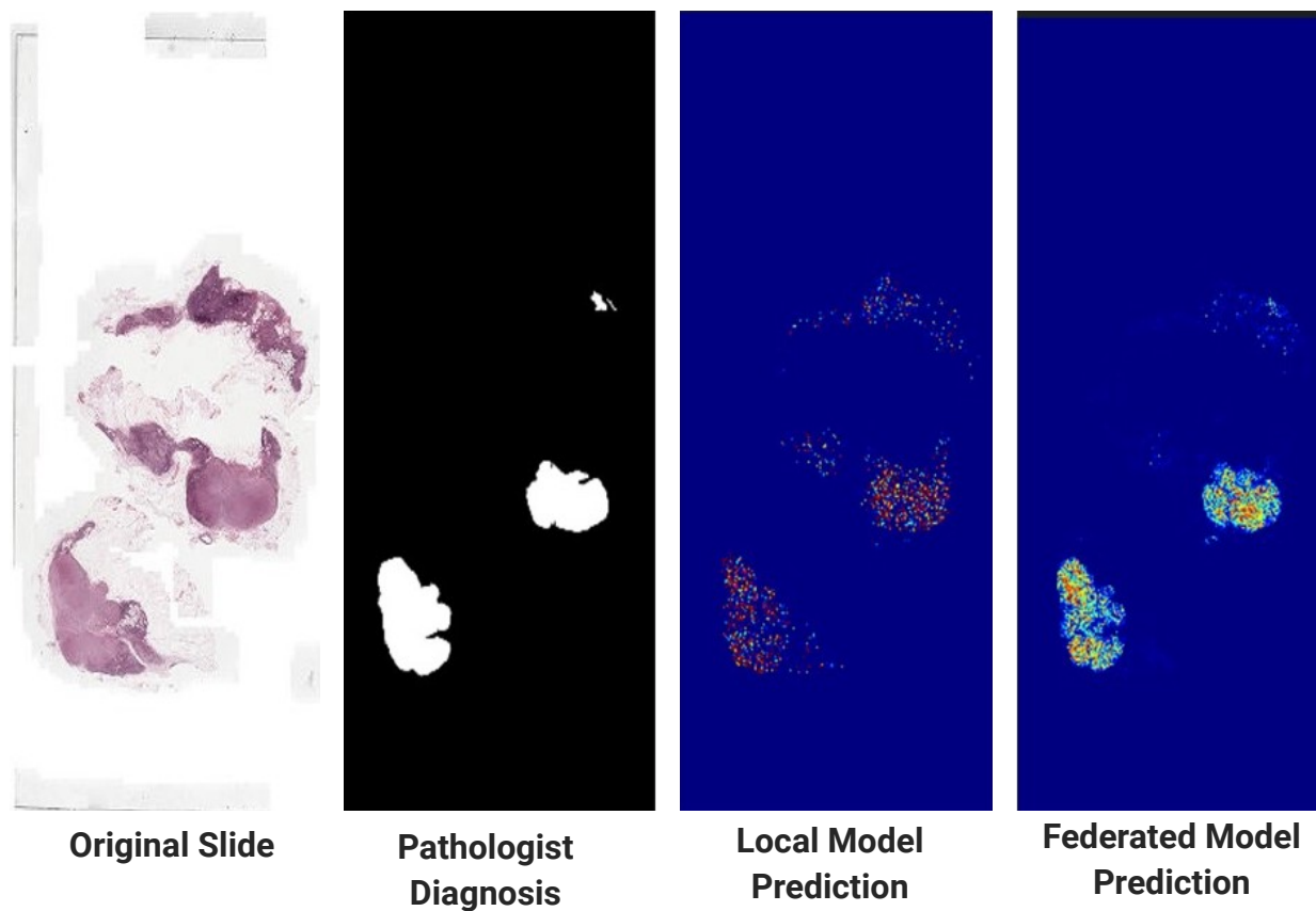
Figure 7. Tumor case A: comparison between the local model prediction and the federated model prediction on cancerous regions on WSI, with the pathologist's diagnosis as ground truth
