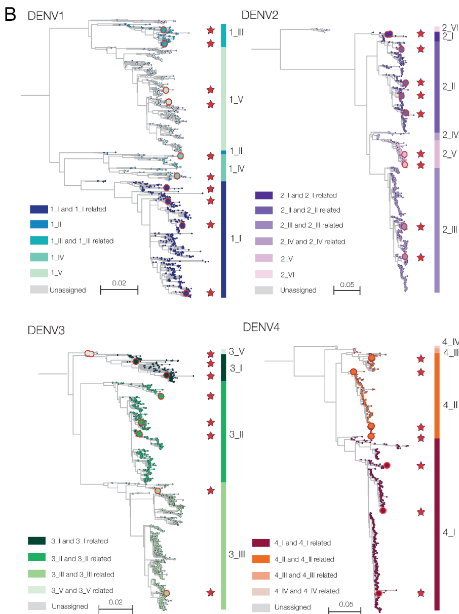
Fig. 1: Overview of the DengueSeq primer design. A) For each of the four serotypes, a selection of genetically diverse genomes was made as input for PrimalScheme. Using PrimalScheme, four serotype-specific primer schemes were generated. Each scheme consists of 35-37 primer pairs which
