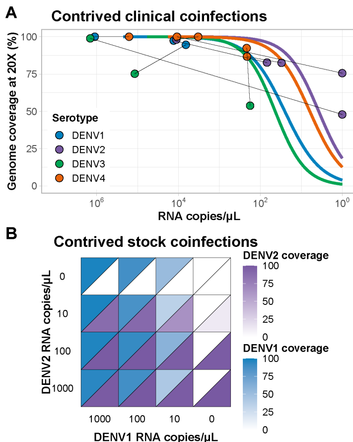
Fig. 5: Detection of dengue virus coinfections using the pan-serotype primer scheme. A) Clinical specimens containing different dengue virus serotypes were mixed to create contrived coinfections. A total of 8 contrived samples were created by mixing two different clinical specimens. Dots represent individual samples connected with lines to indicate mixed pairs and colored lines are expected genome coverage estimated from fitted logistic regression lines determined based on coverage data from Fig. 4. B) Two virus stocks (serotypes 1 and 2) were serially diluted and mixed at different concentrations to represent a range of virus titers in contrived stock coinfections.
