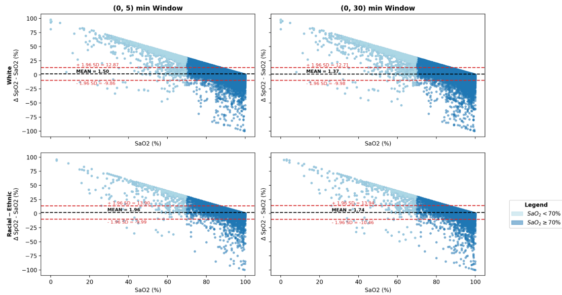
SaO 2 -SpO 2 Modified Bland-Altman Plots
