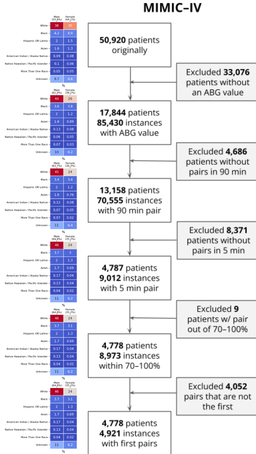
Figure 3b. Flow diagram for MIMIC-IV depicting cohort selection.
