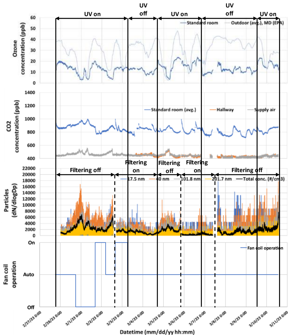
359 360 Figure 5. Standard hotel room O 3 , CO 2 , and UFP measurements from February 27 through March 11, 361 2023. Periods with far-UVC lamps and in-room HEPA filtering on and off and fan coil unit states (on, off 362 and auto) are shown. During the auto state, the fan coil unit ran intermittently as controlled by a 363 thermostat and motion sensor. During the filtering periods the fan coil unit had a MERV 13 filter and the 364 HEPA filter unit had a HEPA filter but they had no filter during other times. 365
