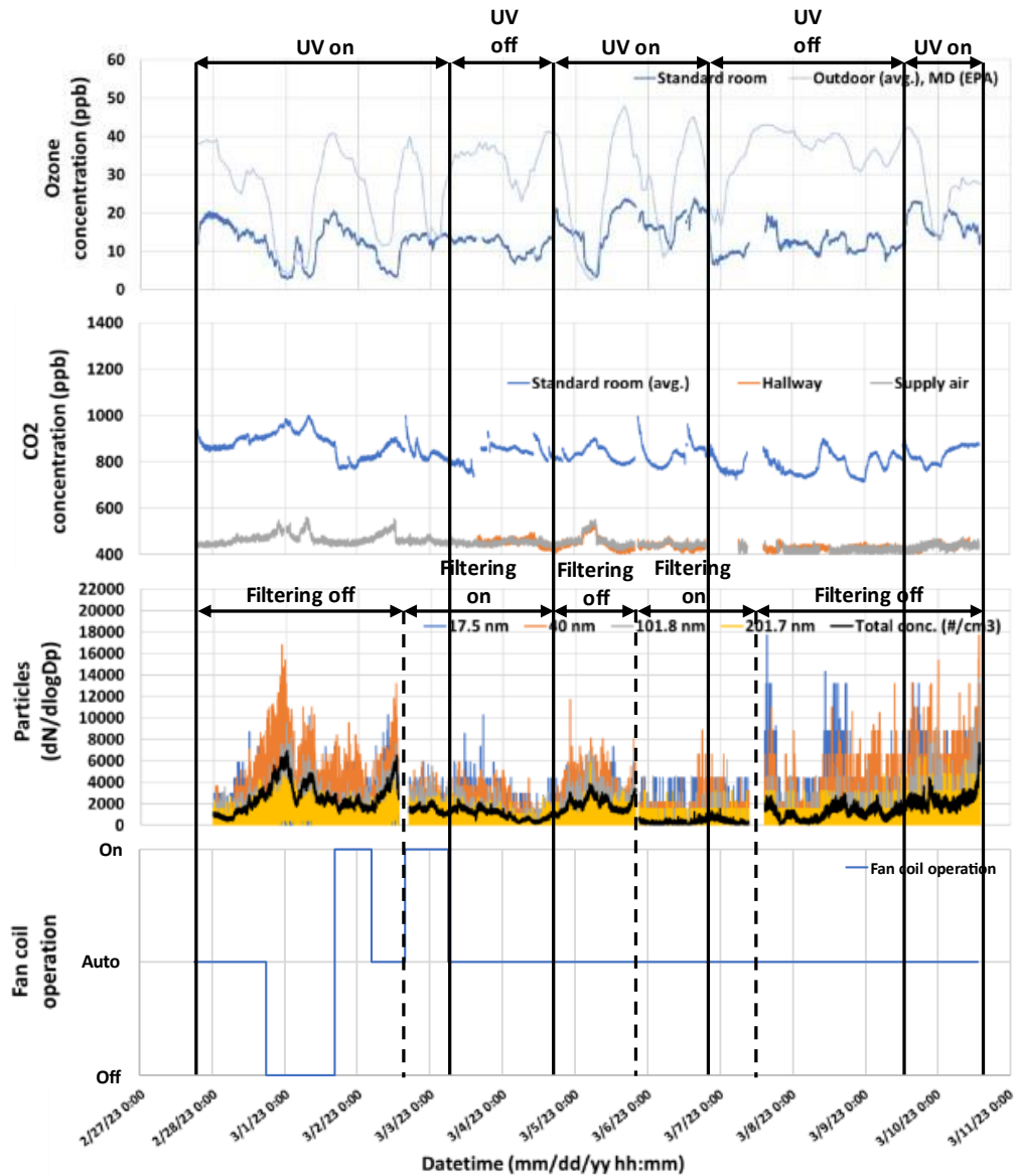
360 Figure 5. Standard hotel room O 3 , CO 2 , and UFP measurements from February 27 through March 11, 361 2023. Periods with far-UVC lamps and in-room HEPA filtering on and off and fan coil unit states (on, off 362 and auto) are shown. During the auto state, the fan coil unit ran intermittently as controlled by a 363 thermostat and motion sensor. During the filtering periods the fan coil unit had a MERV 13 filter and the 364 HEPA filter unit had a HEPA filter but they had no filter during other times.
