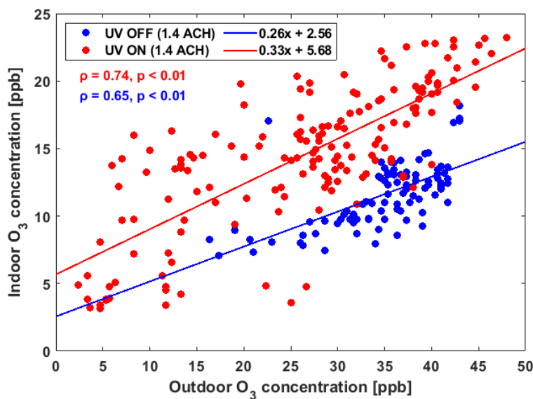
366 367 Figure 6. Indoor versus outdoor O 3 concentrations for the standard hotel room when far-UVC lamps were 368 on and off (with an average air exchange rate of 1.4 ACH). The outdoor O 3 levels are an average of three 369 Maryland sites (Essex, Glen Burnie, Padonia) in the EPA Ambient Air Monitoring Network. \rho is the 370 Spearman's rank correlation coefficient. 371
