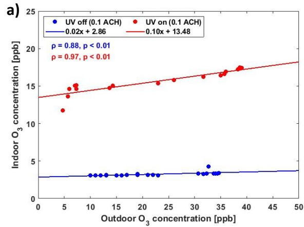
354 Figure 4. Sealed room indoor-outdoor concentration correlations with and without UV with (a) 0.1 ACH 355 (fan coil off) and (b) 0.5 ACH (fan coil on) ventilation rates. The outdoor O 3 levels are an average of three 356 Maryland sites (Essex, Glen Burnie, Padonia) in the EPA Ambient Air Monitoring Network. \rho is the 357 Spearman's rank correlation coefficient.
