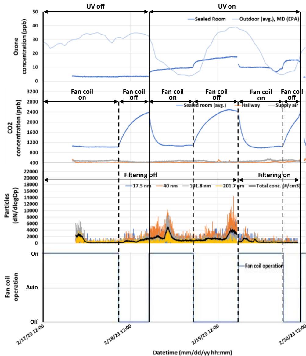
344 345 Figure 3. Sealed room O 3 , CO 2 and ultra-fine particle measurements plotted against time. Periods with 346 far-UVC lamps (on/off), in-room HEPA filtering (on/off) and fan coil unit states (on/off/auto) are shown. 347 Fan coil unit had 2 states: off (0.1 ACH) and on (0.5 ACH). During the filtering periods the fan coil unit had 348 a MERV 13 filter and the HEPA filter unit had a HEPA filter but they had no filter during other times. The 349 outdoor O 3 levels are an average of three Maryland sites (Essex, Glen Burnie, Padonia) in the EPA 350 Ambient Air Monitoring Network. The CO 2 concentration in the sealed room is an average of all sensors 351 in the room. 352
