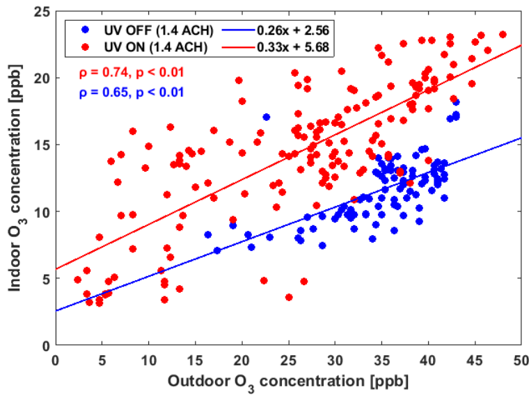
367 Figure 6. Indoor versus outdoor O 3 concentrations for the standard hotel room when far-UVC lamps were 368 on and off (with an average air exchange rate of 1.4 ACH). The outdoor O 3 levels are an average of three 369 Maryland sites (Essex, Glen Burnie, Padonia) in the EPA Ambient Air Monitoring Network. \rho is the 370 Spearman's rank correlation coefficient.
