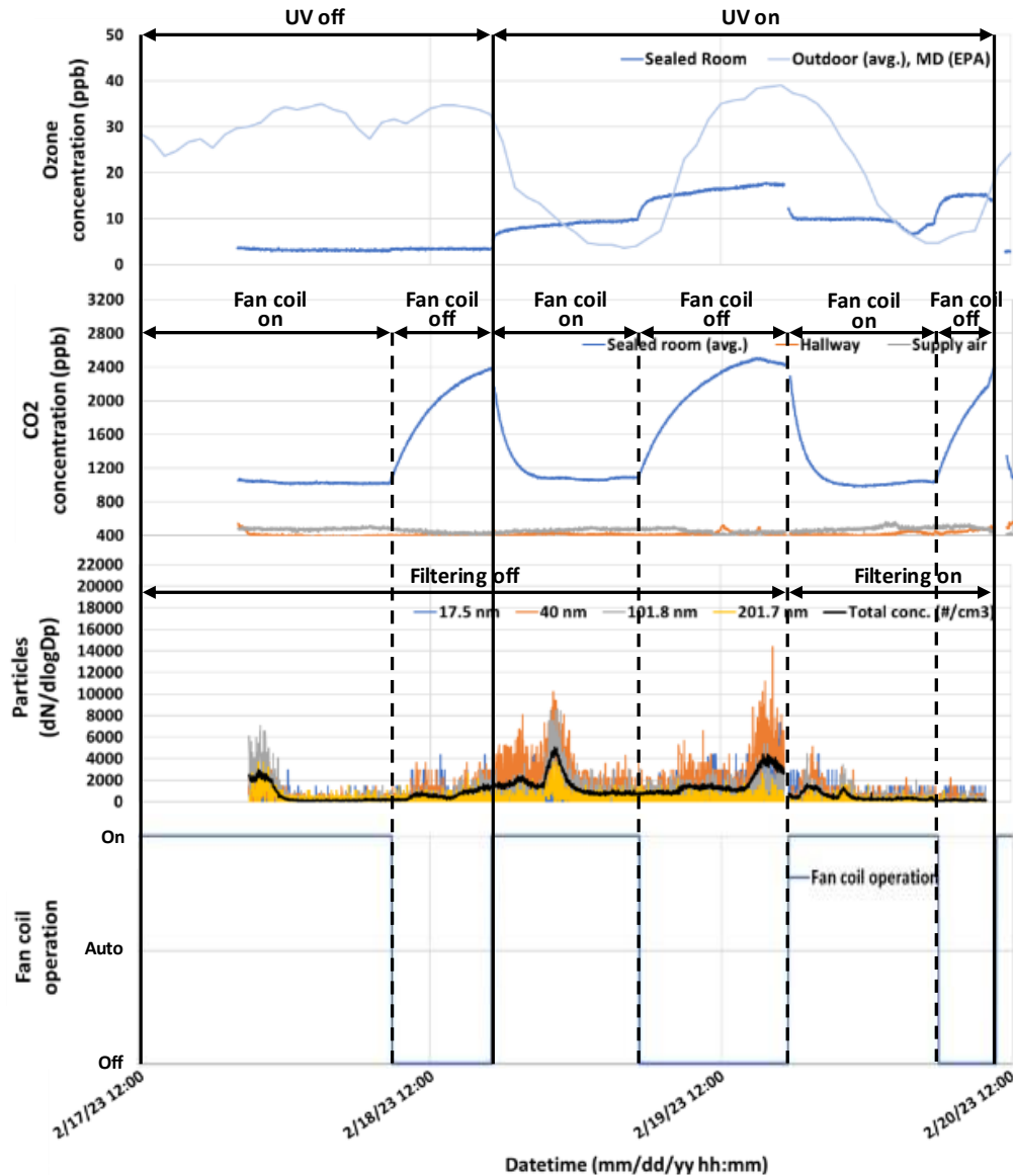
345 Figure 3. Sealed room O 3 , CO 2 and ultra-fine particle measurements plotted against time. Periods with 346 far-UVC lamps (on/off), in-room HEPA filtering (on/off) and fan coil unit states (on/off/auto) are shown. 347 Fan coil unit had 2 states: off (0.1 ACH) and on (0.5 ACH). During the filtering periods the fan coil unit had 348 a MERV 13 filter and the HEPA filter unit had a HEPA filter but they had no filter during other times. The 349 outdoor O 3 levels are an average of three Maryland sites (Essex, Glen Burnie, Padonia) in the EPA 350 Ambient Air Monitoring Network. The CO 2 concentration in the sealed room is an average of all sensors 351 in the room.
