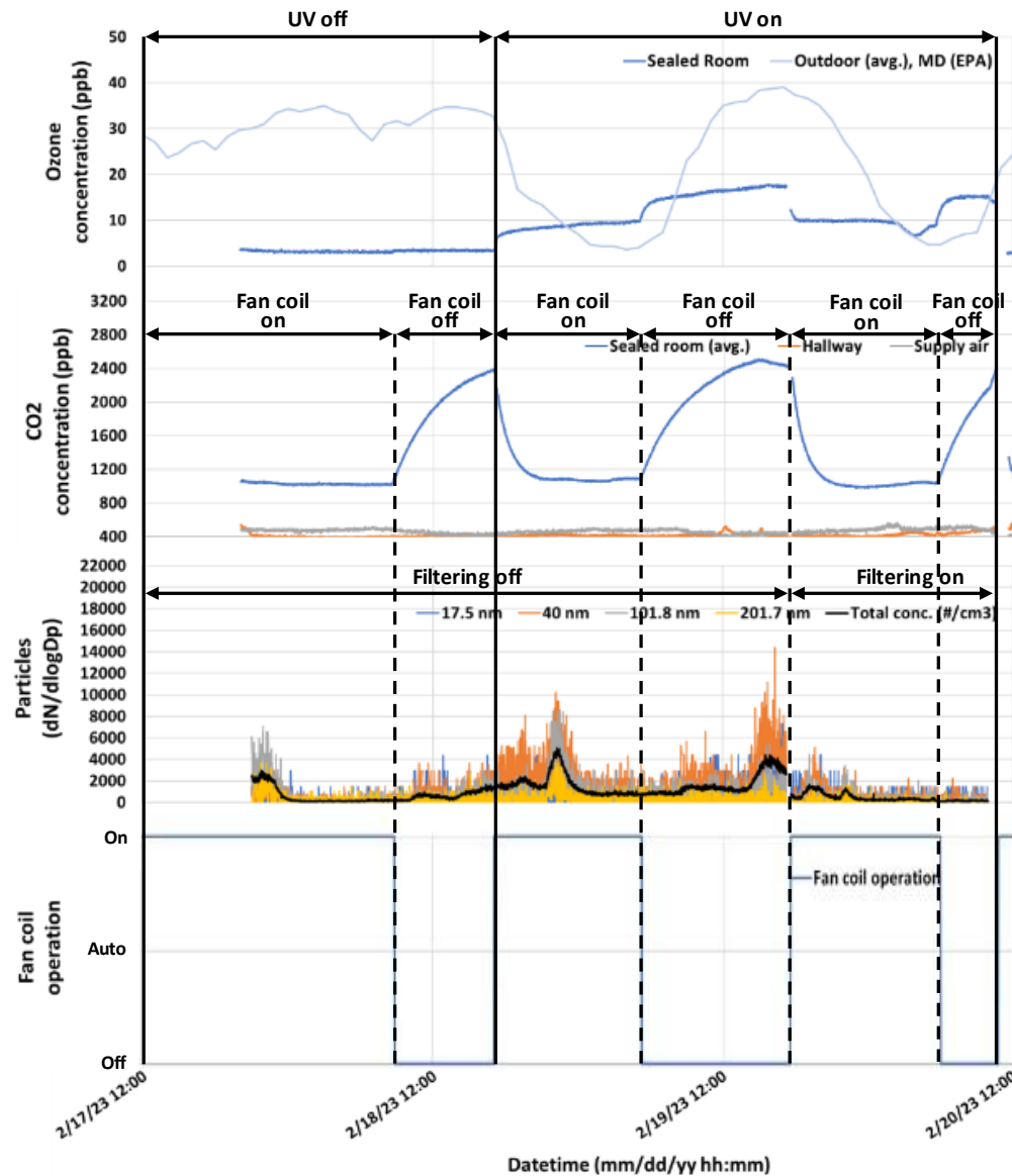
Figure 3. Sealed room O_3 , CO_2 and ultra-fine particle measurements plotted against time. Periods with far-UVC lamps (on/off), in-room HEPA filtering (on/off) and fan coil unit states (on/off/auto) are shown. Fan coil unit had 2 states: off (0.1 ACH) and on (0.5 ACH). During the filtering periods the fan coil unit had a MERV 13 filter and the HEPA filter unit had a HEPA filter but they had no filter during other times. The outdoor O_3 levels are an average of three Maryland sites (Essex, Glen Burnie, Padonia) in the EPA Ambient Air Monitoring Network. The CO_2 concentration in the sealed room is an average of all sensors in the room.
