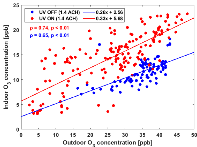
Figure 6. Indoor versus outdoor O 3 concentrations for the standard hotel room when far-UVC lamps were on and off (with an average air exchange rate of 1.4 ACH). The outdoor O 3 levels are an average of three Maryland sites (Essex, Glen Burnie, Padonia) in the EPA Ambient Air Monitoring Network. \rho is the Spearman's rank correlation coefficient.
