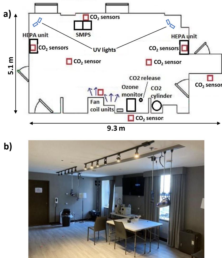
Figure 1. Sealed unfurnished hotel room. a) Floor plan (room height: 2.4 m) and position of far-UVC lamps and sampling equipment. b) Photograph showing SMPS between windows, vinyl flooring, far-UVC lamps and minimal furnishings. Floor plan not in scale.
