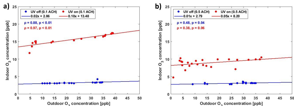
Figure 4. Sealed room indoor-outdoor concentration correlations with and without UV with (a) 0.1 ACH (fan coil off) and (b) 0.5 ACH (fan coil on) ventilation rates. The outdoor O 3 levels are an average of three Maryland sites (Essex, Glen Burnie, Padonia) in the EPA Ambient Air Monitoring Network. \rho is the Spearman's rank correlation coefficient.
