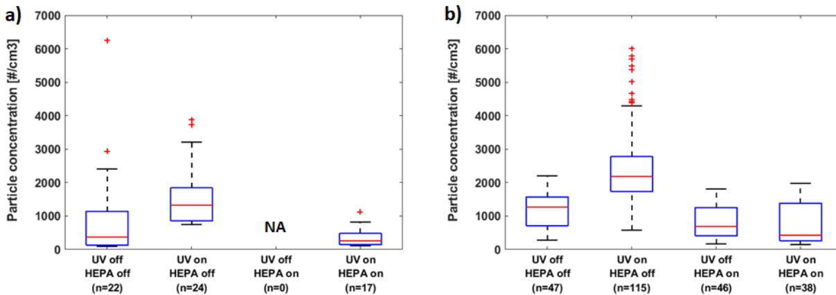
Figure 7. Ultra-fine particle concentrations (17.5 to 289 nm) with and without use of 222 nm far-UVC lamps and HEPA filters a) in the sealed unfurnished room (no data from HEPA on UV off) and b) in the standard room. Boxplots show medians (redline inside the boxes), 25th and 75th percentiles (top and bottom of the boxes), most extreme data not considered outliers (whiskers) and outliers (red crosses) of 1-hr data. n represents the number of 1-hr data points included in each boxplot. HEPA filter units delivered 232 L/s (9.1 ACH) in the sealed room and 116 L/s (7.1 ACH) in the standard room. Simultaneous background measurements to account for indoor and outdoor sources were not collected.
