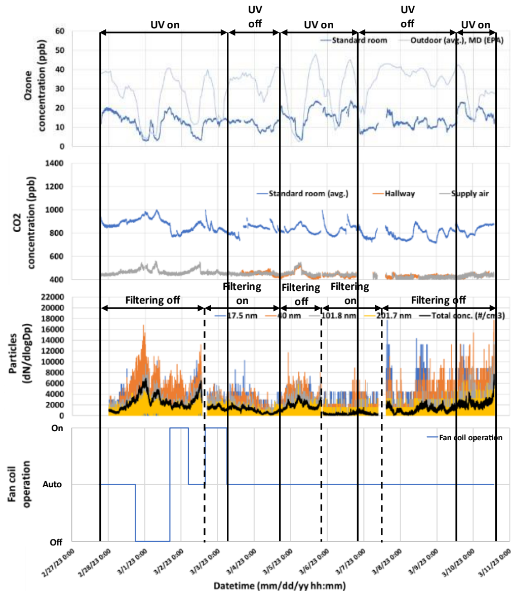
Figure 5. Standard hotel room O 3 , CO 2 , and UFP measurements from February 27 through March 11, 2023. Periods with far-UVC lamps and in-room HEPA filtering on and off and fan coil unit states (on, off and auto) are shown. During the auto state, the fan coil unit ran intermittently as controlled by a thermostat and motion sensor. During the filtering periods the fan coil unit had a MERV 13 filter and the HEPA filter unit had a HEPA filter but they had no filter during other times.
