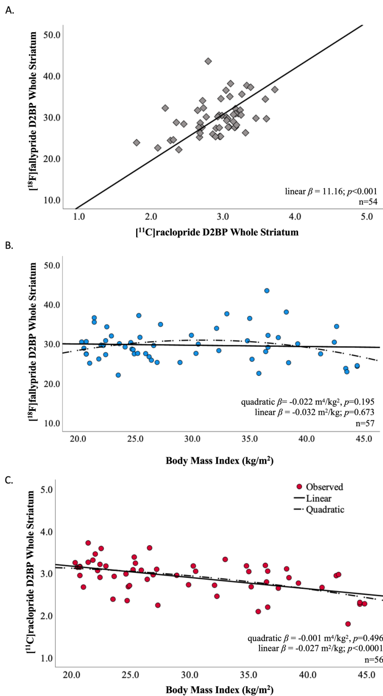
Figure 2. Striatal D2BP as measured within subject by [^{18}\text{F}] fallypride and [^{11}\text{C}] raclopride were correlated but differentially related to BMI. (A) Within-subject measurements of D2BP using [^{18}\text{F}] fallypride and [^{11}\text{C}] raclopride in the overnight fasted state were correlated using the whole striatum in a region of interest analysis. Trendline and slope parameters reflect standard major axis regression. (B) Whole striatal region of interest analysis using [^{18}\text{F}] fallypride indicated no significant relationship between D2BP and BMI. (C) Whole striatal region of interest analysis using [^{11}\text{C}] raclopride indicated a negative linear relationship between BMI and D2BP, but no significant quadratic relationship.
