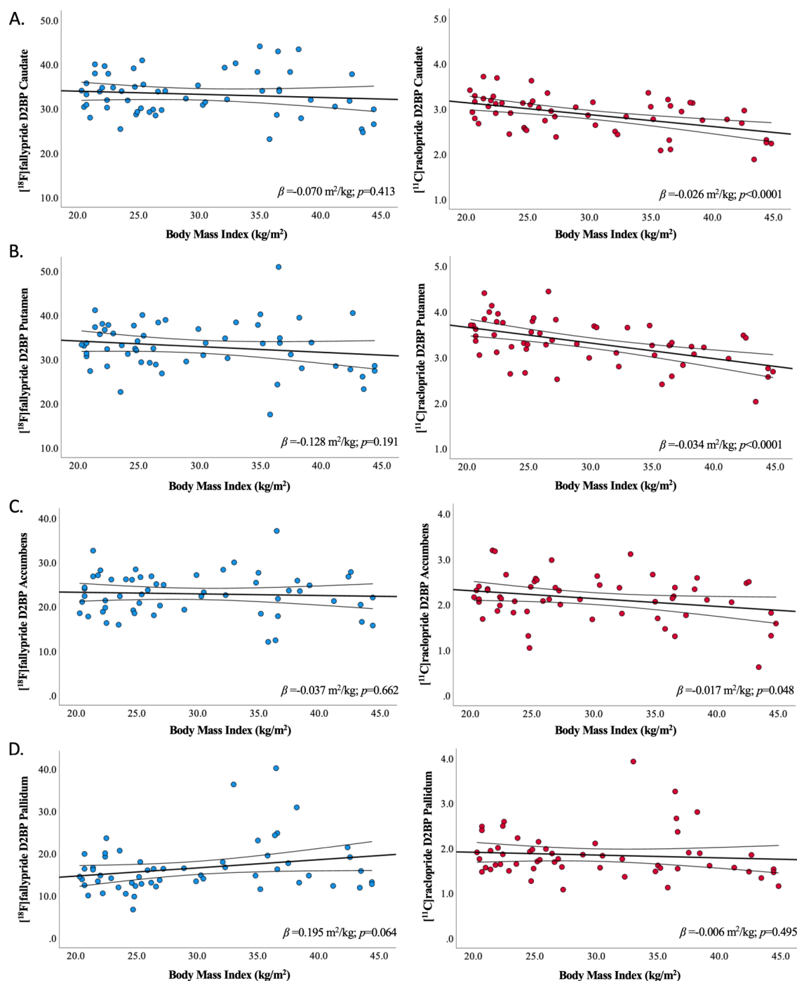
Figure 3. Relationship between BMI and D2BP as measured by [ 18 F]fallypride and [ 11 C]raclopride across striatal regions of interest. Bilateral striatal region of interest analyses reflecting relationships between BMI and D2BP as measured by [ 18 F]fallypride (blue circles, left column; n=57) and [ 11 C]raclopride (red circles, right column; n=56) in (A) caudate, (B) putamen, (C) accumbens, and (D) pallidum. Regression line and 95%CI indicated. ROI analyses are uncorrected for multiple comparisons.
