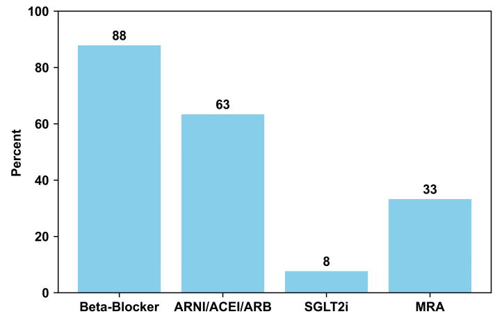
B GDMT Use Among Model-reclassified Patients with HFrEF
