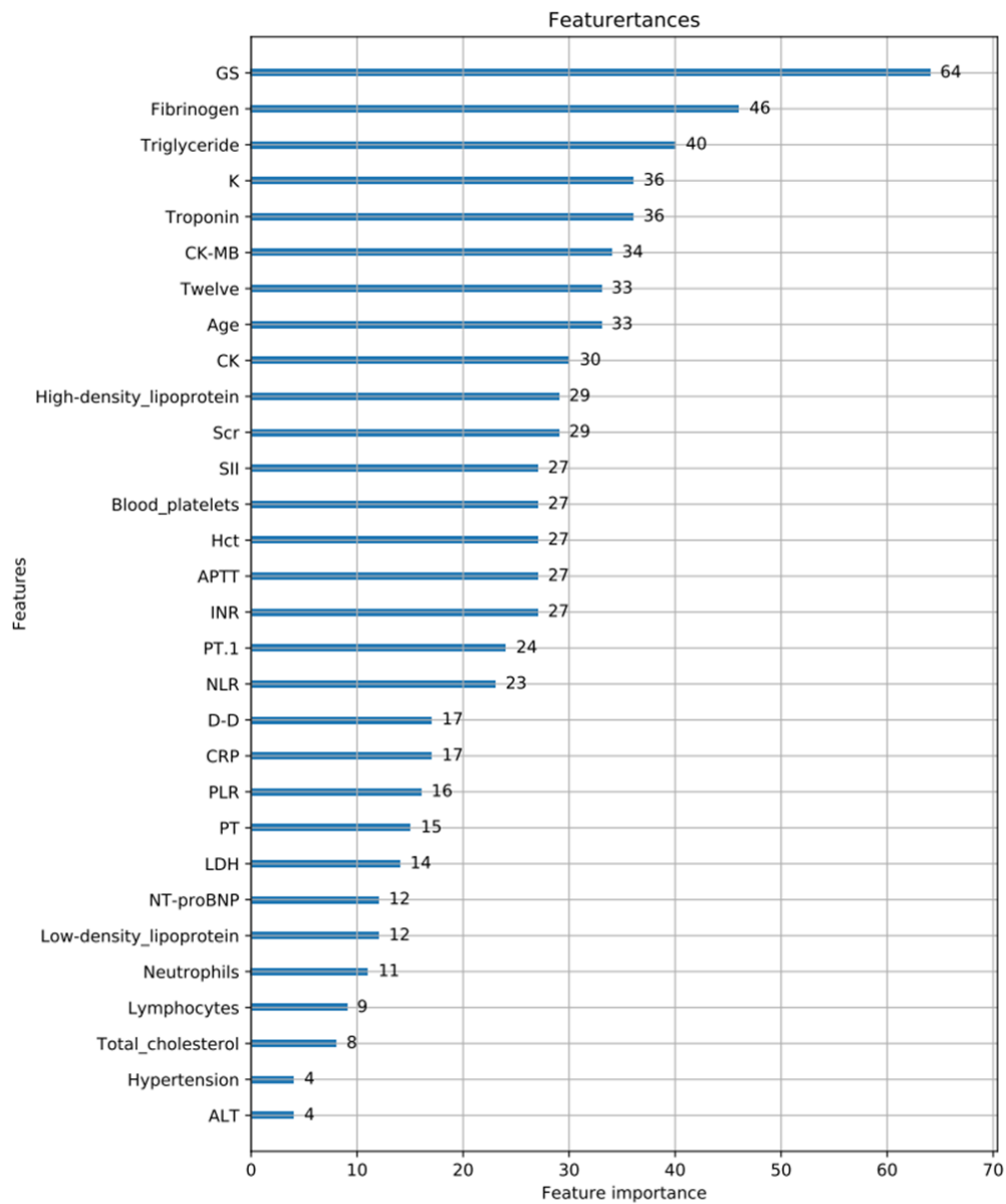
Figure 5. Weighted feature map for XGBoost
