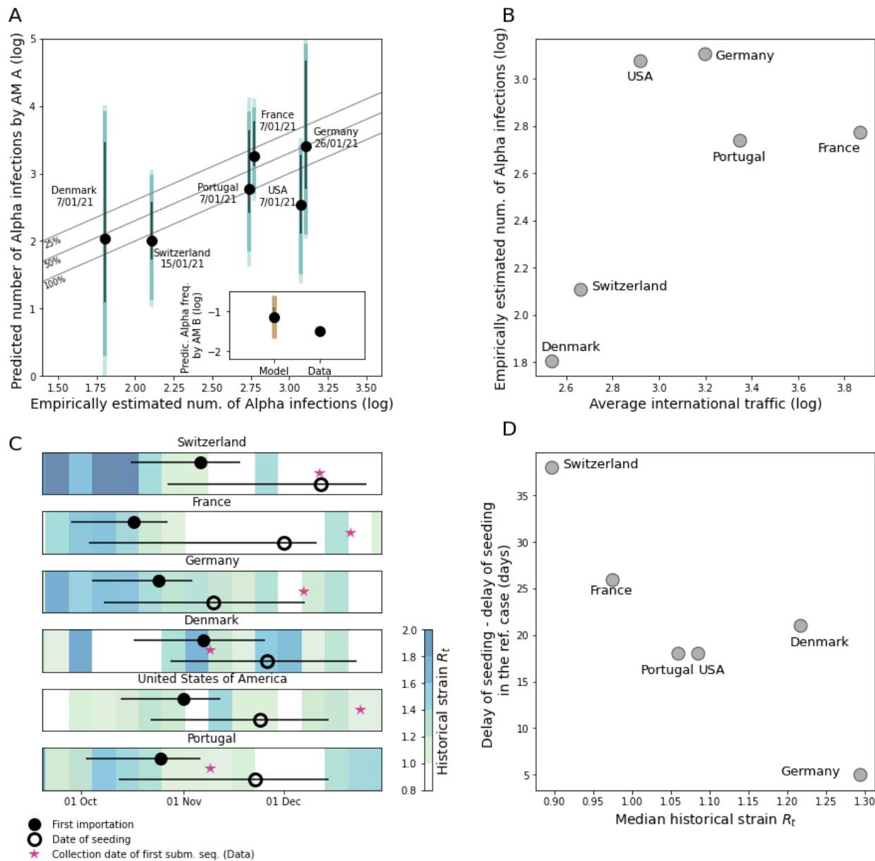
Fig. 4. Local spread of Alpha in six destination countries. (A) Model vs. empirical spread of Alpha for six destination countries outside the UK. For each country we report the date when the percentage of Alpha was determined. In the main plot, the empirical estimates of Alpha cases are computed by multiplying the Alpha frequency resulting from virological investigations by the COVID-19 incidence reported in the country at the same date. Model estimates are obtained with the autochthonous model A (AM A in the plot) as described in the Material and Methods. Gray lines show ratios of 100%, 50% and 25% between observed and predicted that can be attributed to reporting. In the inset, the frequency of Alpha in France obtained from the autochthonous model B (AM B in the plot) is compared with the empirical data. In both panels, black error bars indicate the prediction interval over 500 stochastic simulations obtained with the median volume of Alpha introduction as predicted by the international dissemination model, assuming a 7-day delay between case and infection. Dark colored bars account for the variability in the output of the
