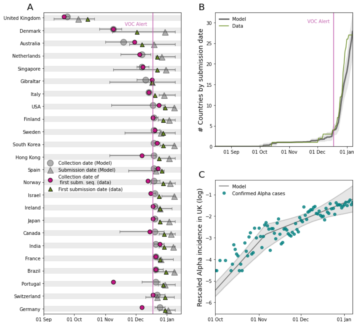
Fig. 2. Comparison between the international dissemination model and the data. (A) Date of collection of the first Alpha sample submitted to GISAID and corresponding date of submission for the 24 countries submitting Alpha sequences before 31 Dec 2020. Data are shown by purple circles (collection) and green triangles (submission). Model output is indicated by gray circles (collection) and gray triangles (submission). The horizontal bars display the 95% prediction interval. (B) Model predicted cumulative number of countries submitting a first Alpha sequence to GISAID compared with observations. In panels A and B, the purple vertical line indicates the date of Alpha international alert (18 Dec 2020). (C) Alpha incidence in the UK 39 and model-predicted epidemic profile in the UK. Both model predictions and data are rescaled to the sum over the period considered to allow comparing the profiles of the curves. To account for testing delays model predictions are shifted right of one week. The gray coloured ribbon represents the 95% credible interval.
