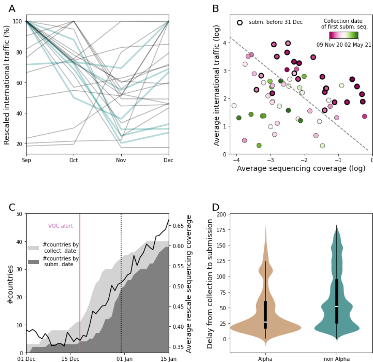
Fig. 1. Factors associated with the pattern of observed Alpha dissemination. (A) Change in outbound international traffic from the UK over time. The 73 countries contributing to GISAID during 1 Sep 2020 - 31 Dec 2020 are shown as an example. Traffic is rescaled to the maximum value over the period. International traffic includes air-travel and estimated passengers via train, ferry and Channel Tunnel (32). Countries displayed in blue are the six countries analyzed in detail in the last subsection of the Results section. (B) Date of first detection, i.e. collection of the first Alpha sequence submitted to GISAID, for each of the 73 countries contributing to GISAID before 31 Dec 2020 according to the sequencing coverage and the international traffic (passengers/day) averaged over the same period. For each day, the sequencing coverage of a country is defined as collected SARS-CoV-2 sequences on GISAID - regardless of the date of submission - divided by reported cases. The dashed line indicates y = x . (C) Cumulative number of countries with at least one Alpha submission plotted by the date of collection and date of
