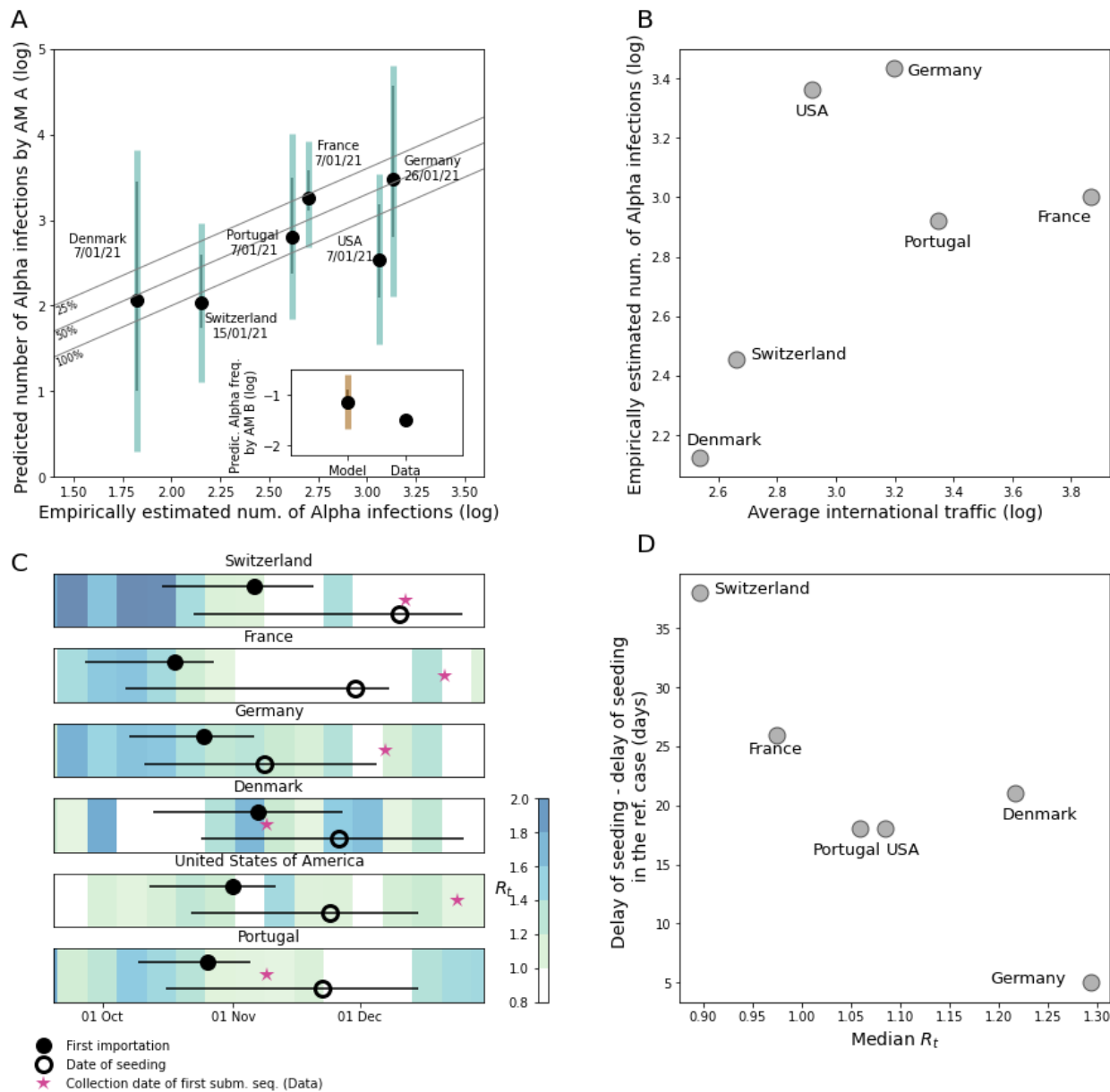
Fig. 4. Local spread of Alpha in six destination countries. (A) Model vs. empirical spread of Alpha for six destination countries outside the UK. In the main plot, the empirical estimates of Alpha cases are computed by multiplying the Alpha frequency resulting from virological investigations by the COVID-19 incidence reported in the country at the same date. Model estimates are obtained with the autochthonous model A (AM A in the plot) as described in the Material and Methods. Grey lines show ratios of case detection of 100%, 50% and 25% between observed and predicted. In the inset, the frequency of Alpha in France obtained from the autochthonous model B (AM B in the plot) is compared with the empirical data. In both panels, black error bars indicate the prediction interval over 500 stochastic simulations obtained with the median volume of Alpha introduction as predicted by the international dissemination model. Colored bars account for the variability in the output of the autochthonous models accounting for the upper and the lower limit of the prediction interval of the Alpha introductions as given by the international
