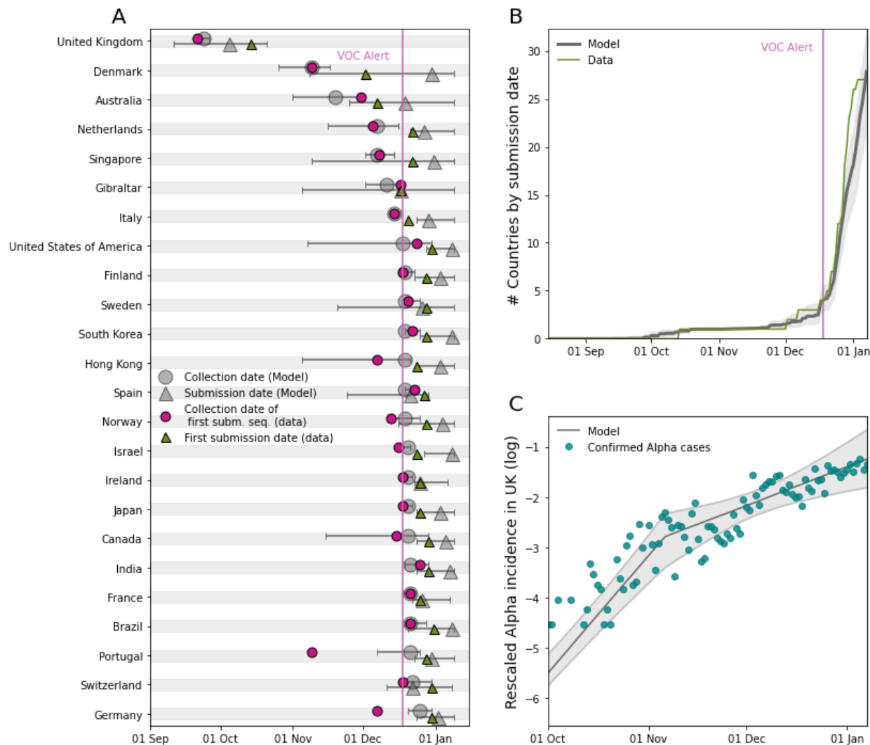
Fig. 2. Comparison between the international dissemination model and the data. (A) Date of collection of the first Alpha sample submitted to GISAID and corresponding date of submission for the 24 countries submitting Alpha sequences before 31 Dec 2020. Data are shown by purple circles (collection) and green triangles (submission). Model output is indicated by gray circles (collection) and gray triangles (submission). The horizontal bars display the 95% prediction interval. (B) Model predicted cumulative number of countries submitting a first Alpha sequence to GISAID compared with observations. In panels A and B, the purple vertical line indicates the date of Alpha international alert (18 Dec 2020). (C) Alpha incidence in the UK (36) and model-predicted epidemic profile in the UK. Both model predictions and data are rescaled to the sum over the period considered to allow comparing the profiles of the curves. To account for testing delays model predictions are shifted right of one week.
