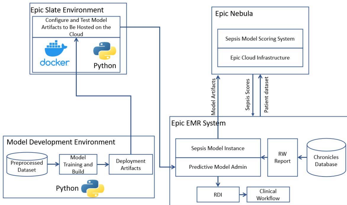
Figure 2. Model deployment and operationalization.
