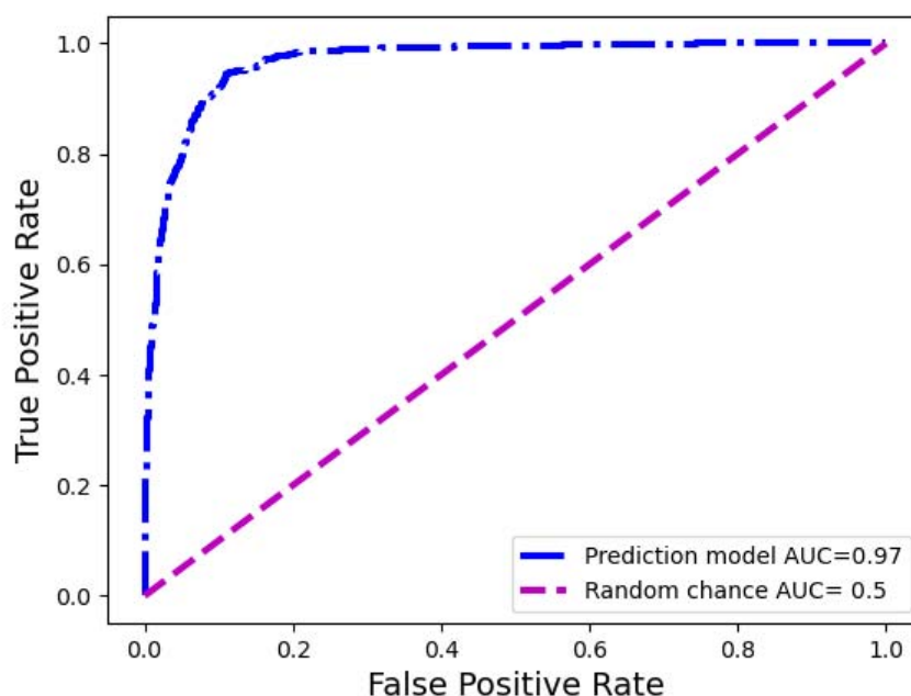
Figure 4. Receiver operating curve of the sepsis prediction model: Pre-deployment performance
