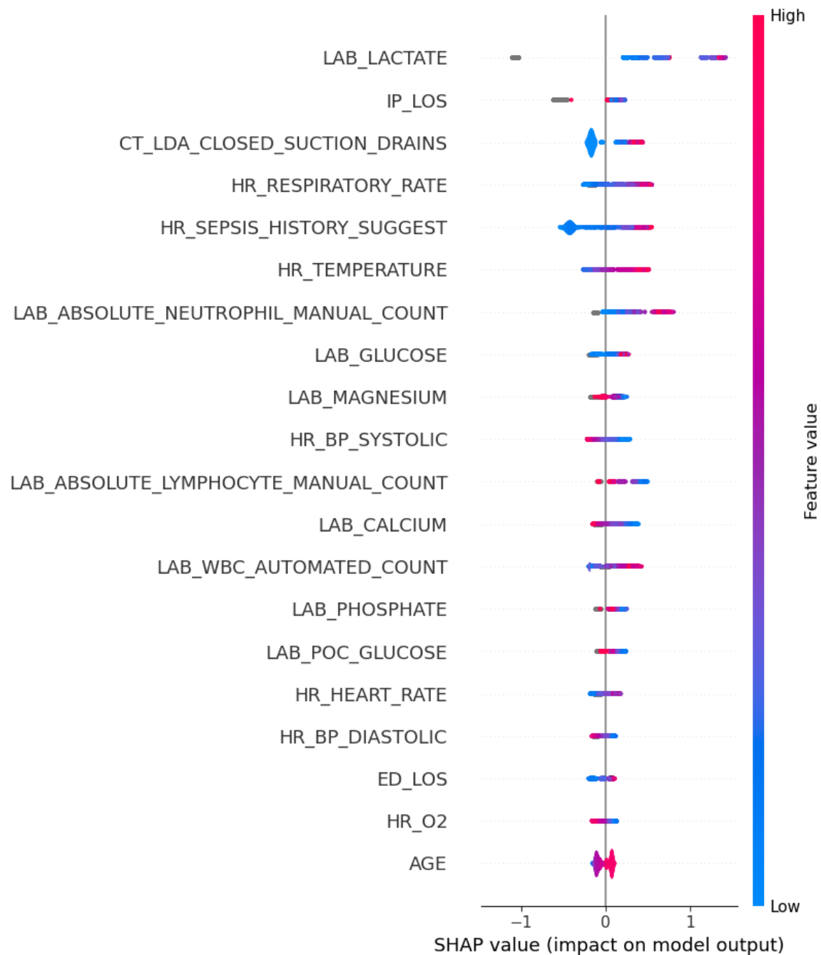
Figure 5. Highly important features and their corresponding Shapley values. The grey color depicts the missing values (NaN) in a certain feature.
