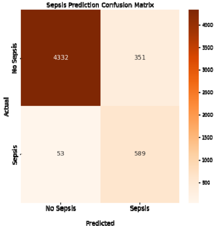
Figure 3. Confusion matrix of the sepsis prediction model. Sensitivity is 92% and specificity is 93% with a 7% false positive rate. Colorbar represents the count of cases.
