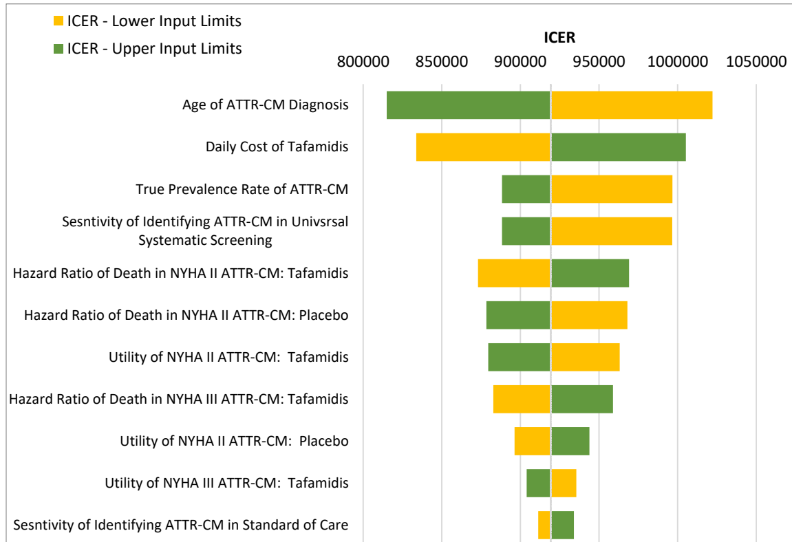
Figure 2: Tornado diagram of 1-way Sensitivity Analysis
