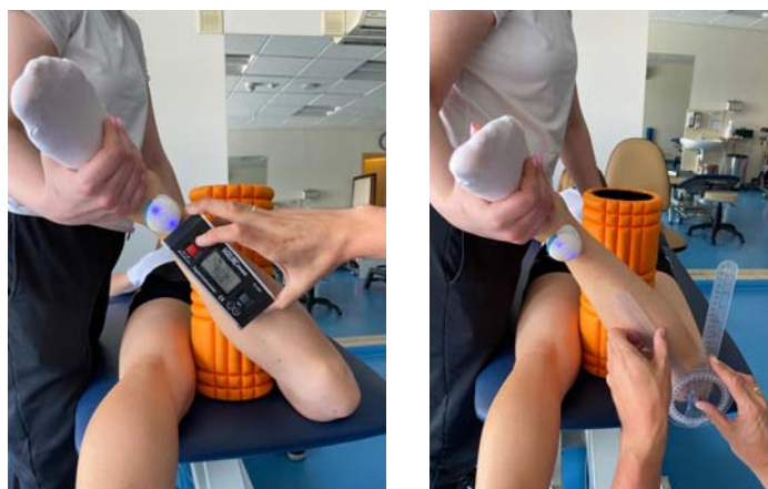
Figure 2. Active internal rotation range of motion assessment with IMU and inclinometer(a) and goniometer(b).
