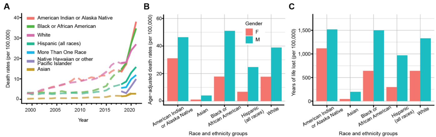
Figure 3: Burden of opioid overdose deaths by race and ethnicity in the United States. A) Opioid overdose death rates from 1999-2021, by race and ethnicity group. Dashed lines are death rates from 1999-2020 with the bridged-race categories, and solid lines are death rates from 2018-2021, with the new single race categories. The rates for Native Hawaiian and Other Pacific Islander and for More Than One Race were only reported separately in the new single race categories, starting in 2018. B) Age-adjusted death rates and C) years of life lost per capita, by race/ethnicity groups and by gender in 2021.
