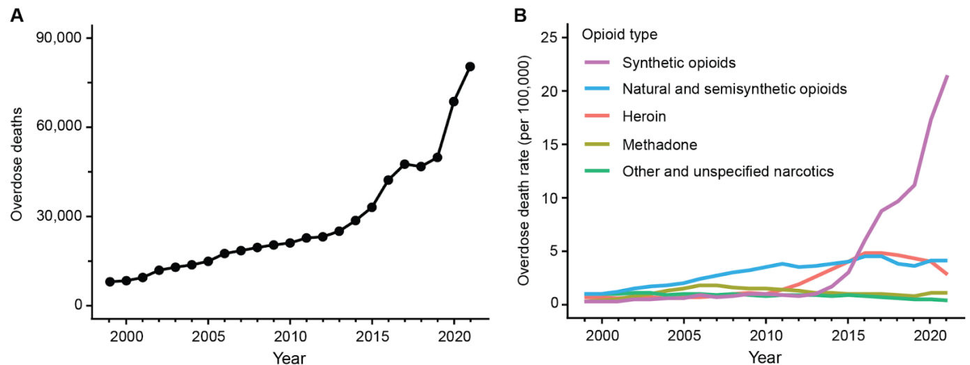
Figure 1: Trends in opioid overdose deaths in the United States from 1999 to 2021. A) Total number of overdose deaths each year involving an opioid. B) Annual rates (per 100,000 population) of overdose deaths, by type of opioid involved. Note that some deaths involve more than one type of opioid. Synthetic Opioids include, for example, drugs such fentanyl (and its derivatives) and tramadol, but excludes methadone. Natural and Semisynthetic Opioids include, for example, oxycodone, hydrocodone, and morphine. Heroin is categorized separately although it is also a semisynthetic opioid. Methadone, a synthetic opioid prescribed to treat opioid use disorder, is categorized separately. Other and Unspecified Narcotics include deaths due to opioid or cocaine-like substances, or mixtures thereof, that were not further sub-categorized on the death certificate.
