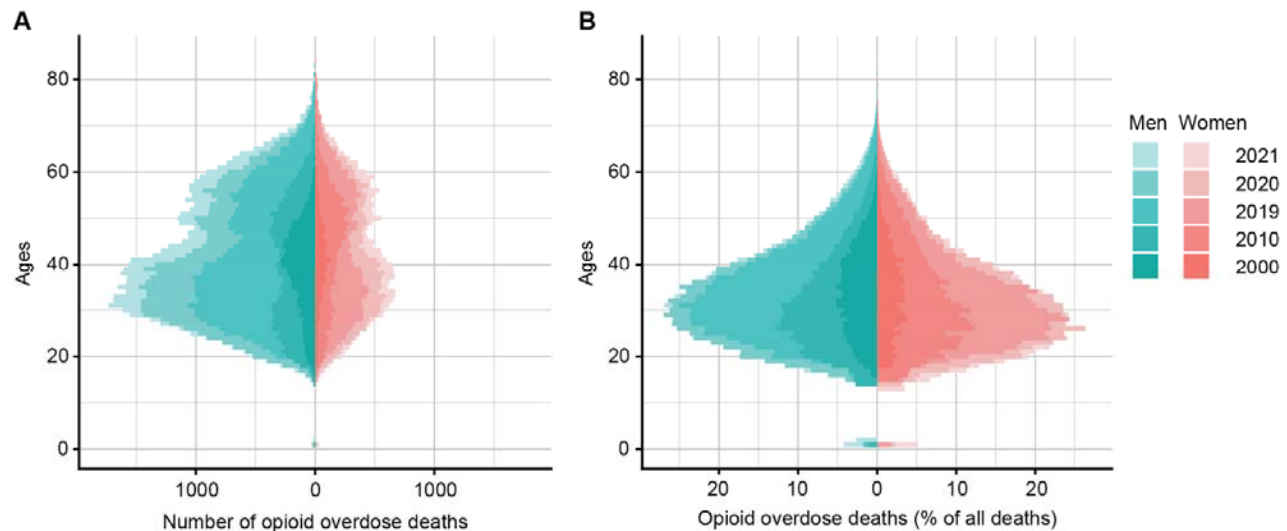
Figure 2: Age distributions of opioid overdose deaths in the United States. Age distribution of opioid overdose deaths by gender, in total numbers A) and as percentage of all deaths B). Distributions for the years 2000, 2010, 2019, 2020 and 2021 are shown in subsequently lighter colors. Note the similarity of the 2021, 2020 and 2019 distributions of % deaths in (B). In 2021 and 2020, despite the increase in the number of opioid overdose deaths, they represented a similar percentage of total deaths in the US due to additional COVID-19 deaths 53 .
