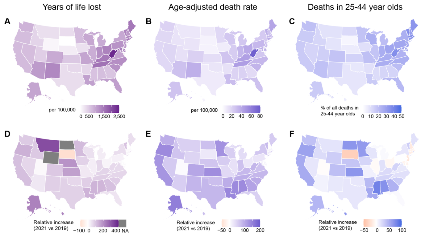
Figure 4: Geographic variation in the opioid epidemic in 2021 (top row) and relative change from 2019 (bottom row). A) and D) Years of life lost per capita due to opioid overdose deaths, by state, B) and E) Age-adjusted opioid overdose death rates by state, C) and F) Percentage of all deaths in 25-44 year olds that are opioid-related, by state. Gray indicates states for which years of life lost estimates were not possible in 2019, due to suppression of counts <10 (see Methods).
