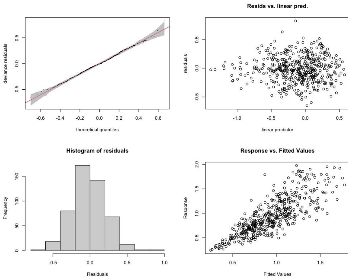
Appendix figure S10: Model diagnostic plots for Model Omicron-Booster-RCHR. The correlation coefficient between fitted RCHR and predicted RCHR is 0.83.
