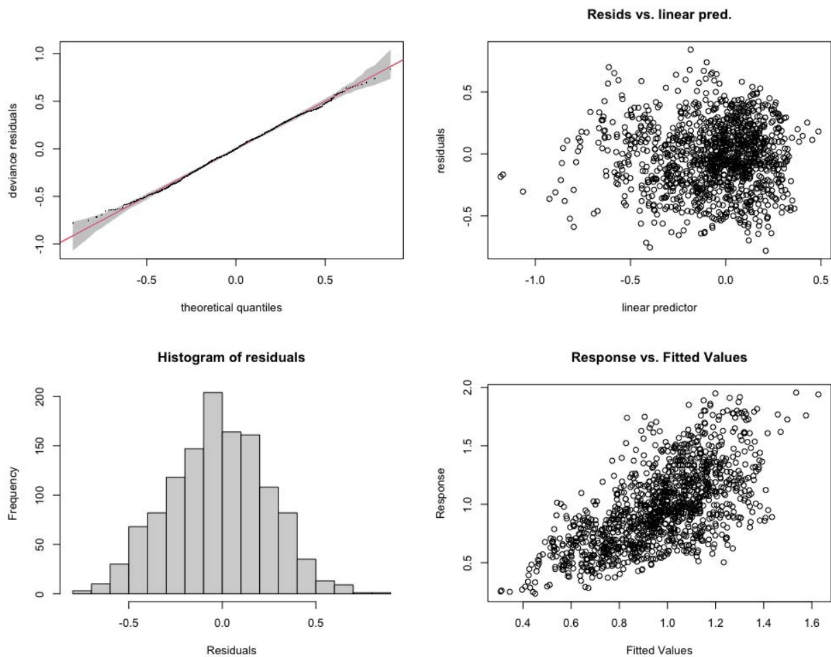
1048 1049 Appendix figure S8: Model diagnostic plots for Model Delta-RCHR. The correlation coefficient between fitted 1050 RCHR and predicted RCHR is 0.67. 1051
