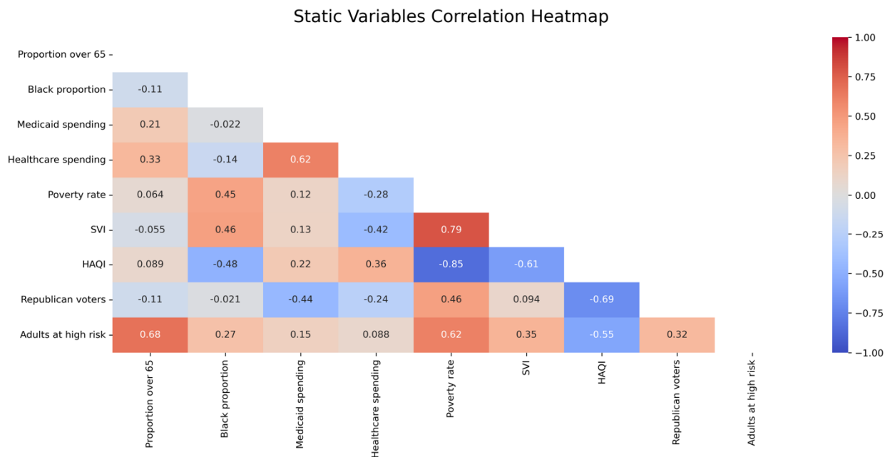
923 Appendix figure S3. Pearson’s correlation heatmap between each pair of static variables. 924
