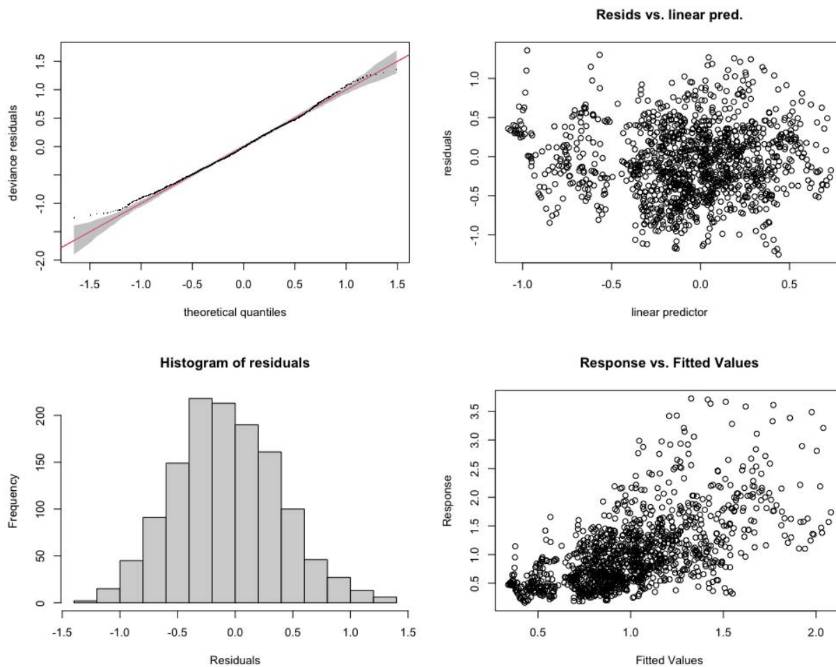
1142 1143 Appendix figure S12: Model diagnostic plots for Model Delta-RCIR. The correlation coefficient between fitted 1144 RCHR and predicted RCHR is 0.61. 1145
