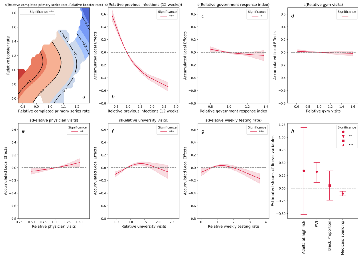
297 298 Figure 2: Results of Omicron-Booster-RCHR for just the Omicron wave with the additional 299 inclusion of an interaction effect between the relative completed primary series rate and the 300 relative booster rate. a: Two-dimensional contour plot for the interaction between relative 301 completed primary series rate and relative booster rate. The deeper red indicates a more positive 302 effect on the RCHR, and the deeper blue indicates a more negative effect to the RCHR. b-g: 303 Accumulated local effects (ALE) of dynamic variables. Shaded areas in each plot indicate 95% 304 confidence intervals. h: Estimated slopes for each static variables, the upper and lower band 305 indicate 95% confidence intervals. ‘***’: variable significant at p < 0.001 . ‘**’: variable 306 significant at p < 0.01 . ‘*’: variable significant at p < 0.05 . ‘’: variable significant at p > 0.05 .
