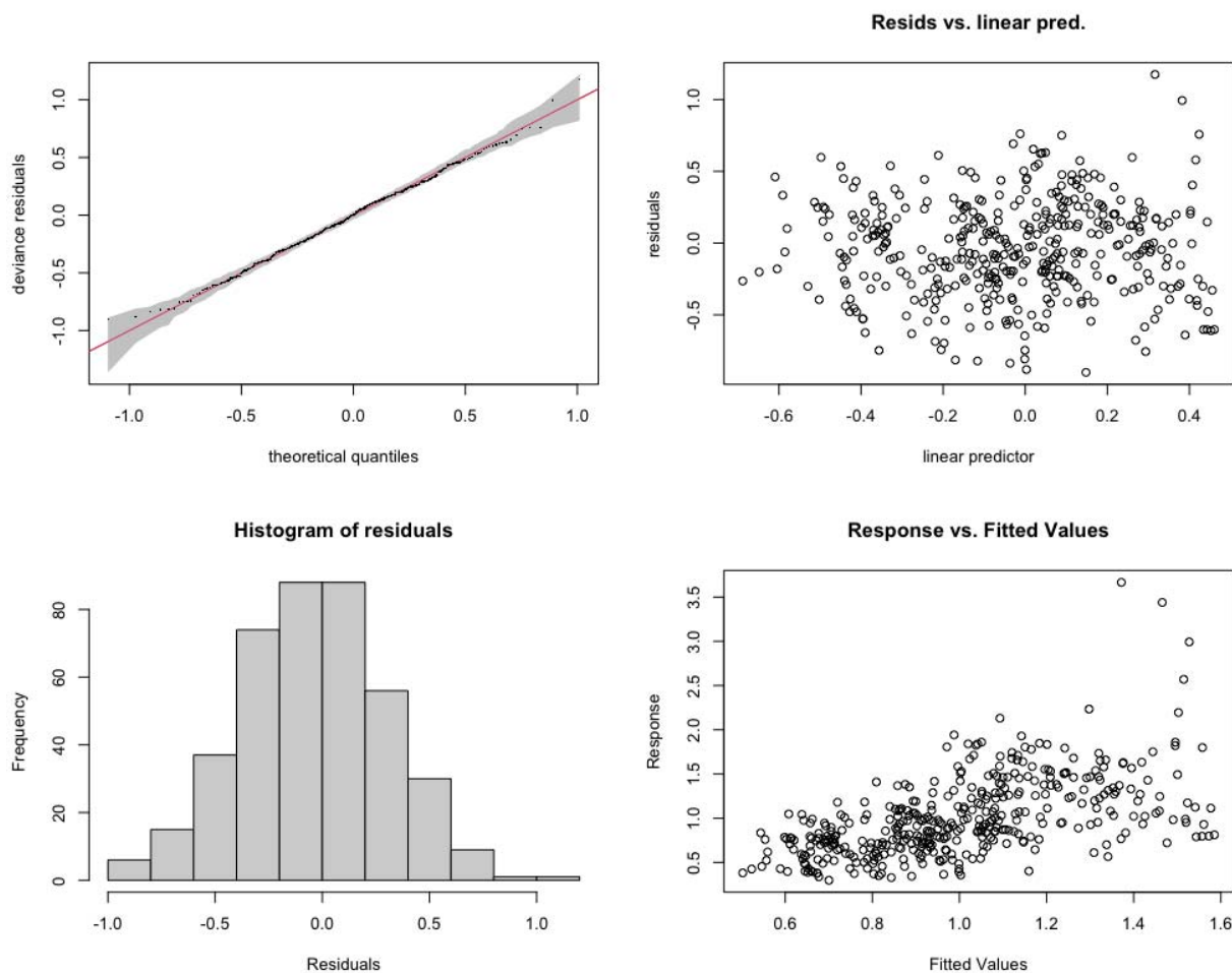
1119 Appendix figure S11: Model diagnostic plots for Model Pre-Delta-RCIR. The correlation coefficient between fitted 1120 RCHR and predicted RCHR is 0.57. 1121
