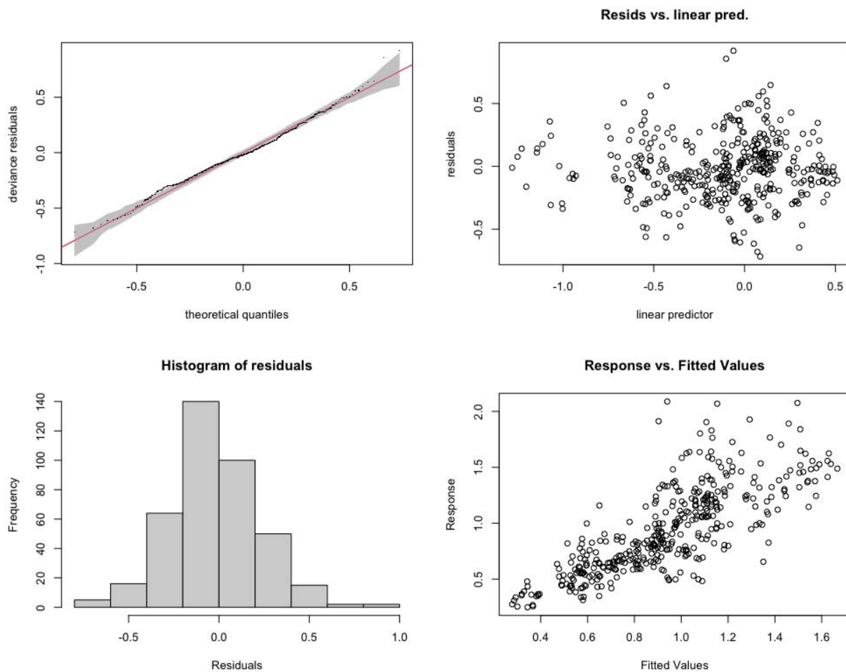
1044 1045 Appendix figure S7: Model diagnostic plots for Model Pre-Delta-RCHR. The correlation coefficient between fitted 1046 RCHR and predicted RCHR is 0.78. 1047
