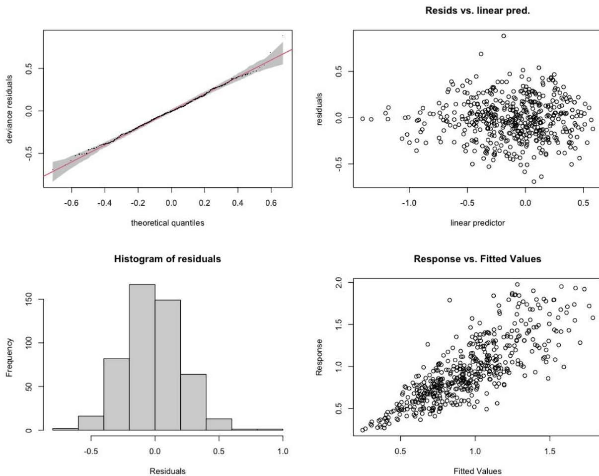
Appendix figure S9: Model diagnostic plots for Model Omicron-RCHR. The correlation coefficient between fitted RCHR and predicted RCHR is 0.81.
