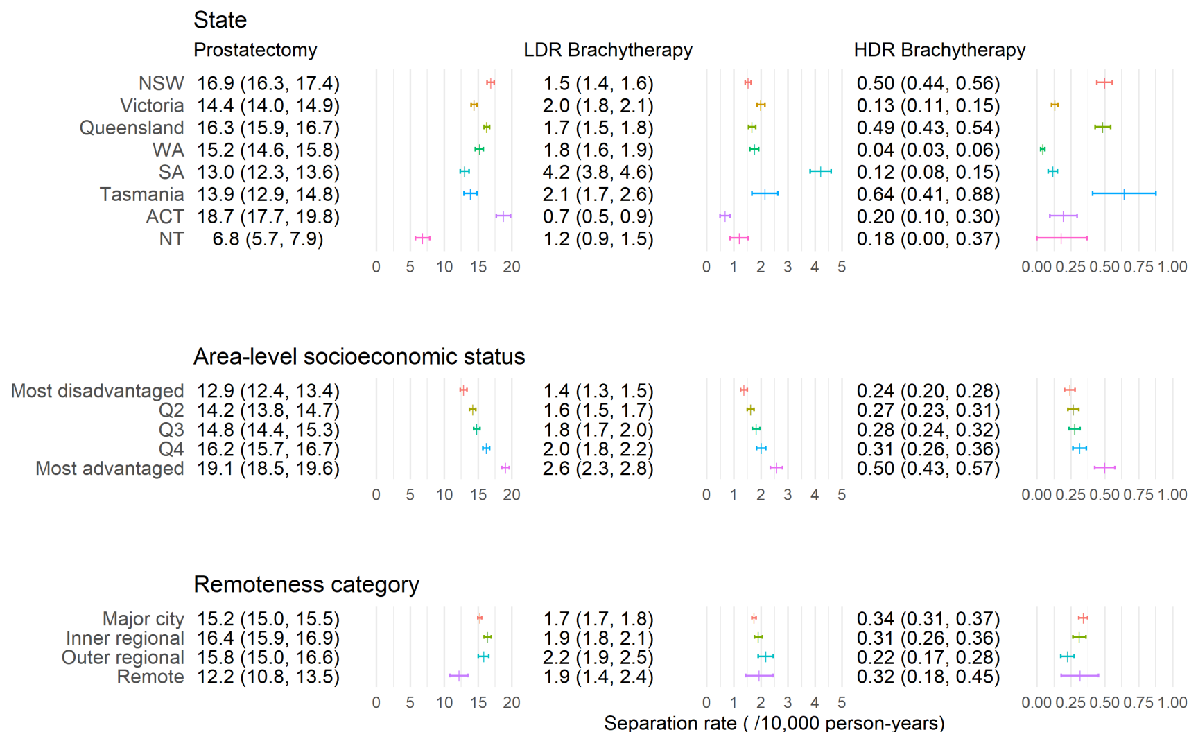
Figure 1; Age-adjusted marginal separation rates (and 95% confidence intervals) for men aged 40 and over by State or Territory, area-level socioeconomic quintile and remoteness category for each treatment. "Prostatectomy" refers to radical prostatectomy. Abbreviations: high dose rate (HDR), low dose rate (LDR), New South Wales (NSW), Western Australia (WA), South Australia (SA), Australian Capital Territory (ACT) and Northern Territory (NT). Note that the horizontal axis scale varies by treatment type.
