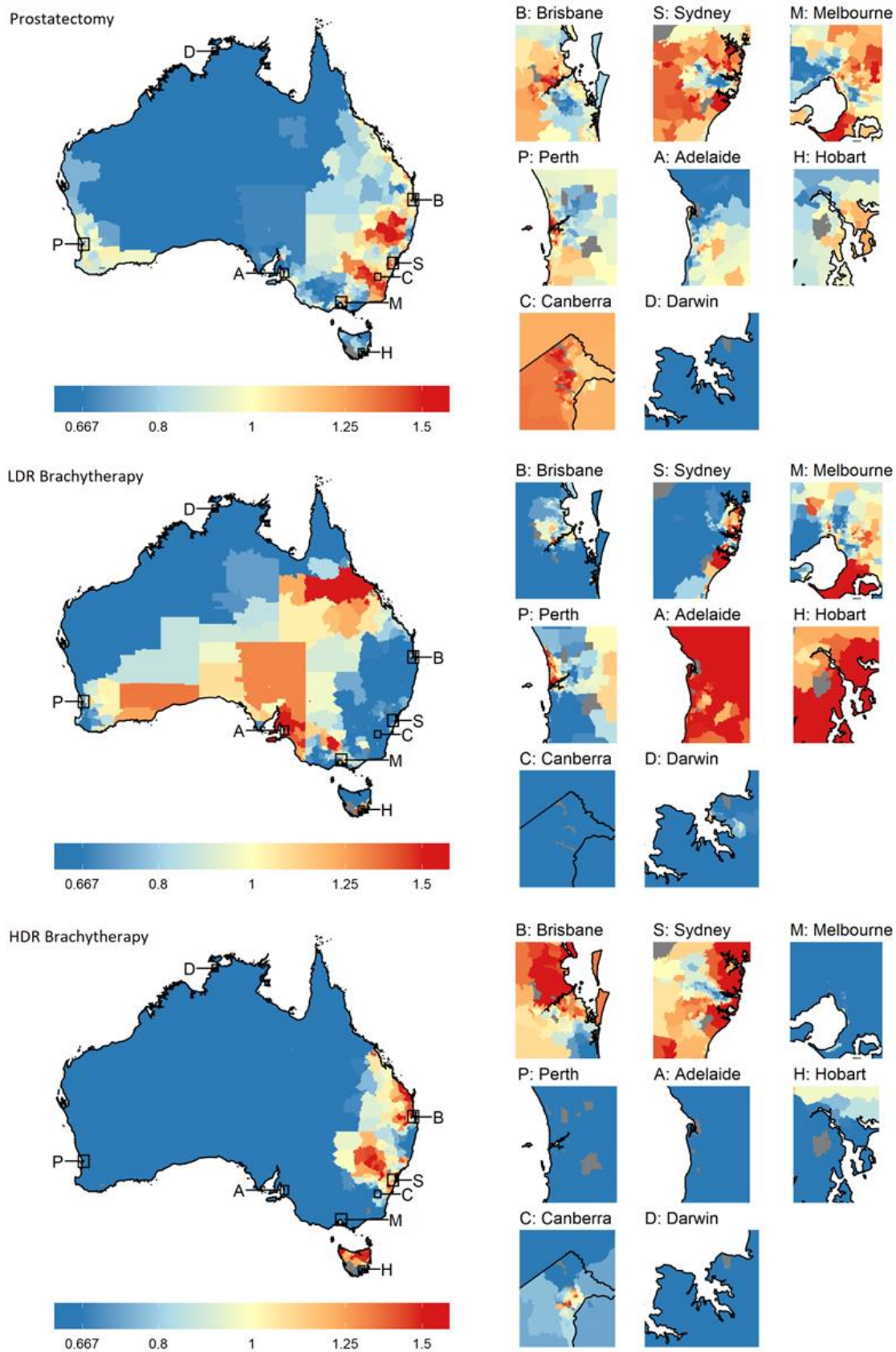
Figure 2; Maps of the standardised separation ratios (SSRs) across Australia for radical prostatectomy (top), low dose rate (LDR) brachytherapy (middle) and high dose rate (HDR) brachytherapy (bottom). Insets show the capital city regions for each State and Territory, which are identified on the main map using their initial. Note that the insets are not of equal dimension.
