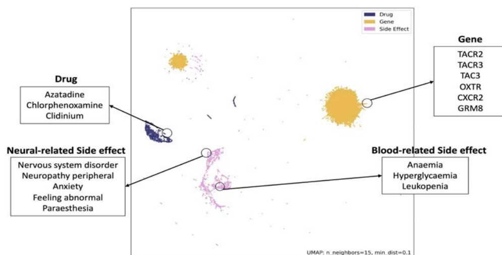
Fig. 3: Node embedding via UMAP visualization. Each point shows the position of a node's 2-dimensional UMAP embedding derived from HHAN-DSI outputs. Different colors show the node type. We annotated some nodes that have high Jaccard Index values, which means that they are similar to each other.
