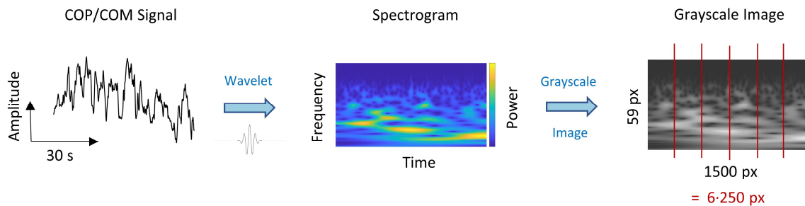
Fig. 3 Data preprocessing. The time-course signals of the COP and COM trajectories underwent wavelet decomposition, resulting in spectrogram images with frequency power as a function of time and frequency. These spectrograms were then treated as grayscale images. Subsequently, each image was cut into six sections. The final samples constituted grayscale images with a size of 59x250 px.
