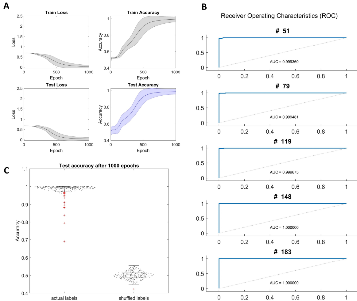
Fig. 1: Network performance on medio-lateral COM data. Panel A: Network performance indicated by total loss and classification accuracy evaluated on the train and test sets over 1000 epochs of training. Solid lines represent the average across 250 models with different subjects assigned to the train and test sets in each case. Shaded areas indicate standard error. Panel B: ROC curves of the 5 best-performing models evaluated after 1000 epochs. Panel C: Test accuracy after 1000 epochs of training. Results from 250 models trained with correctly labeled data versus shuffled labels. Each model trained with different subjects in the train and test set. Grey dots indicate single samples. Red crosses indicate outliers.
