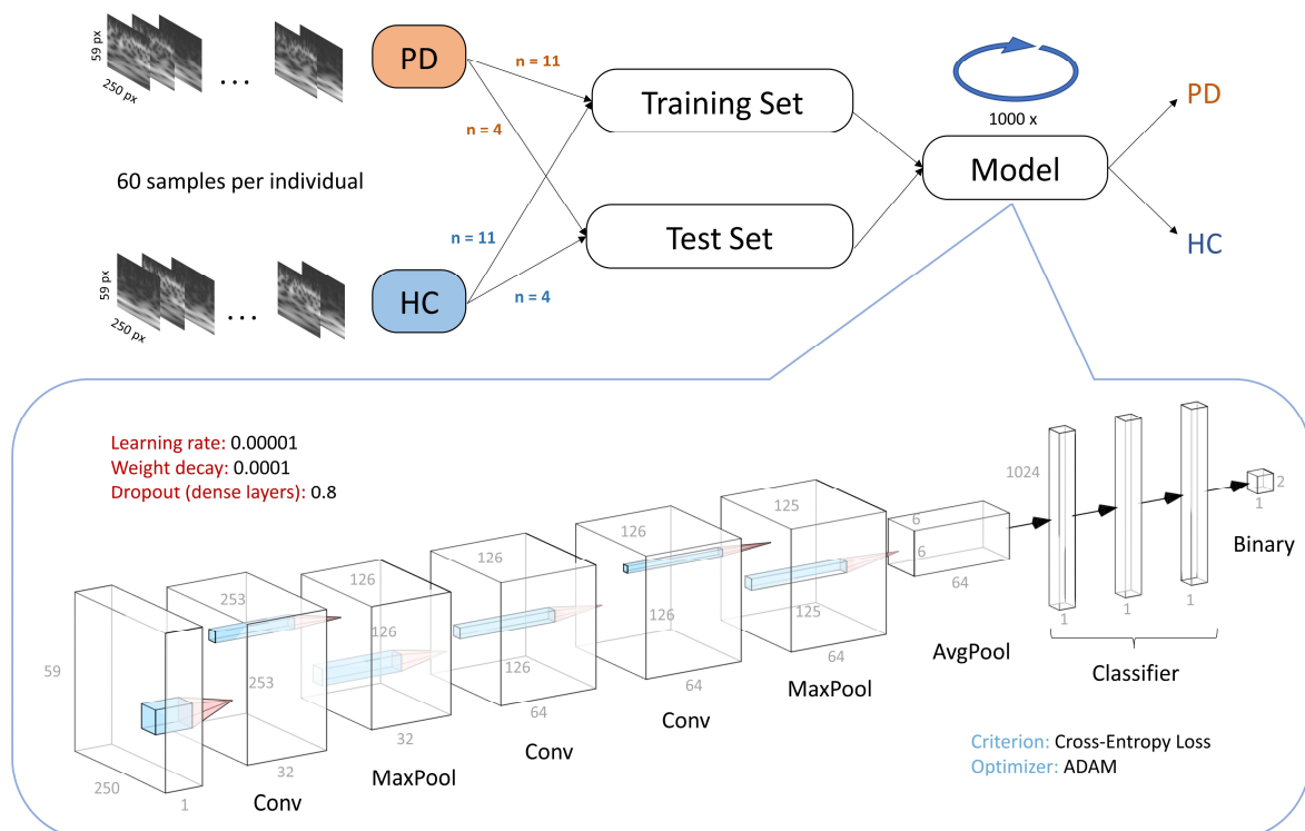
Fig. 4 Data pipeline and architecture. Data was split into train and test sets on a randomized per-subject basis. For each model that we trained, data from 11 participants out of each group, consisting of the corresponding 60 sample images per participant, went into the training set. The remaining data went into the test set. The model was then trained and evaluated for 1000 epochs. We built a CNN with three convolutional and three pooling layers, feeding into a classifier network consisting of three fully-connected layers.
