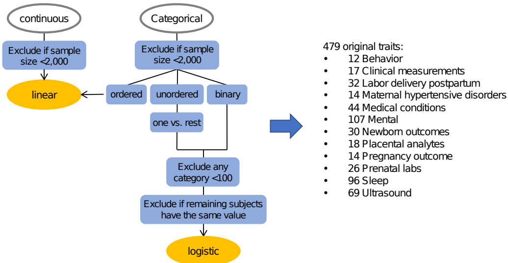
Figure 1. Preprocessing of GWAS traits. The continuous or ordered categorical traits were analyzed using linear regression models. The unordered categorical traits were recoded into several binary traits following the one vs. rest manner, and the binary traits were analyzed using logistic regression models.
