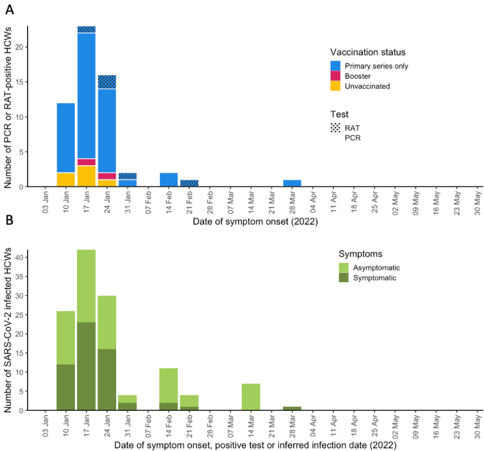
423 424 425 426 Figure 1. SARS-CoV-2 infections among HCWs by week, January 1 – May 31, 2022
