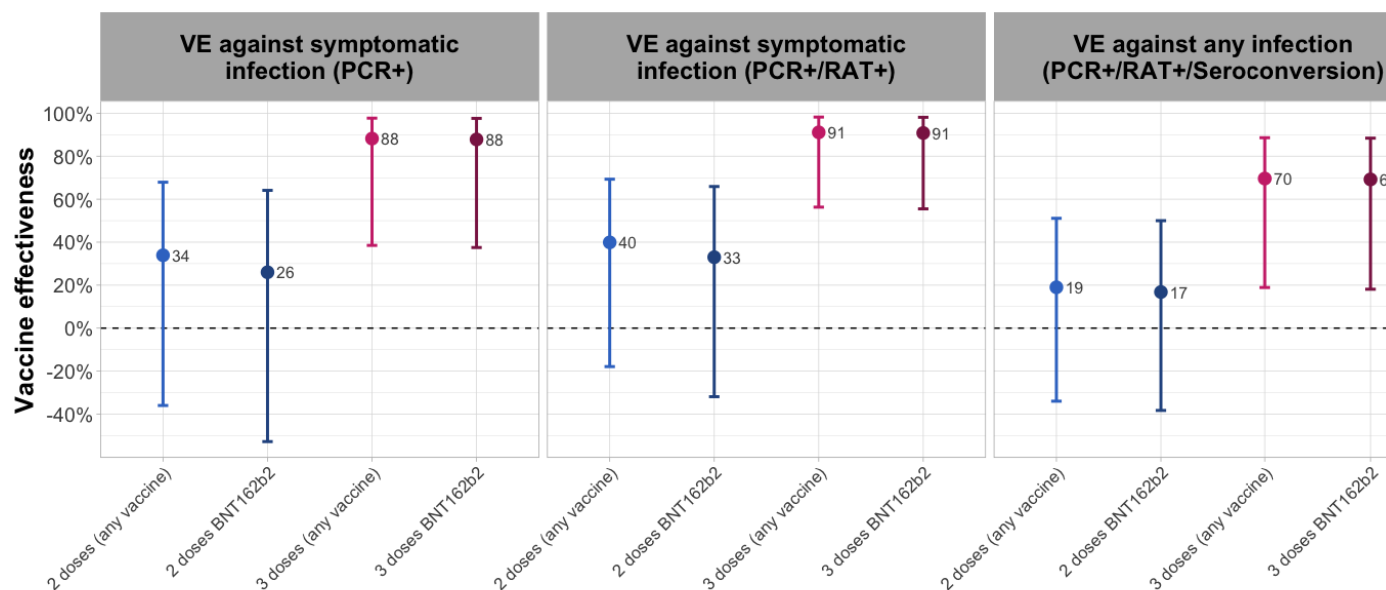
434 435 Figure 2. COVID-19 vaccine effectiveness estimates of primary vaccine series and booster dose against 436 PCR-confirmed symptomatic SARS-CoV-2 infection (left), PCR- or RAT-confirmed symptomatic SARS- 437 CoV-2 infection (middle) and any (asymptomatic or symptomatic) SARS-CoV-2 infection confirmed by 438 PCR, RAT or seroconversion (right) 439 Dot – point estimate; lines – 95% confidence interval; blue – Primary series VE; violet – booster dose VE
