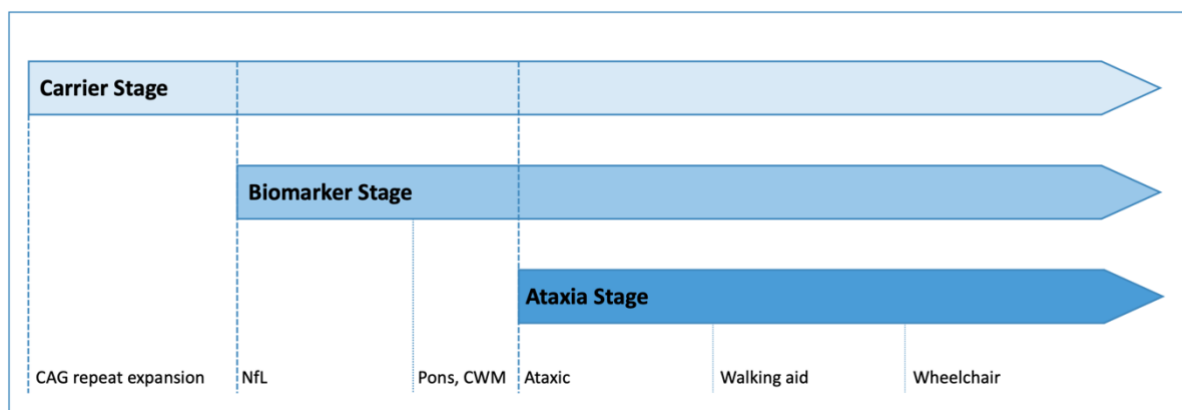
Figure 2: Staging model of SCA3. Proposed staging model of SCA3 based on the studied fluid and MRI biomarker data. The model includes an initial asymptomatic carrier stage followed by the biomarker stage defined by absence of ataxia, but a significant rise of NfL. The biomarker stage leads into the ataxia stage, which is defined by manifest ataxia. Following previous suggestions, the ataxia stage is further subdivided into three substages defined by milestones of gait deterioration. 30
