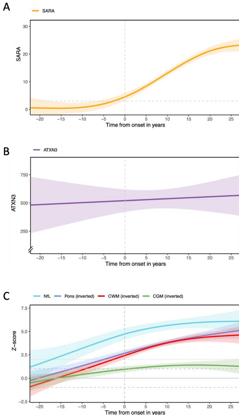
Figure 1: Scale for the Assessment and Rating of Ataxia (SARA) scores, fluid and MRI biomarker data in SCA3 mutation carriers in relation to time of ataxia onset. Data were analyzed with additive Gaussian regression on a time scale defined by ataxia onset. The time of ataxia onset is indicated with a vertical dashed line in all graphs. The estimated 95% CIs are shown by the shaded areas around the curves. (A) SARA sum score. The SARA cut-off of 3
