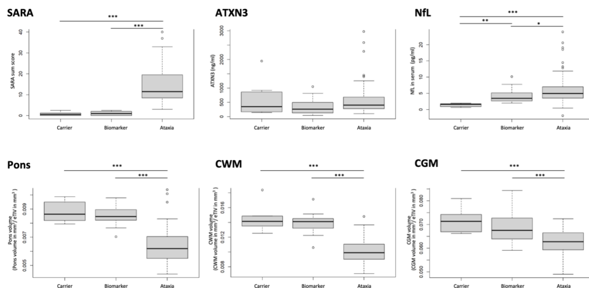
Figure 3 Scale for the Assessment and Rating of Ataxia (SARA) scores, fluid and MRI biomarker data in the carrier, biomarker and ataxia stage of SCA3. Data were analyzed with one-way ANOVA followed by pairwise comparisons using Tukey's test * p<0.01; **p<0.001. NfL - neurofilament light, CWM – cerebellar white matter, CGM – cerebellar grey matter, eTIV – estimated intracranial volume.
