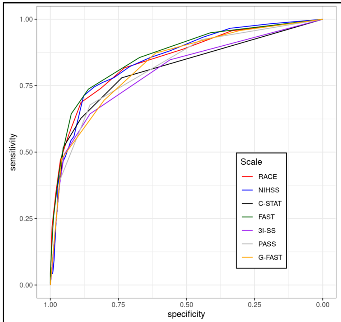
Figure 2. ROC Curves for Prehospital LVO Scales using Posterior Circulation Criteria
