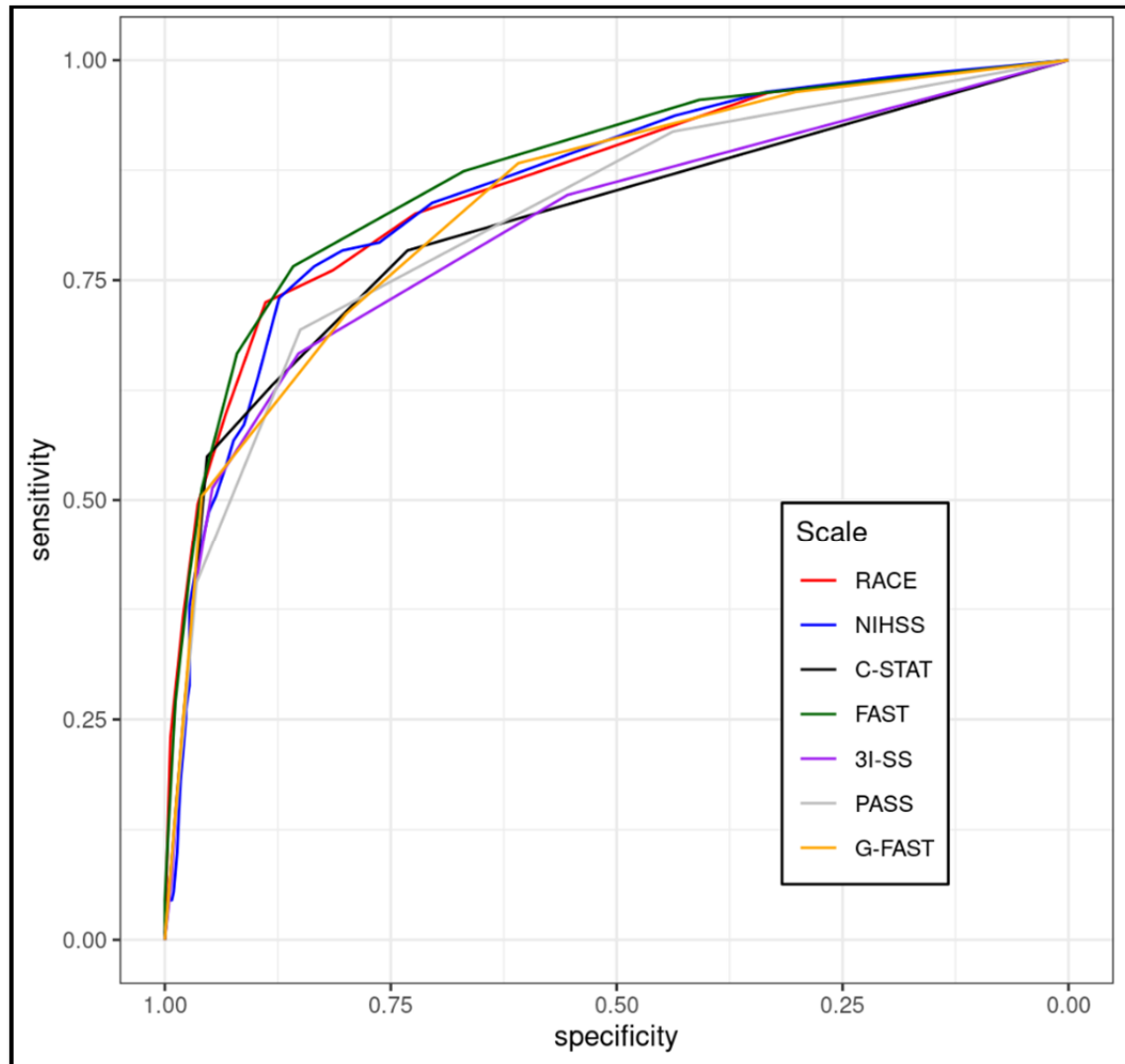
Figure 1. ROC Curves for Prehospital LVO Scales using Anterior Circulation Criteria
