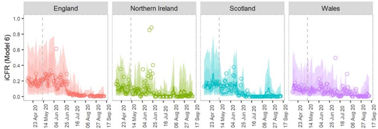
Figure 3. Sensitivity analysis of the best model (Model 6) . The panels show the model's prediction results until mid-September, the time when the first alpha variant has been detected in the UK. The points in each subplot represent the instantaneous CFR (iCFR) estimated using the back-projection method for each date. Solid lines represent the CFR estimated using the best-prediction model. The shaded regions indicate pointwise 75% and 95% prediction intervals, respectively. The vertical dashed lines represent the day until which we train the data in the model, whereas on the right side of the line are tested data.
