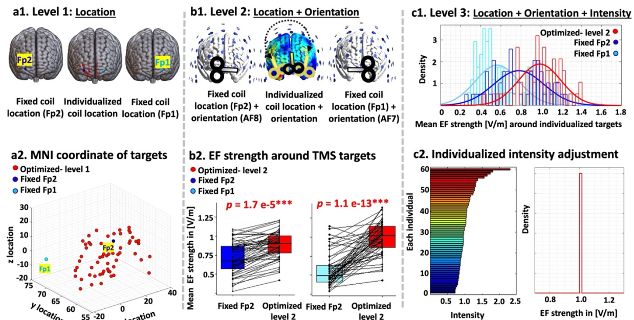
Figure 4. Stimulation parameter optimization. Simulation results were compared between three approaches (1/2) fixed Fp2: coil placed over Fp2/Fp1 in EEG standard system with a fixed orientation toward AF8/AF7 and constant stimulation intensity across the population, and (3) optimized: Optimization was performed at three levels: location, orientation, and intensity. coil was placed over the individualized maximal PPI location, coil direction was optimized to maximize EF perpendicular to the individualized targets, and stimulation intensity was adjusted to have identical 1 V/m averaged EF strength across the population in a 5mm sphere around the individualized targets. (a) Level 1: Location (coil location individualization). Brains in MNI space and the scatter plot shows target location in each approach. The blue dot represents the Fp1 (light blue) and Fp2 (dark blue) locations which were targeted in the fixed approaches and the red dots represent the individualized targets in the optimized approach obtained from maximal amygdala-frontopolar PPI connectivity. (b) Level 2: Location + Orientation (coil orientation optimization in individualized targets). In the fixed approaches standard coil directions were used (AF8/AF7) while in the optimized approach optimization algorithm (ADM method) tried to maximize perpendicular EFs in individualized brain targets. Boxplots showing effects of orientation optimization on averaged EF in a 5mm sphere around the individualized target. Dots and spaghetti lines over the boxplots represent the data for each individual participant. P values for differences are reported above boxplots. (c) Level 3: Location + Orientation + Intensity (stimulation intensity adjustment). Distributions of the averaged EF strength in a 5mm sphere around the individualized targets are represented for the fixed (Fp1/Fp2 in light/dark blue) and optimized (in red)
