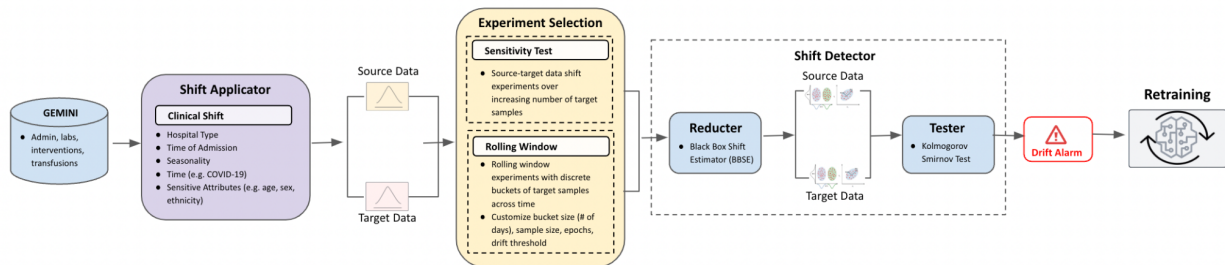
Figure 2. Monitoring and evaluation pipeline. An end-to-end pipeline where EHR data is first sent to the Shift Applicator , which outputs a source and target data based on the clinical shift of choice. The source and target data can then be leveraged by the Shift Detector to conduct a drift sensitivity test or a rolling window analysis—if drift is detected, retraining is triggered.
