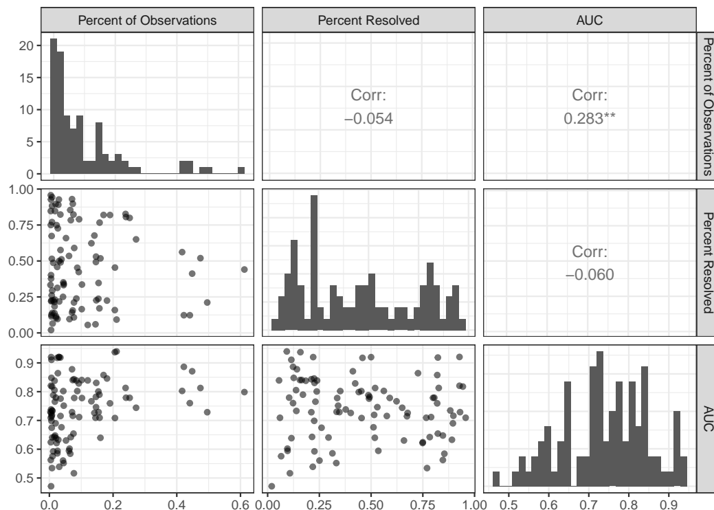
Figure SM2 Resolution likelihood models—Pairwise comparison of test set AUC, percent of observations with a given barrier, and percent resolved for that barrier. The diagonal shows histograms for each of those three measures; the upper diagonal displays correlation coefficients; and the lower diagonal shows scatter plots.
