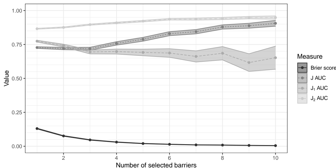
Figure SM3 Brier score and AUC metrics for composite objective as a function of the number of barriers selected (95% CI are shown for each metric). The Brier score shown is for J (not J_1 nor J_2 ).
