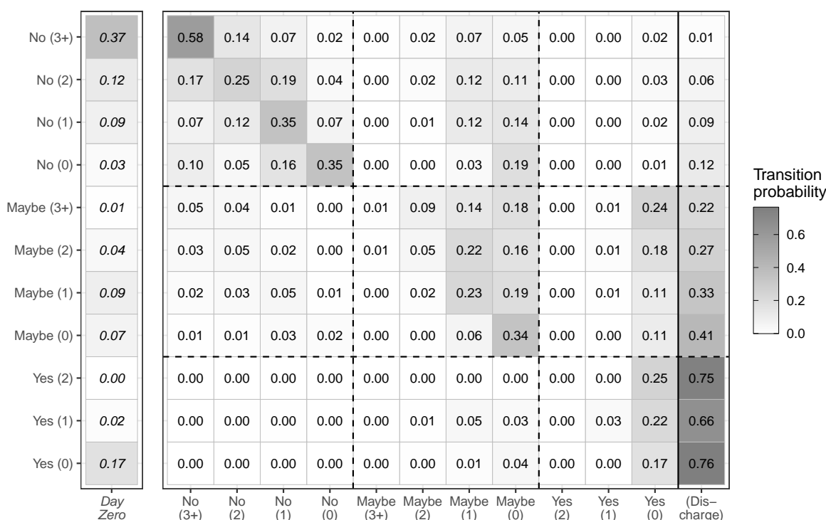
Figure SM5 Transition probabilities from various states determined by frequencies in the test set. Each row corresponds to an initial state, and the columns correspond to the patient’s state on the following day. States are displayed in the format “Yes/Maybe/No group (# prescribed barriers).” Dashed lines are shown for visual reference in order to group states in Yes/Maybe/No groups. “(Discharge)” is treated as an absorbing state. The initial (day zero) state percentages are shown on the left for reference.
