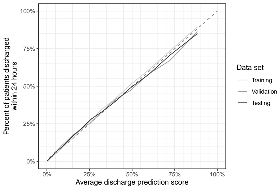
Figure SM1 Calibration curves for the discharge prediction scores on the three data sets. Predictions grouped into 20 equally sized groups for each of the data sets.
