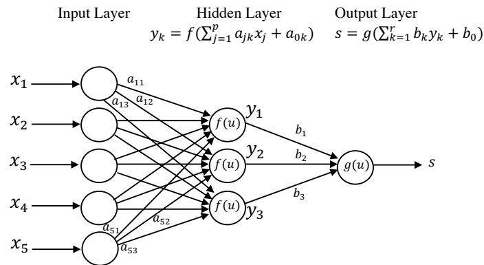
Figure SM4 Network structure and parameters for an example feedforward neural network classifier
