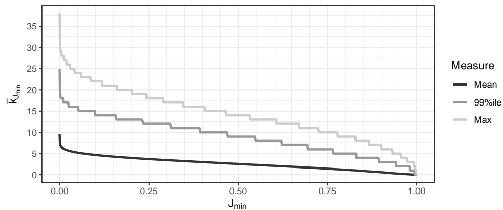
(a) \bar{k}_{J_{\min}} as function of J_{\min} .
