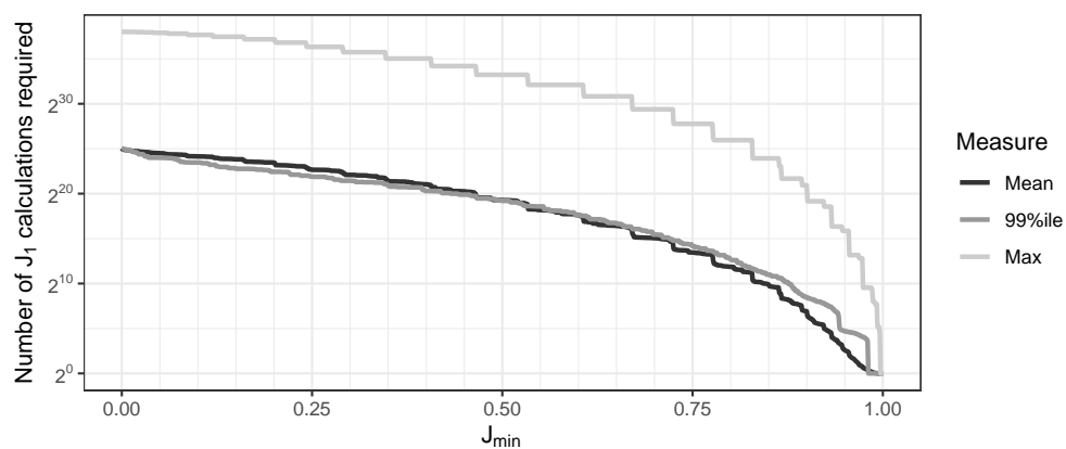
(b) Number of calculations of J_1 required (based on upper bound \bar{k}_{J_{\min}} ); note the logarithmic scale.
