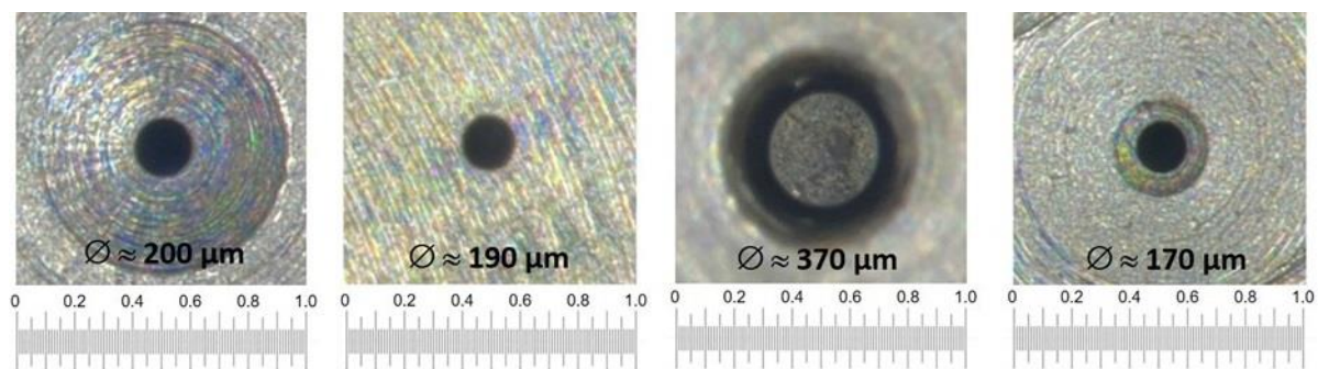
201 202 Figure 2: Light microscopic images of the outlet orifices with determined orifice diameters of the 203 examined nozzles; scaling in mm.
