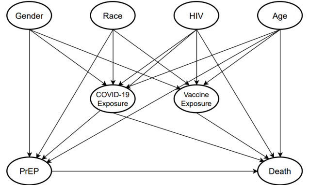
Fig. 1: Proposed causal graph with all observed variables
