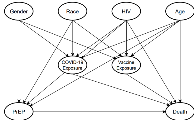
Fig. 1: Proposed causal graph with all observed variables
