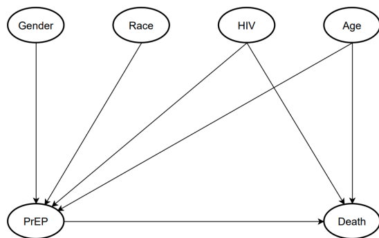
Fig. 2: Proposed causal graph after adjusting for bias
