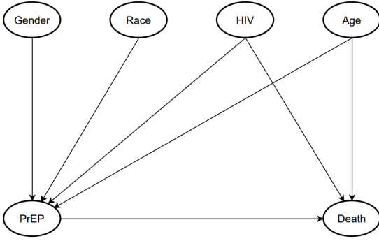
Fig. 2: Proposed causal graph after adjusting for bias
