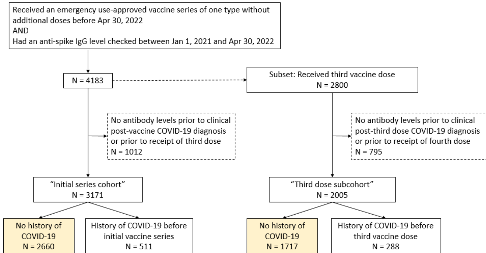
Figure 1. Consort diagram
