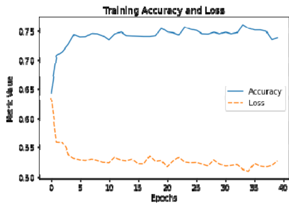
Figure 3. Training accuracy and loss curve
