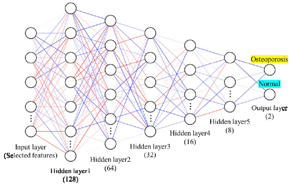
Figure 2. Schematic diagram of multi-layer perceptron neural network
