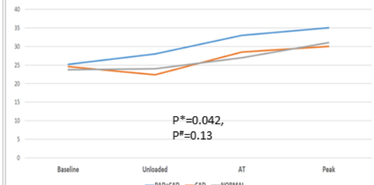
SPAP, mmHg
