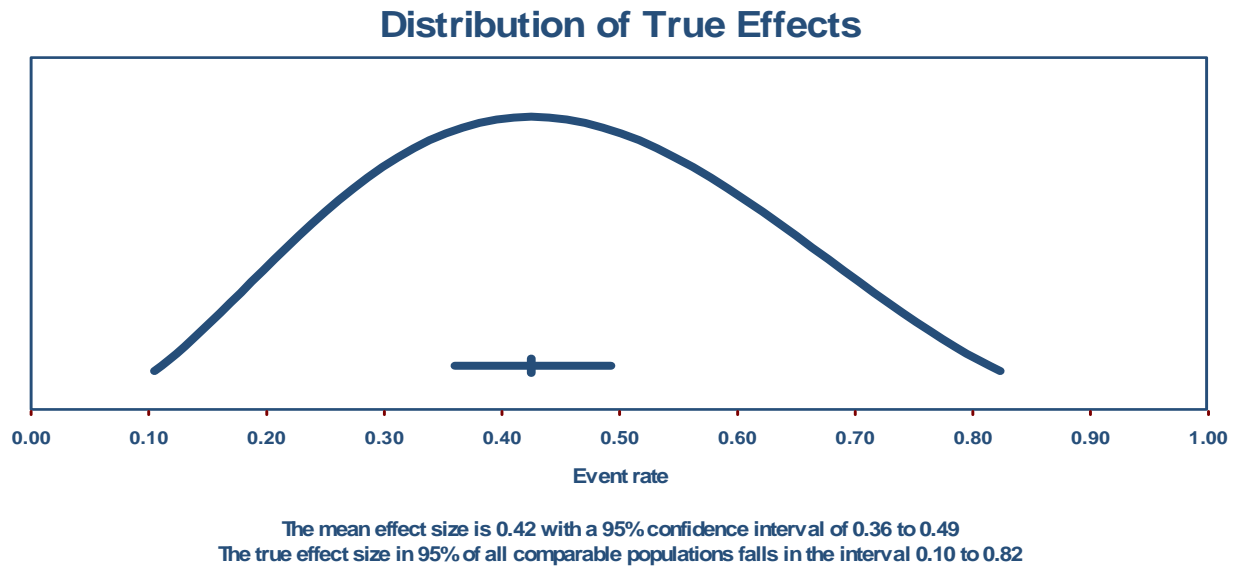
Figure 3: The prediction interval demonstrating the true effects size in 95% of all the comparable populations
