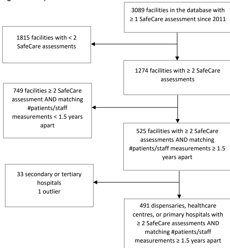
Figure 1. Study flowchart.
