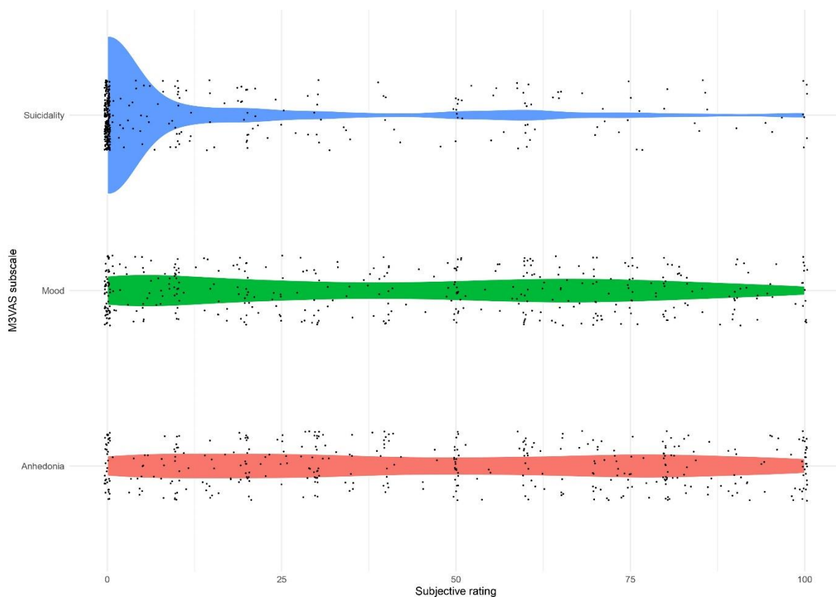
Figure 3: Violin plot of kernel density estimates from the M3VAS. Individual participant scores are represented by dots (the random vertical distribution of the dots is a visual aid only).
