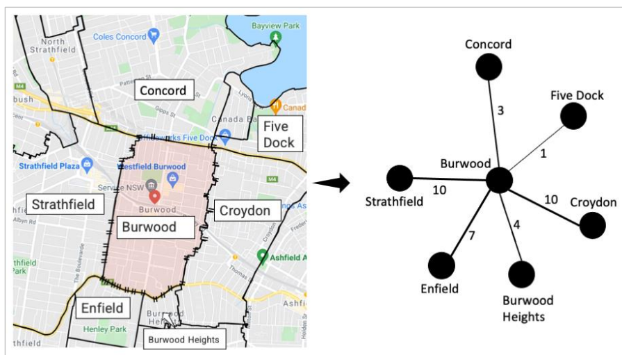
Figure 1: An illustration of the construction of the suburban road network. The left-hand figure shows the map from the Google Maps website. The right-hand figure is the corresponding suburban road network. Burwood (shaded with light red colour) is the suburb under consideration. Edge weights between two suburbs are the number of roads connecting them. For example, the edge weight (right-hand figure) between Burwood and Strathfield is ten since ten roads connect these two suburbs (left-hand figure). Edge thickness in the right-hand figure proportionates to the corresponding edge weight.
